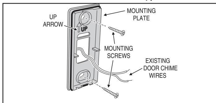
Door Chime/Sensor Mounting
