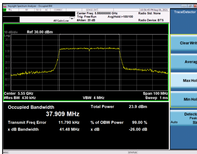
Plot 7-34. 26dB BW & 99% OBW Antenna 5T (40MHz BW 802.11ax(SU) – Ch. 110, MCS3)
