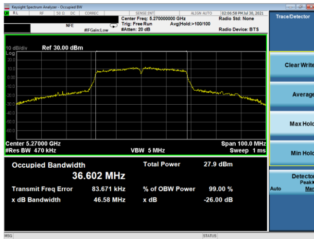
Plot 7-9. 26dB BW & 99% OBW Antenna 5T (40MHz BW 802.11n – Ch. 54, MCS2)
