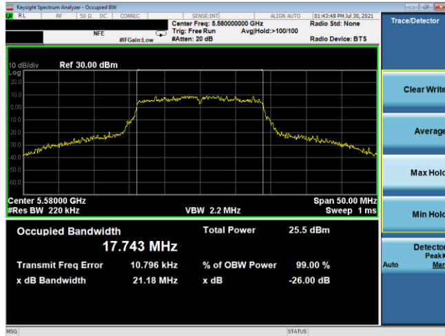
Plot 7-13. 26dB BW & 99% OBW Antenna 5T (20MHz BW 802.11n - Ch. 116, MCS2)
