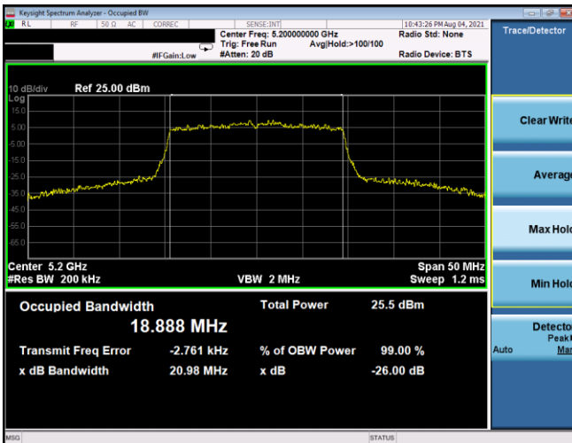
Plot 7-2. 26dB BW & 99% OBW Antenna 5T (20MHz BW 802.11ax(SU) – Ch. 40, MCS2)
