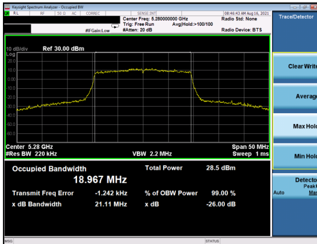
Plot 7-8. 26dB BW & 99% OBW Antenna 5T (20MHz BW 802.11ax(SU) – Ch. 56, MCS2)
