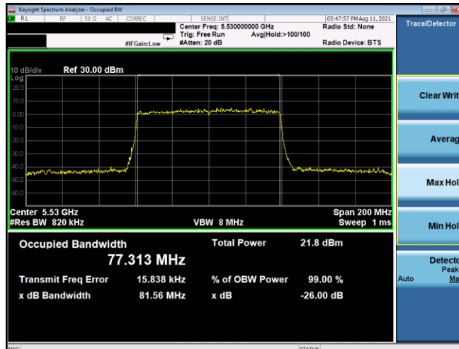
Plot 7-54. 26dB BW & 99% OBW Antenna 5T (80MHz BW 802.11ax(SU) – Ch. 106, MCS5)
