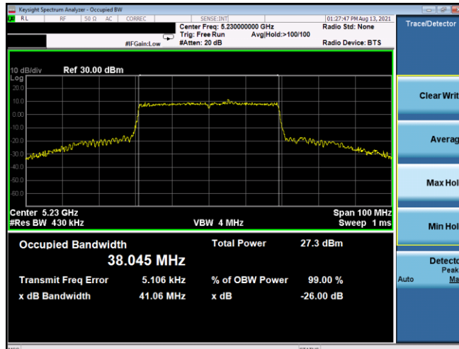
Plot 7-40. 26dB BW & 99% OBW Antenna 5T (40MHz BW 802.11ax(SU) – Ch. 46, MCS5)
