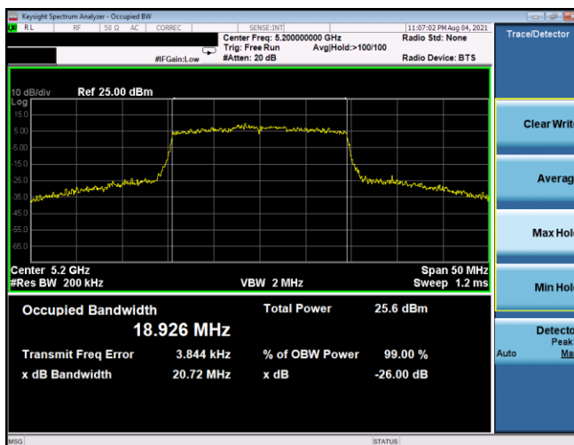
Plot 7-20. 26dB BW & 99% OBW Antenna 5T (20MHz BW 802.11ax(SU) - Ch. 40, MCS3)
