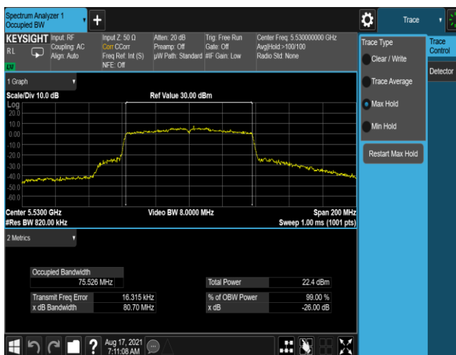
Plot 7-35. 26dB BW & 99% OBW Antenna 5T (80MHz BW 802.11ac – Ch. 106, MCS3)
