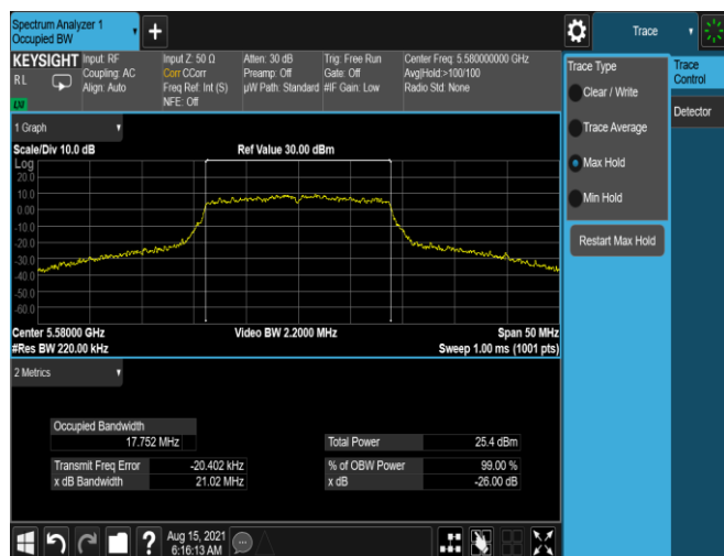
Plot 7-31. 26dB BW & 99% OBW Antenna 5T (20MHz BW 802.11n – Ch. 116, MCS3)
