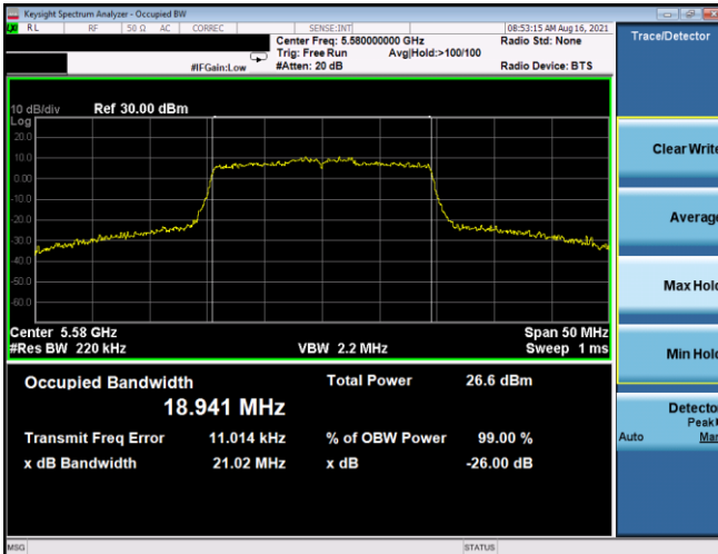
Plot 7-14. 26dB BW & 99% OBW Antenna 5T (20MHz BW 802.11ax(SU) - Ch. 116, MCS2)
