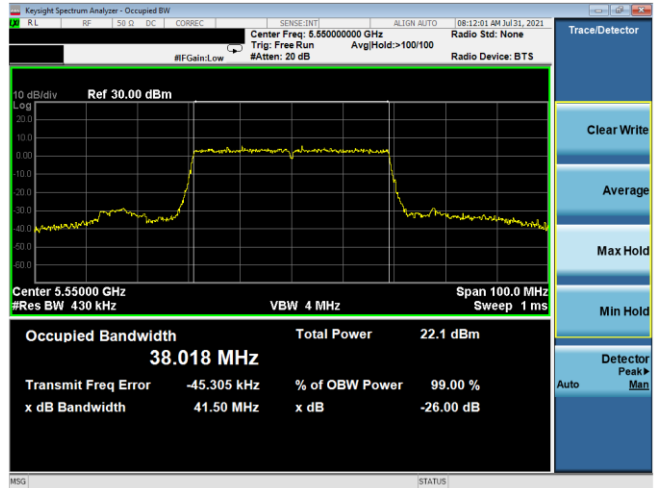
Plot 7-16. 26dB BW & 99% OBW Antenna 5T (40MHz BW 802.11ax(SU) - Ch. 110, MCS2)
