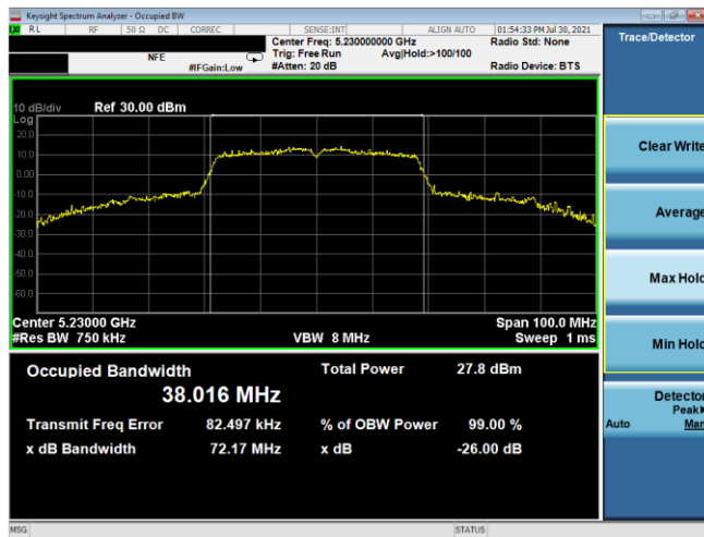
Plot 7-3. 26dB BW & 99% OBW Antenna 5T (40MHz BW 802.11n – Ch. 46, MCS2)
