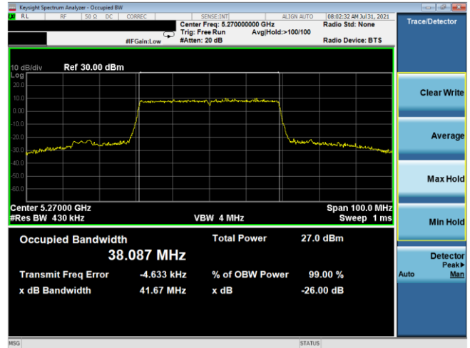
Plot 7-10. 26dB BW & 99% OBW Antenna 5T (40MHz BW 802.11ax(SU) – Ch. 54, MCS2)
