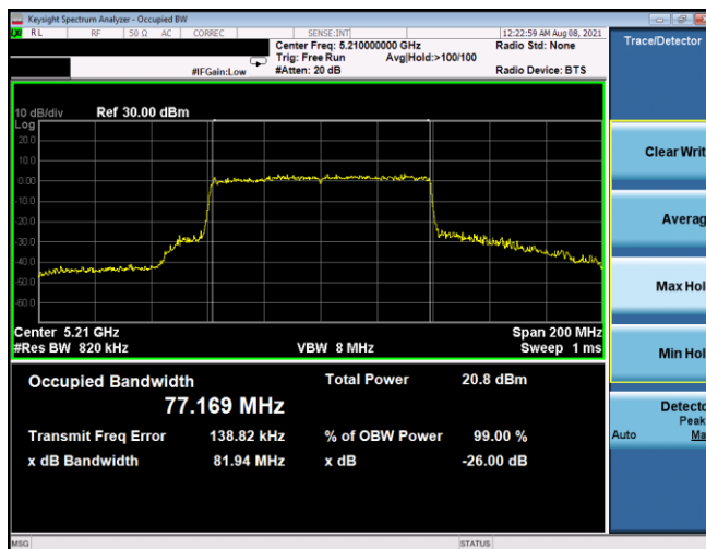
Plot 7-24. 26dB BW & 99% OBW Antenna 5T (80MHz BW 802.11ax(SU) - Ch. 42, MCS3)
