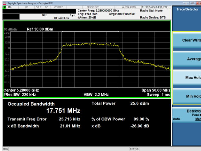
Plot 7-6. 26dB BW & 99% OBW Antenna 5T (20MHz BW 802.11n – Ch. 56, MCS2)
