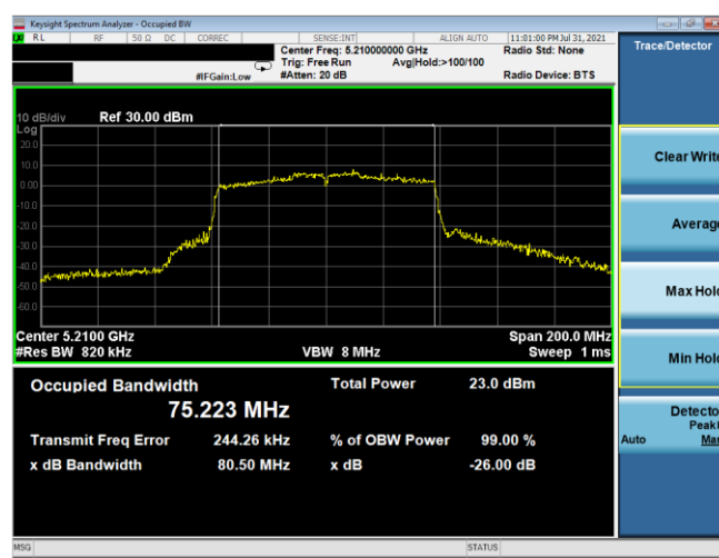
Plot 7-23. 26dB BW & 99% OBW Antenna 5T (80MHz BW 802.11ac - Ch. 42, MCS3)
