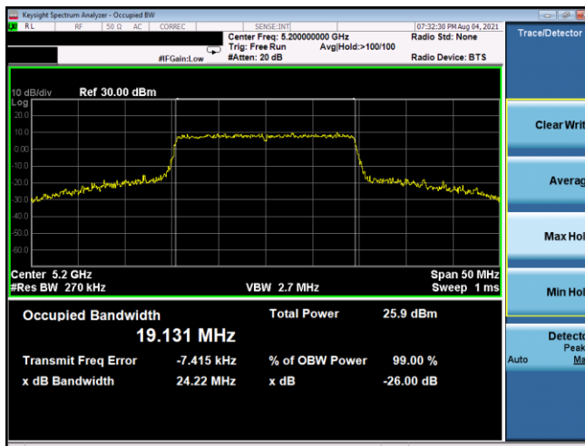
Plot 7-38. 26dB BW & 99% OBW Antenna 5T (20MHz BW 802.11ax(SU) – Ch. 40, MCS5)
