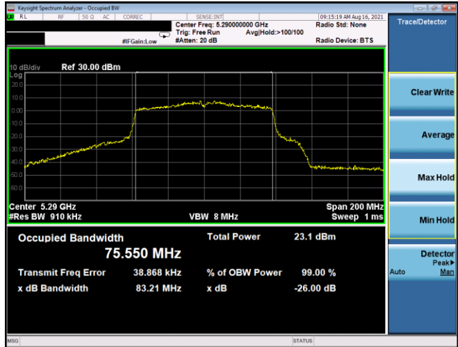
Plot 7-11. 26dB BW & 99% OBW Antenna 5T (80MHz BW 802.11ac – Ch. 58, MCS2)
