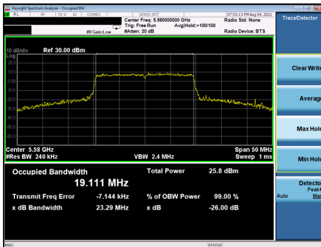
Plot 7-50. 26dB BW & 99% OBW Antenna 5T (20MHz BW 802.11ax(SU) – Ch. 116, MCS5)
