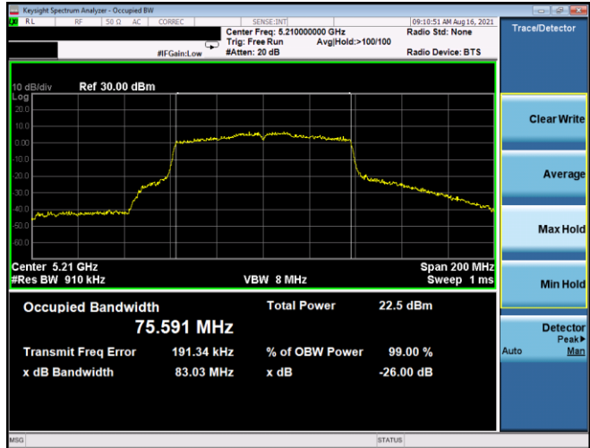
Plot 7-5. 26dB BW & 99% OBW Antenna 5T (80MHz BW 802.11ac – Ch. 42, MCS2)
