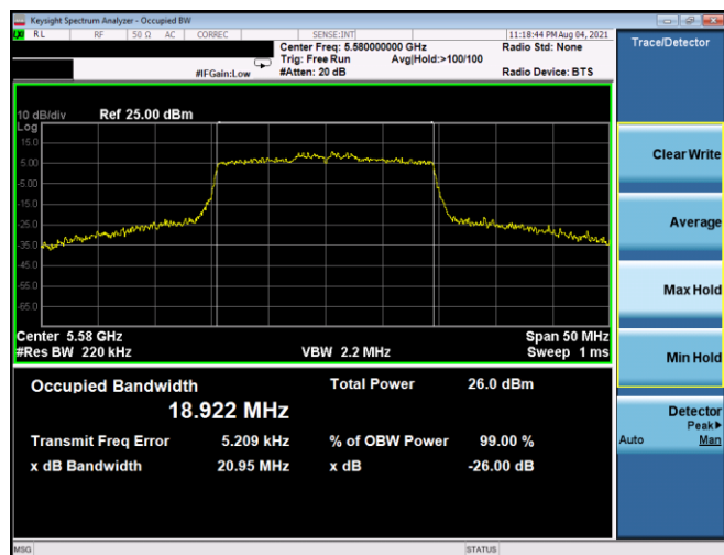
Plot 7-32. 26dB BW & 99% OBW Antenna 5T (20MHz BW 802.11ax(SU) – Ch. 116, MCS3)
