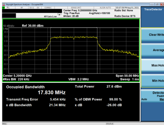
Plot 7-37. 26dB BW & 99% OBW Antenna 5T (20MHz BW 802.11n – Ch. 40, MCS5)
