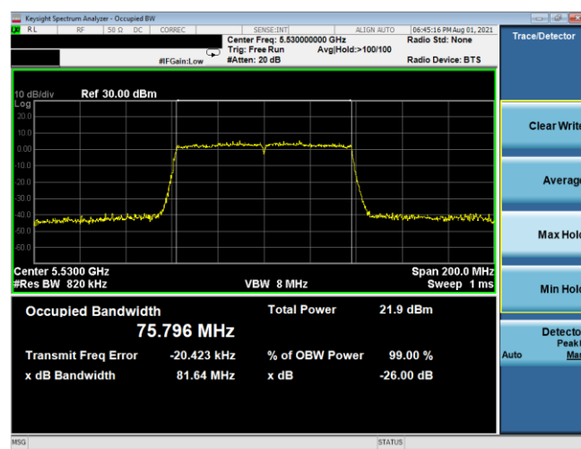
Plot 7-53. 26dB BW & 99% OBW Antenna 5T (80MHz BW 802.11ac – Ch. 106, MCS5)
