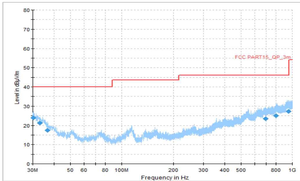
Figure A.1.7. Radiated Emission (GSM receiver 850MHz, 30MHz to 1GHz) Final_Results
