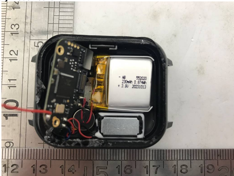
Battery Model: 552020
