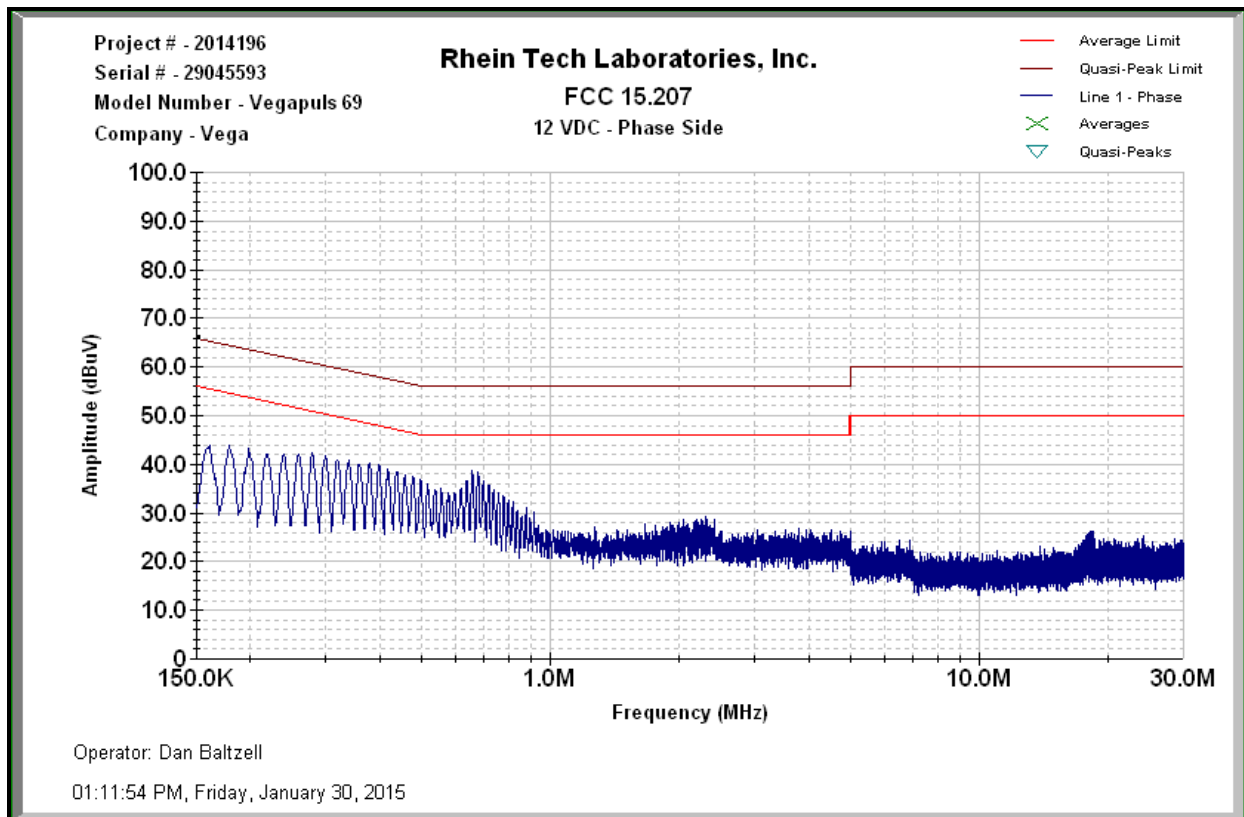
Plot 4-1: Conducted Emissions Transmit - Phase (TC #1)
