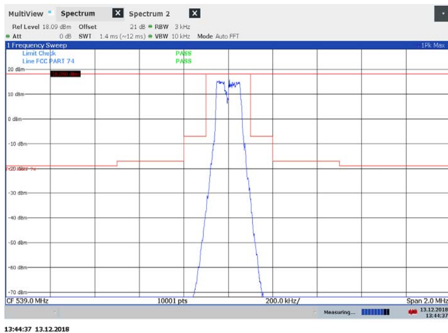
Plot 1: middle channel, Spectrum Mask
