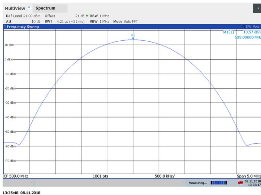
Plot 2: middle channel, peak (unmodulated carrier)
