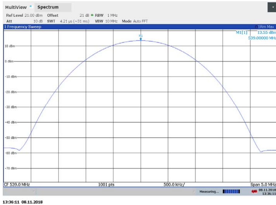
Plot 1: middle channel, average (modulated carrier)
