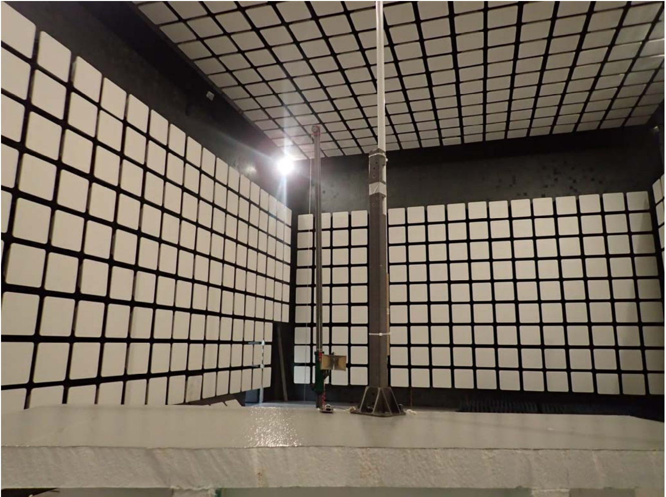
Radiated Emissions @ 3 m, Above 1 GHz EUT with 8.15 dBi Omni Directional Antenna
