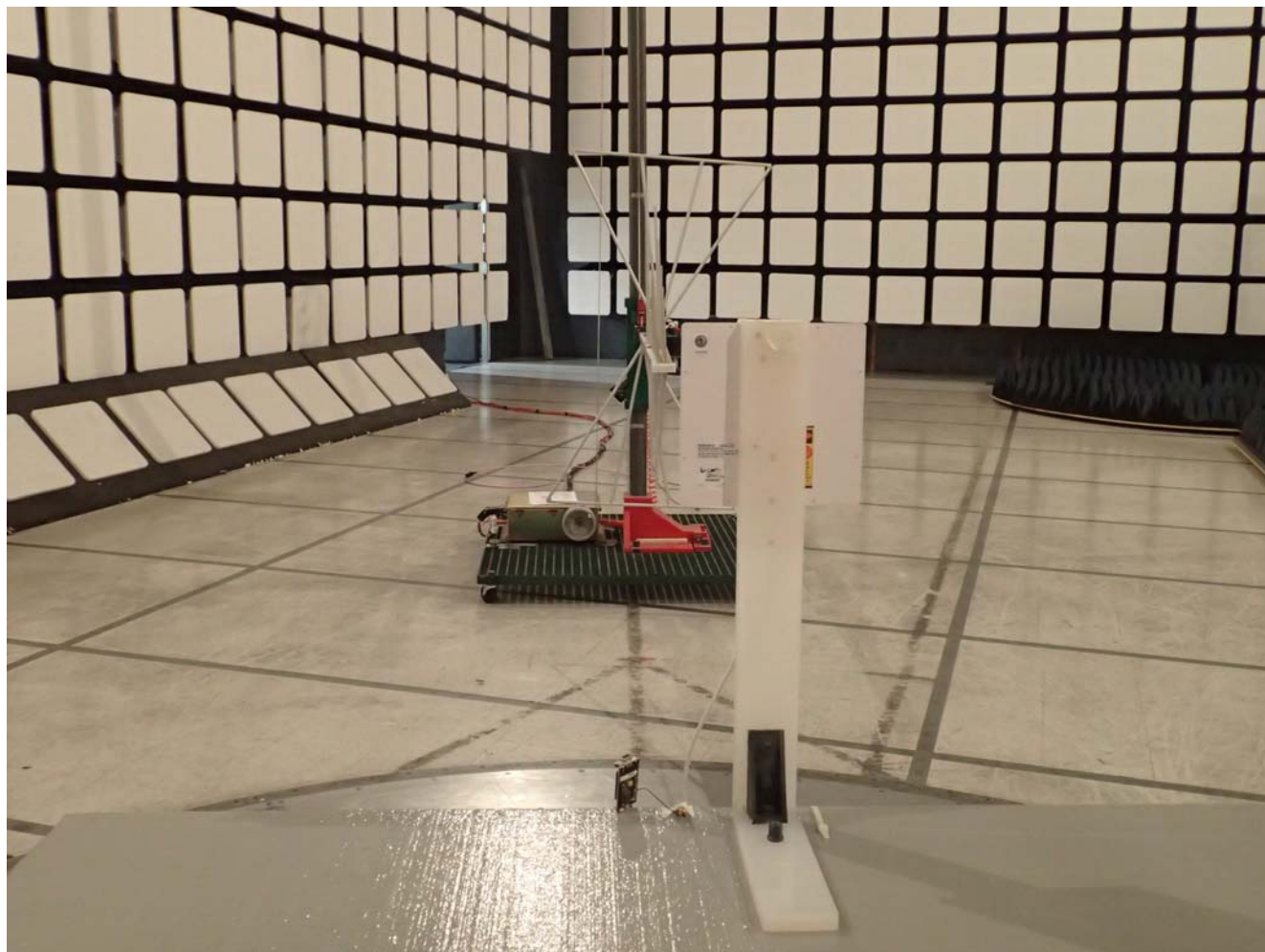
Radiated Emissions @ 3 m, 30 – 1000 MHz EUT with 8 dBi Flat Patch Antenna
