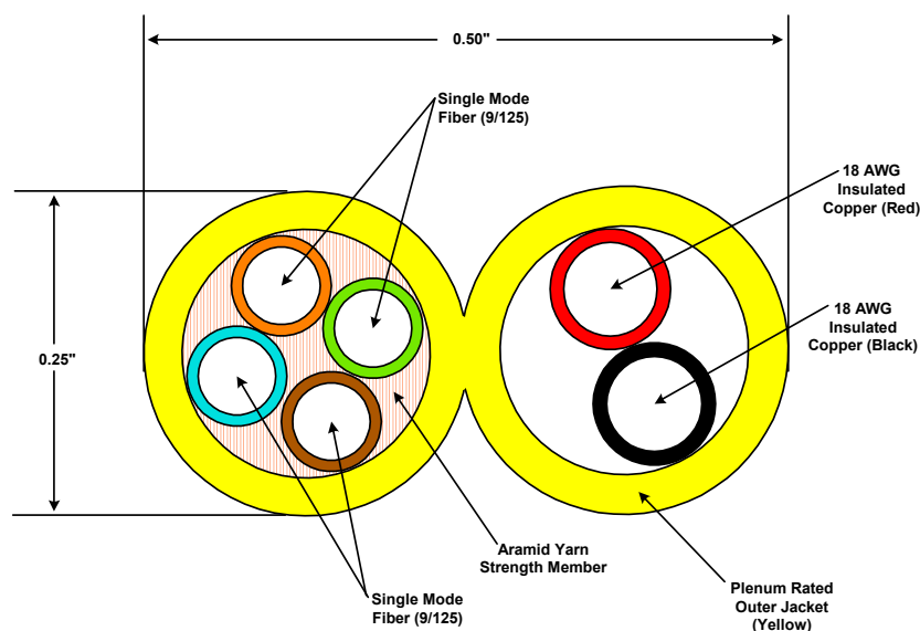
Figure 3-2. Cross Section of Andrew Composite Fiber/Copper Cable
