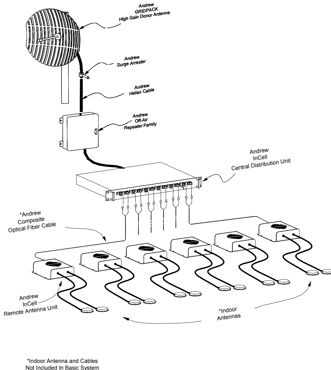
Figure 4-3. Typical System Configuration Using Off-Air Interface
