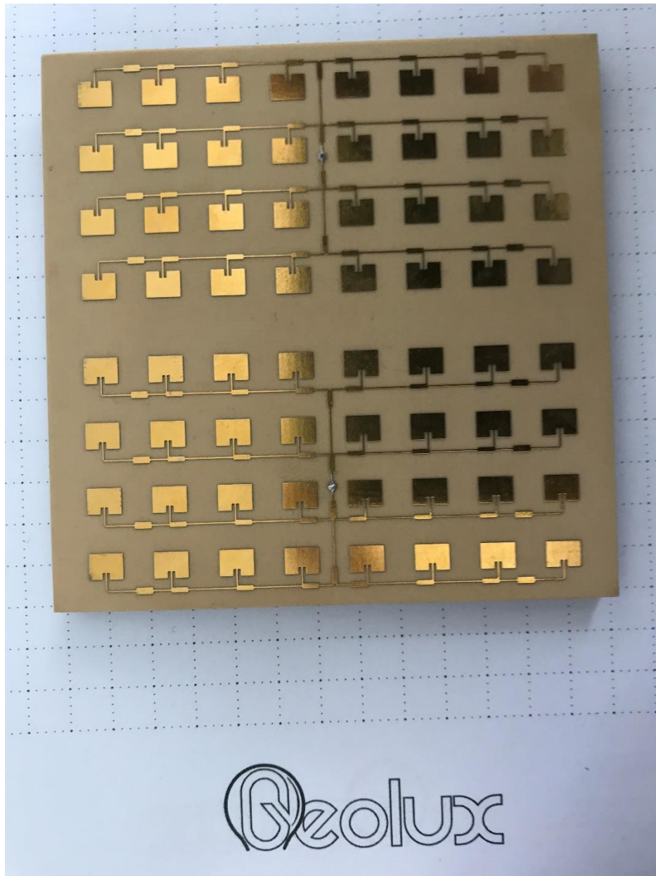
7. RSS-2-300W microwave transceiver antenna board front view
