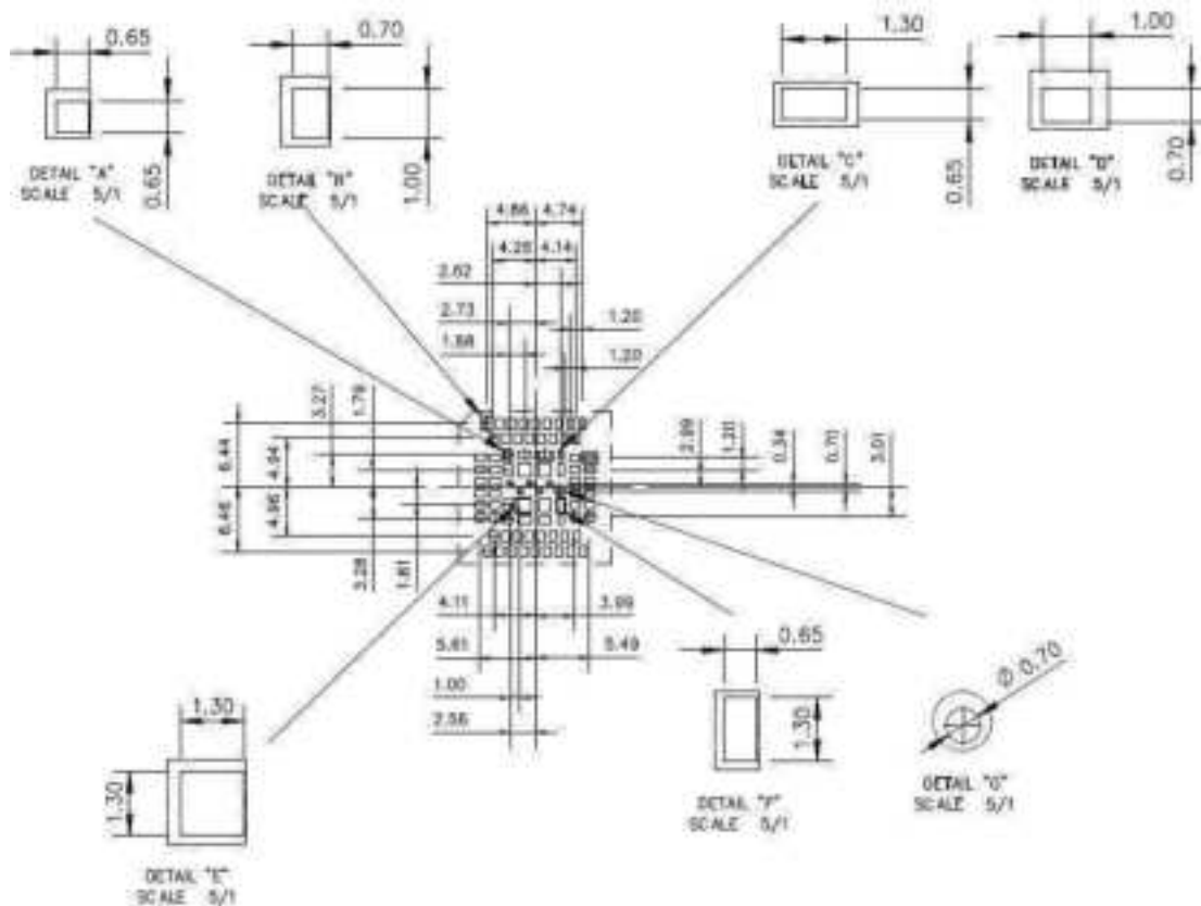
Figure 4-4. Pin dimensions
