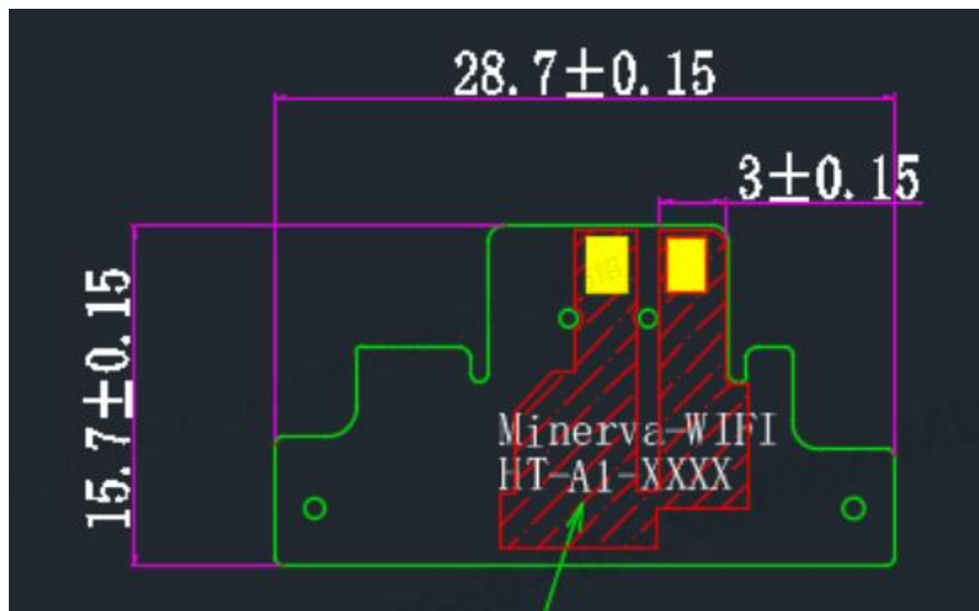
Antenna layout pattern
