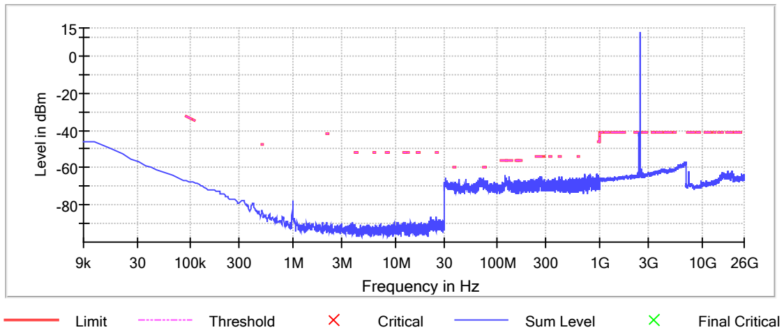
Restricted Band
