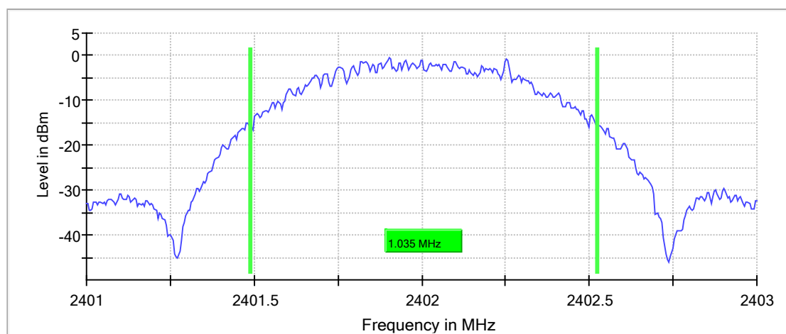
99 % Bandwidth
