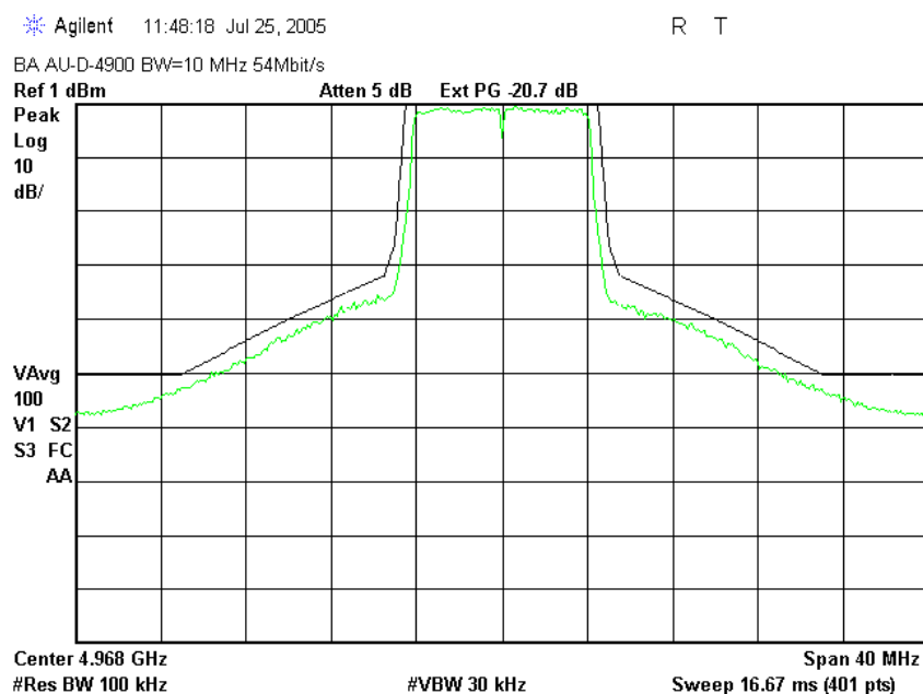
Plot # 17. HIGH frequency 4.968 GHz, Bandwidth = 10 MHz, PRBS = 54 MBit/s
