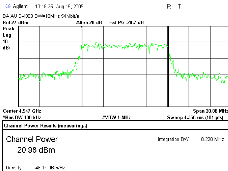
Plot # 43. LOW frequency 4.947 GHz, Bandwidth = 10 MHz, PRBS = 54 MBit/s
