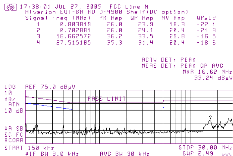
Plot # 6. Base Station Unit (BS-SH Shelf, DC option) Conducted emissions measurement result on 115 VAC power line: neutral
