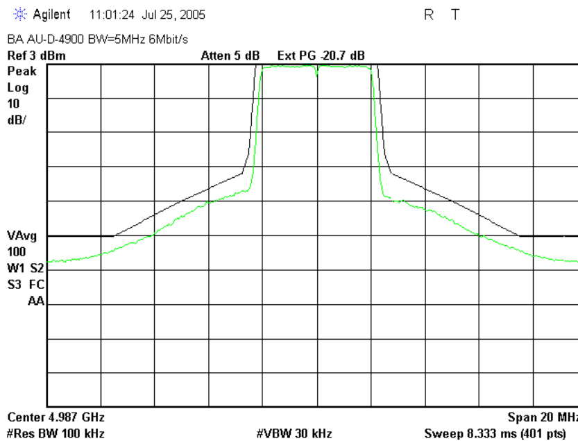
Plot # 9. HIGH frequency 4.987 GHz, Bandwidth = 5 MHz, PRBS = 6 MBit/s
