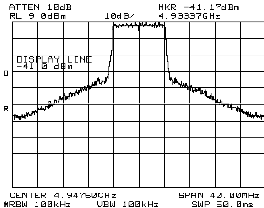
Plot # 19. Carrier, LOW frequency 4.9475 GHz,
