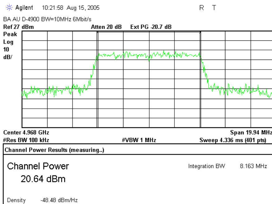
Plot # 41. MIDDLE frequency 4.968 GHz, Bandwidth = 10 MHz, PRBS = 6 MBit/s
