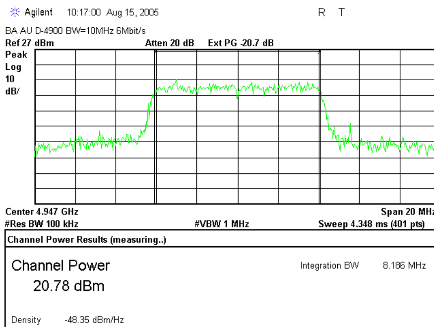
Plot # 40. LOW frequency 4.947 GHz, Bandwidth = 10 MHz, PRBS = 6 MBit/s
