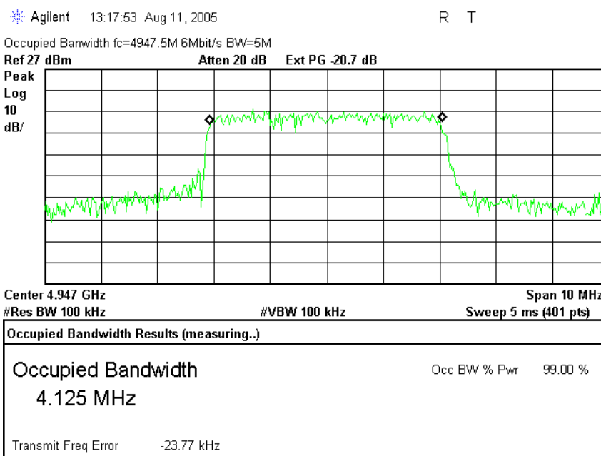
Plot #58. LOW frequency 4.947 GHz, Bandwidth = 5 MHz, PRBS = 6 Mbit/s
