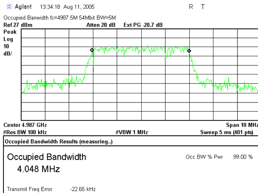
Plot # 58. HIGH frequency 4.987 GHz, Bandwidth = 5 MHz, PRBS = 54 Mbit/s
