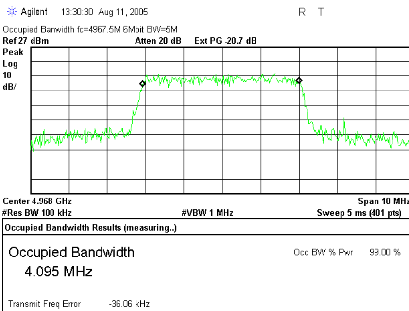
Plot # 62. Middle frequency 4.968 GHz, Bandwidth = 5 MHz, PRBS = 6 Mbit/s
