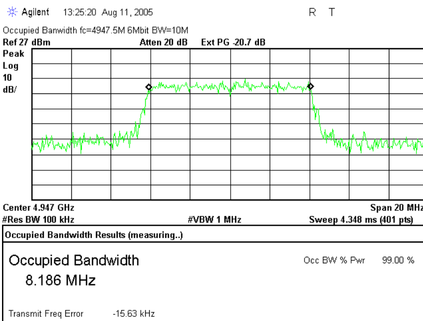
Plot # 60. LOW frequency 4.947 GHz, Bandwidth = 10 MHz, PRBS = 6 Mbit/s
