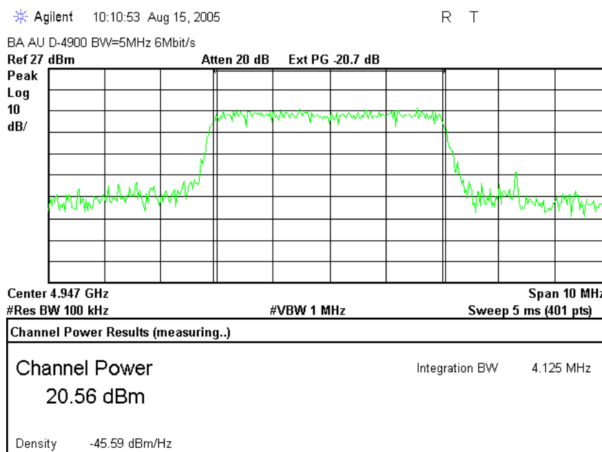
Plot # 34. LOW frequency 4.947 GHz, Bandwidth = 5 MHz, PRBS = 6 MBit/s
