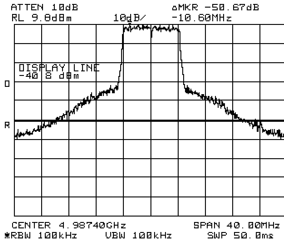
Plot # 29. Carrier, HIGH frequency 4.9875 GHz,
