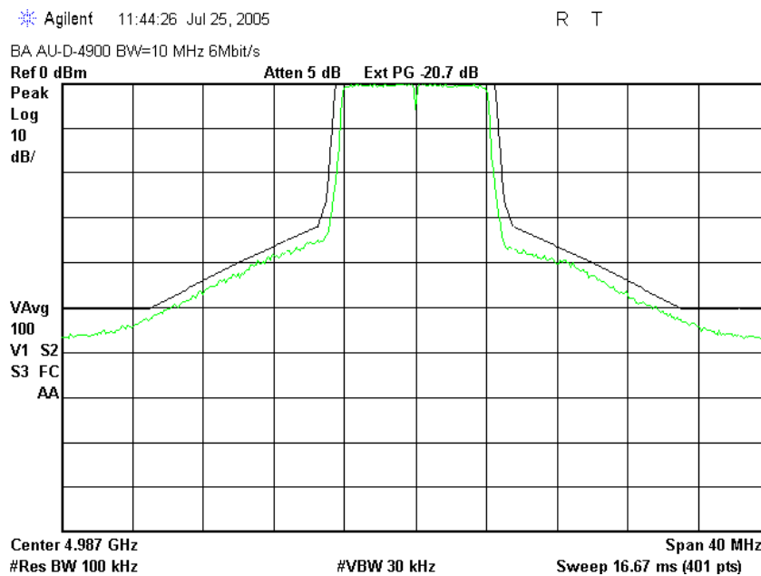
Plot # 15. HIGH frequency 4.987 GHz, Bandwidth = 10 MHz, PRBS = 6 MBit/s,
