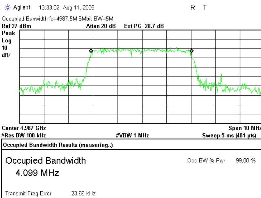
Plot # 66. HIGH frequency 4.987 GHz, Bandwidth = 5 MHz, PRBS = 6 Mbit/s
