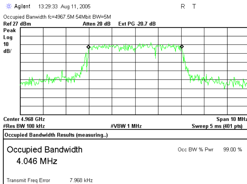
Plot # 63. Middle frequency 4.968 GHz, Bandwidth = 5 MHz, PRBS = 54 Mbit/s
