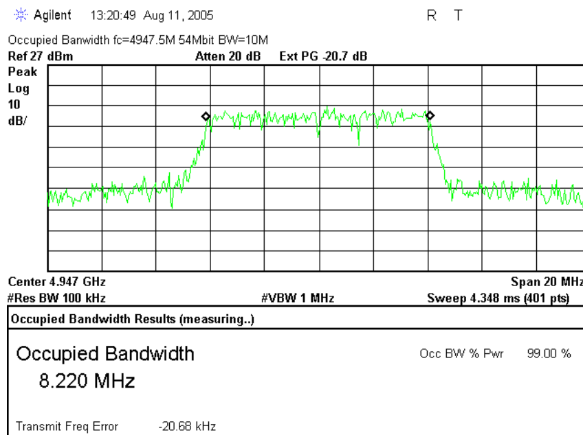
Plot # 61. LOW frequency 4.947 GHz, Bandwidth = 10 MHz, PRBS = 54 Mbit/s
