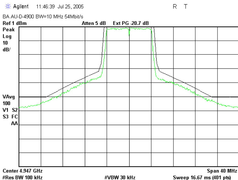
Plot # 16. LOW frequency 4.947 GHz, Bandwidth = 10 MHz, PRBS = 54 MBit/s,
