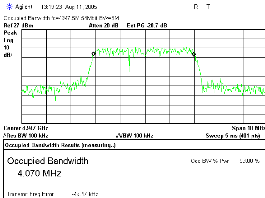
Plot # 59. LOW frequency 4.947 GHz, Bandwidth = 5 MHz, PRBS = 54 Mbit/s
