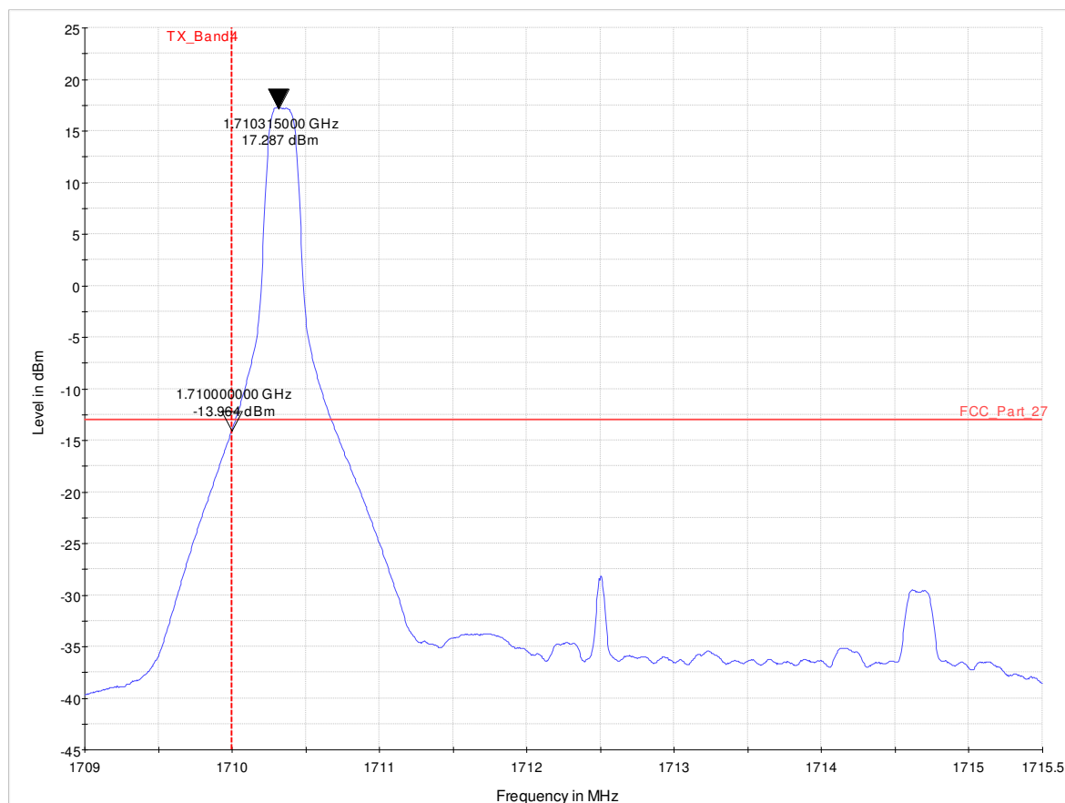
Diagram 37.01_Ch19975_QPSK_1RB_Low_5MHz
