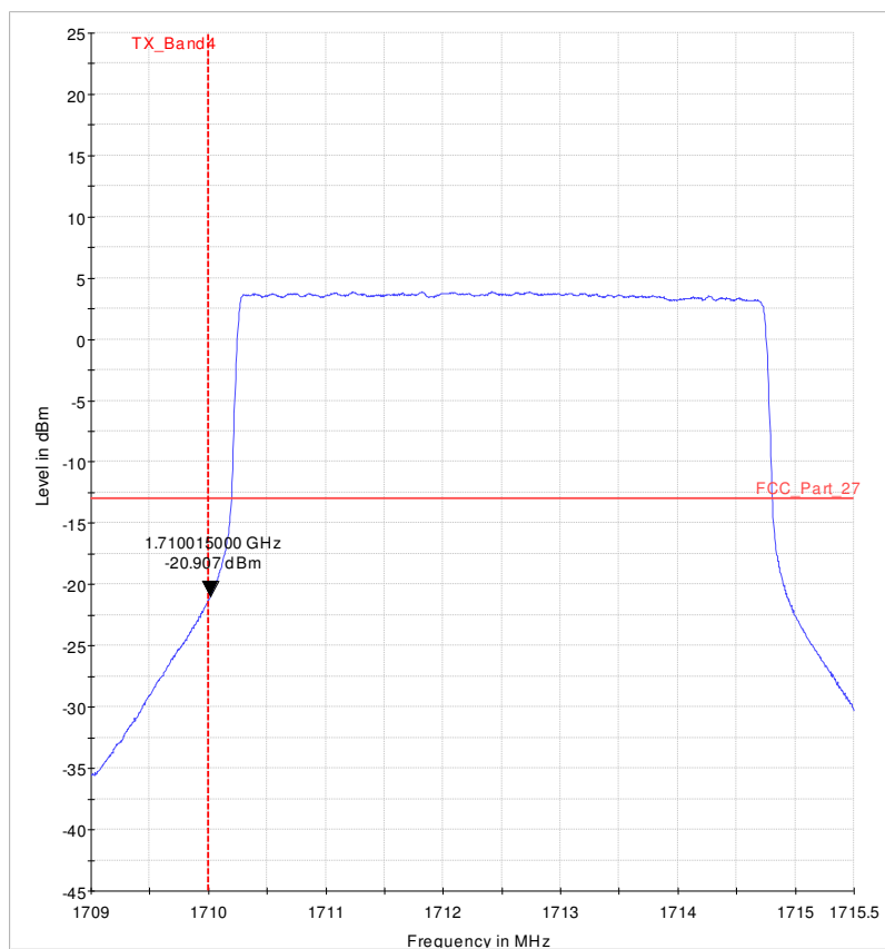
Diagram 37.03_Ch19975_QPSK_25RBlow_5MHz
