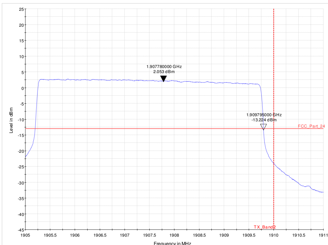
Diagram 37.23_CH19175_16QAM_25RBhigh_5MHZ
