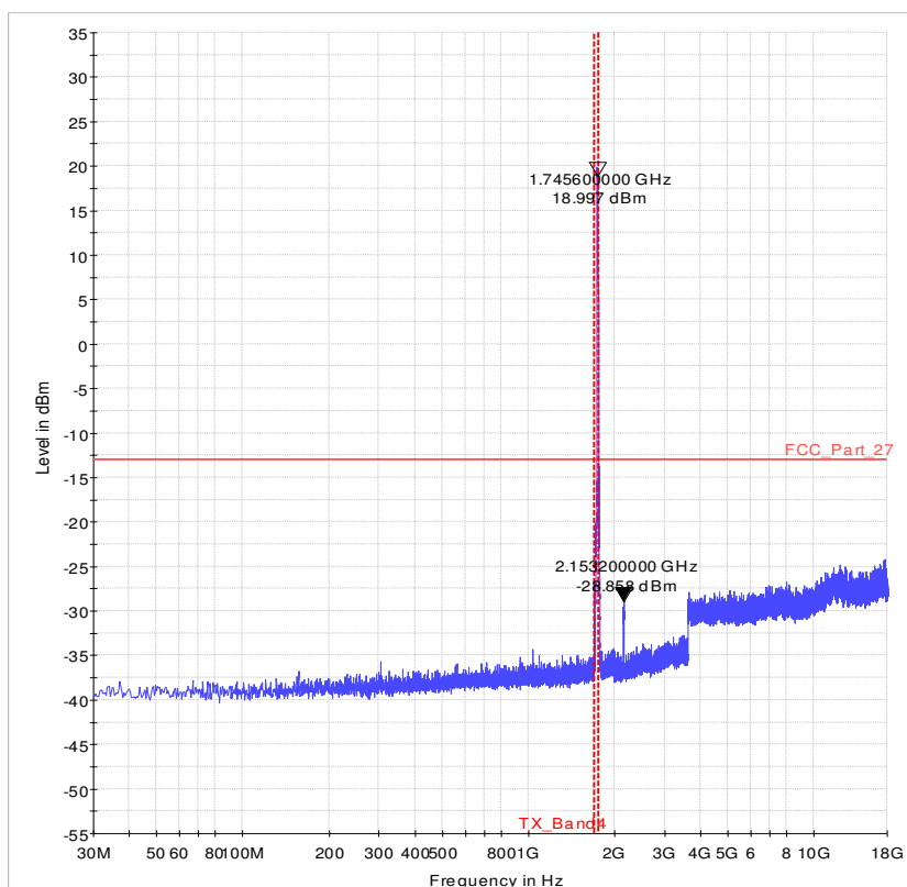
Diagram 36.10_Ch20300_QPSK_100RBS_20MHz_Sweep2
