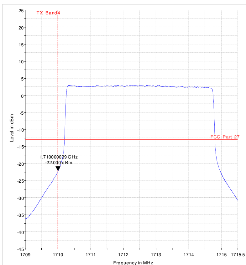
Diagram 37.04_Ch19975_16QAM_25RBlow_5MHz
