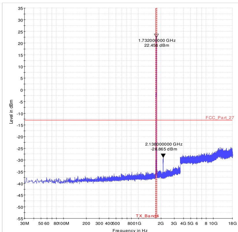
Diagram 36.06_Ch20175_16QAM_100RB_20MHz_Sweep1
