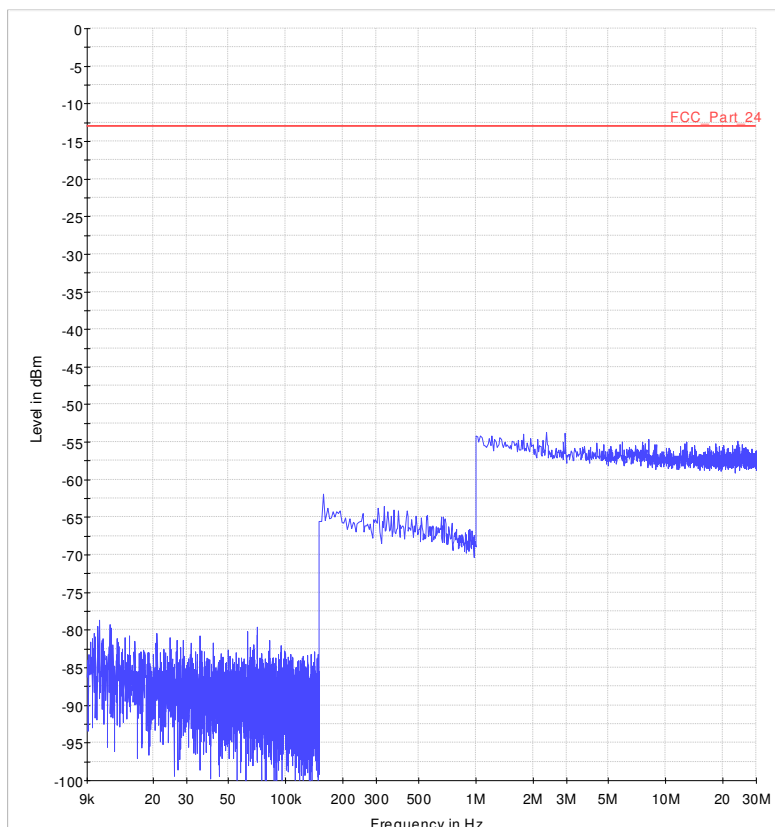
Diagram 36.06_Ch20175_16QAM_100RB_20MHz_Sweep1
