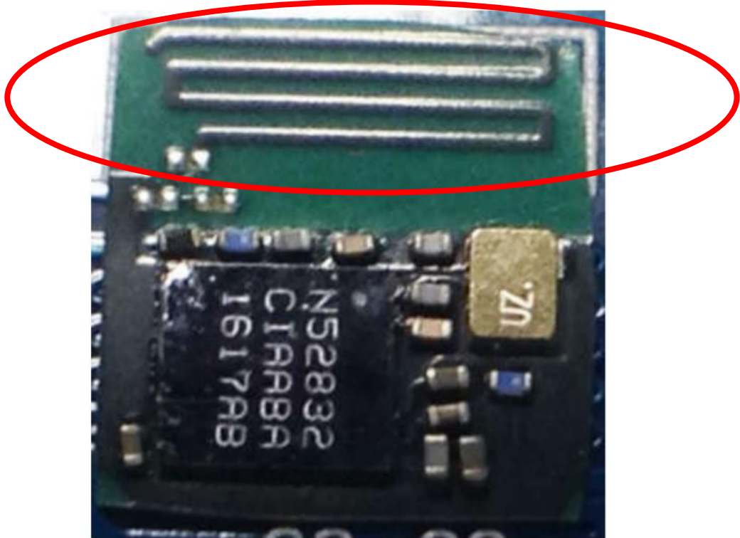
BT Antenna
