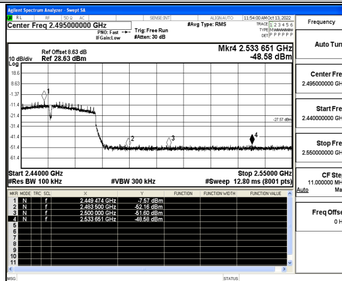
11N40SISO_Ant_High_2452
