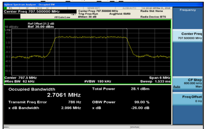
Band12_3MHz_64QAM_15_0_MidCH23095-707.5
