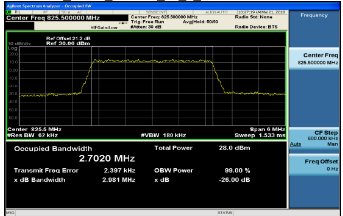
Band5 3MHz 64QAM 15 0 LowCH20415-825.5
