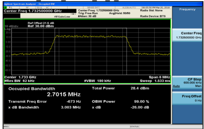
Band4_3MHz_64QAM_15_0_MidCH20175-1732.5
