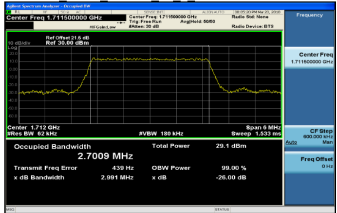
Band4_3MHz_64QAM_15_0_LowCH19965-1711.5
