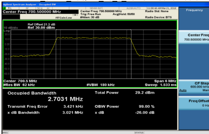
Band12_3MHz_16QAM_15_0_LowCH23025-700.5
