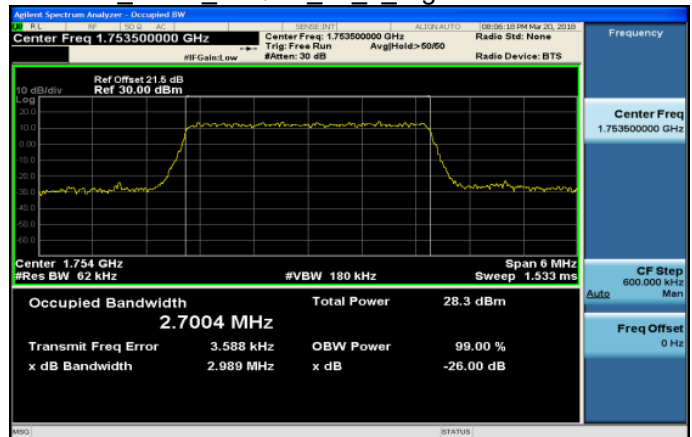
Band4_3MHz_64QAM_15_0_HighCH20385-1753.5
