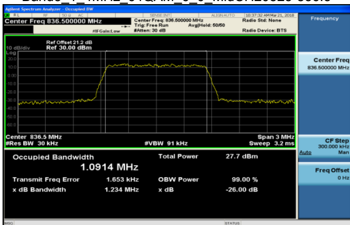
Band5 1 4MHz 64QAM 6 0 MidCH20525-836.5
