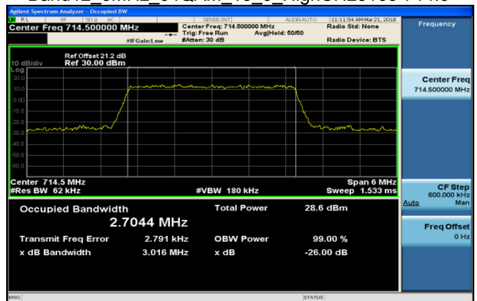
Band12_3MHz_64QAM_15_0_HighCH23165-714.5
