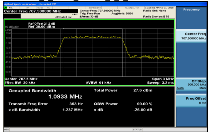
Band12_1_4MHz_16QAM_6_0_MidCH23095-707.5
