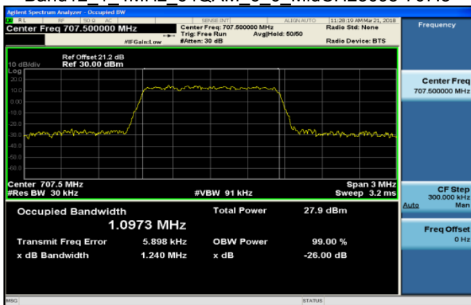
Band12 1 4MHz 64QAM 6 0 MidCH23095-707.5
