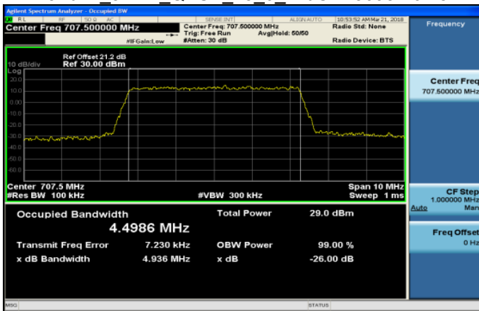
Band12 5MHz QPSK 25 0 MidCH23095-707.5
