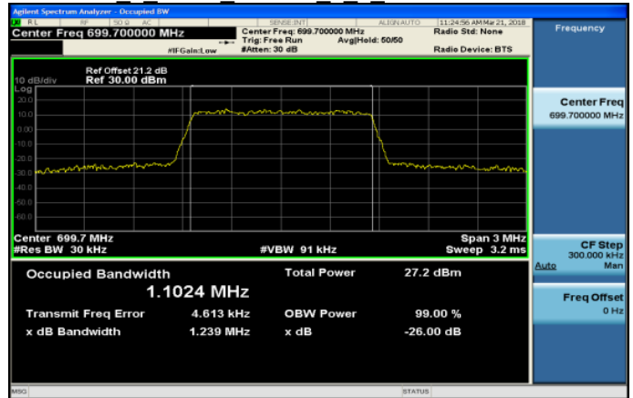
Band12_1_4MHz_16QAM_6_0_LowCH23017-699.7
