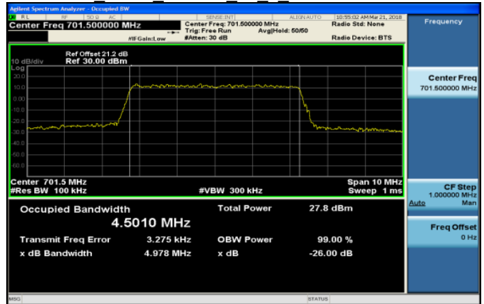
Band12 5MHz 16QAM 25 0 LowCH23035-701.5
