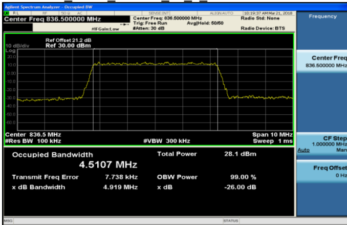
Band5 5MHz 64QAM 25 0 MidCH20525-836.5
