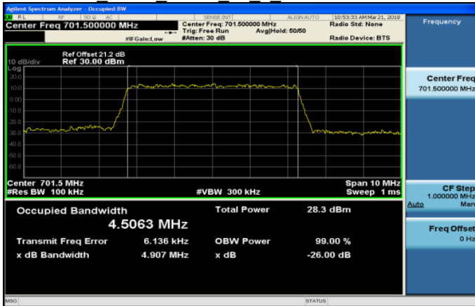
Band12 5MHz QPSK 25 0 LowCH23035-701.5
