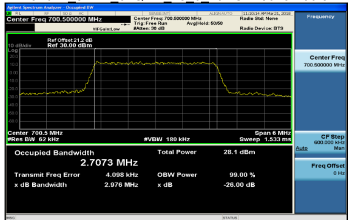
Band12_3MHz_64QAM_15_0_LowCH23025-700.5
