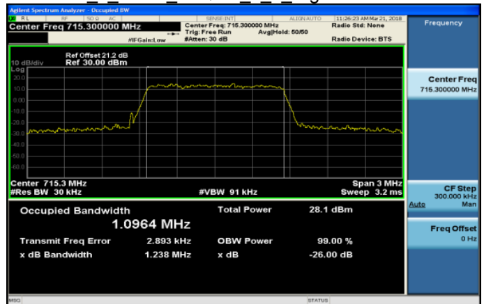
Band12_1_4MHz_16QAM_6_0_HighCH23173-715.3
