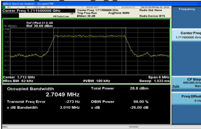
Band4_3MHz_16QAM_15_0_LowCH19965-1711.5
