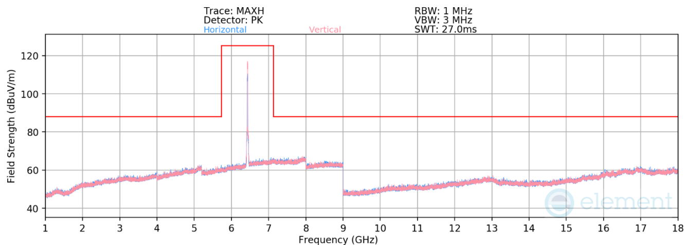
Plot 7-538. Radiated Spurious Emissions above 1GHz CDD Primary (802.11ax – Ch. 97)
