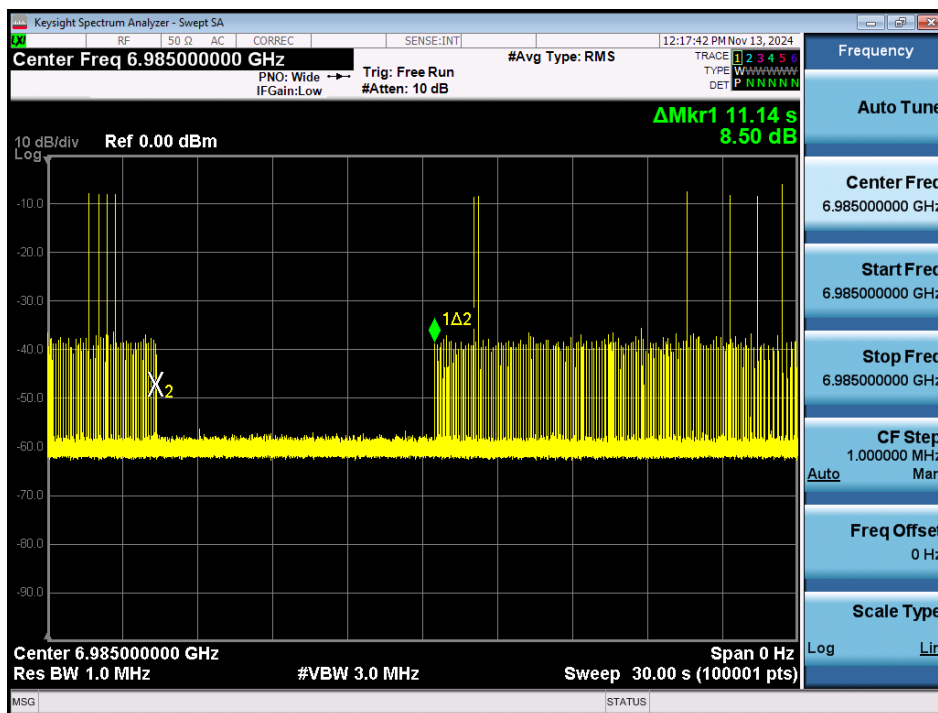
Plot 7-528. Contention Based Protocol Timing Plot – UNII 8 – 160MHz Channel 207 – Mid
