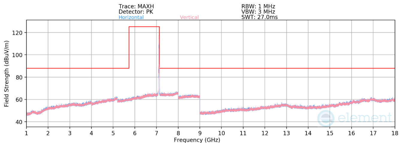
Plot 7-549. Radiated Spurious Emissions above 1GHz CDD Primary (802.11ax – Ch. 233)
