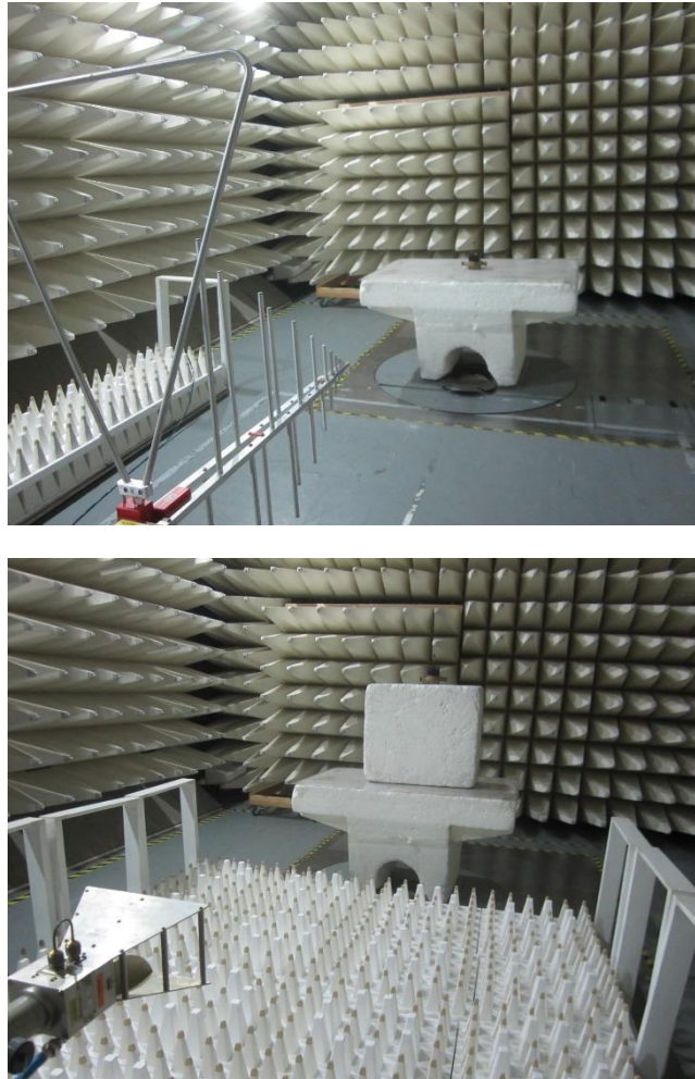
Photograph No.3 Setup for spurious emission measurements in the anechoic chamber above 30 MHz
