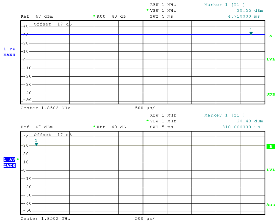
(Plot A1: GSM 1900 MHz Channel = 512)
