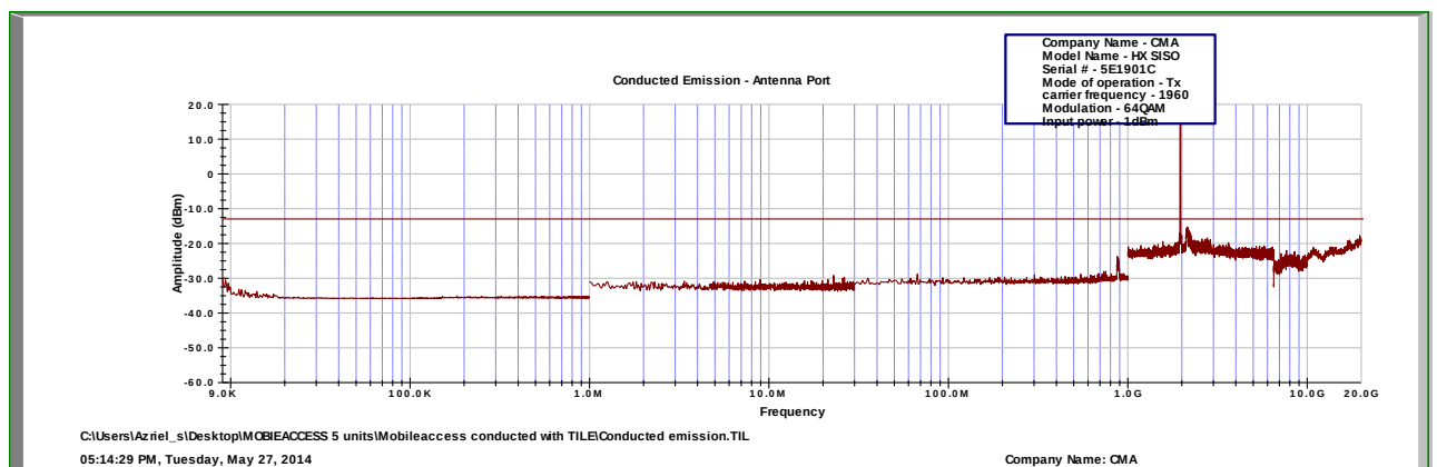
Figure 90.— 1960 MHz
