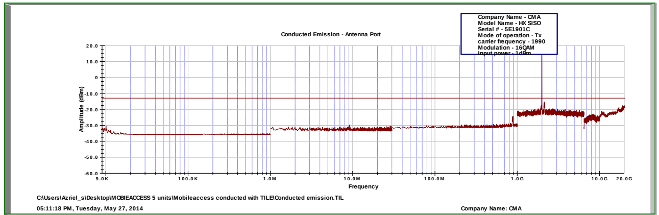
Figure 88.— 1990 MHz
