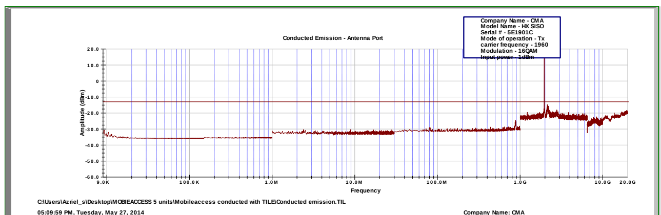
Figure 87.— 1960 MHz
