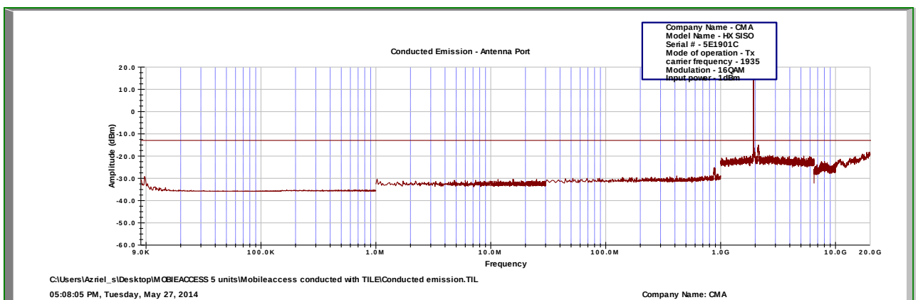
Figure 86.— 1935 MHz
