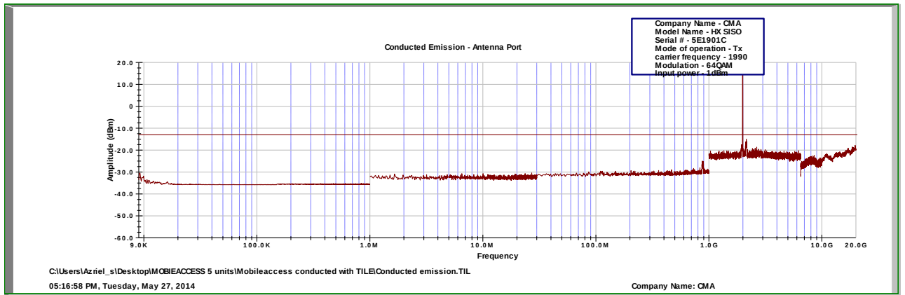
Figure 91.— 1990 MHz
