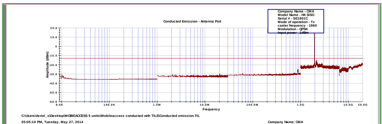
Figure 84.— 1960 MHz
