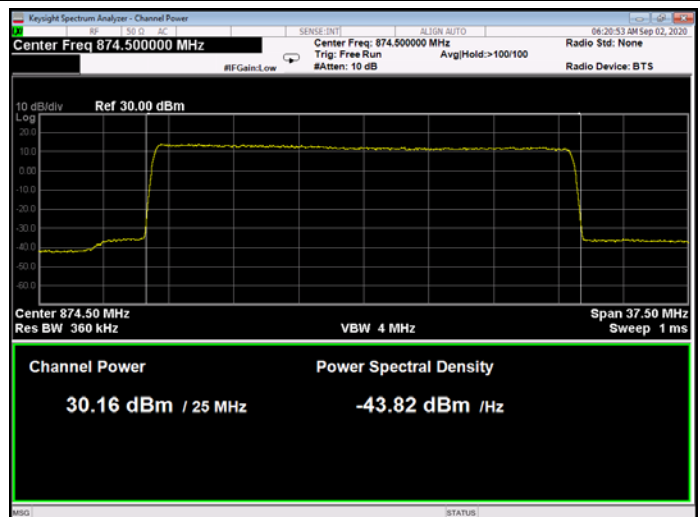
Figure 125: 256QAM 25MHz B.W.; 874.5MHz, 15kHz
