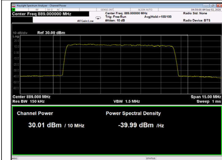
Figure 106: 256QAM 10MHz B.W.; 889.0MHz, 60kHz
