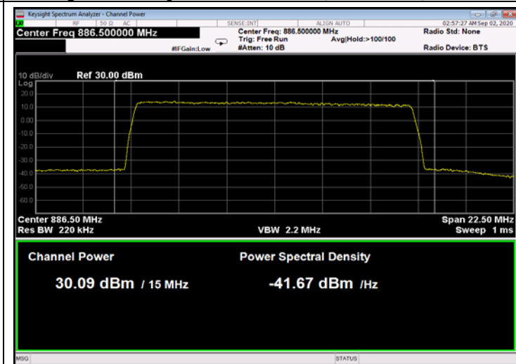
Figure 157: QPSK 15MHz B.W.; 886.5MHz, 60kHz
