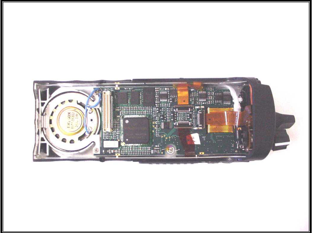
PHOTOGRAPH 16: USER INTERFACE BOARD IN FRONT COVER
