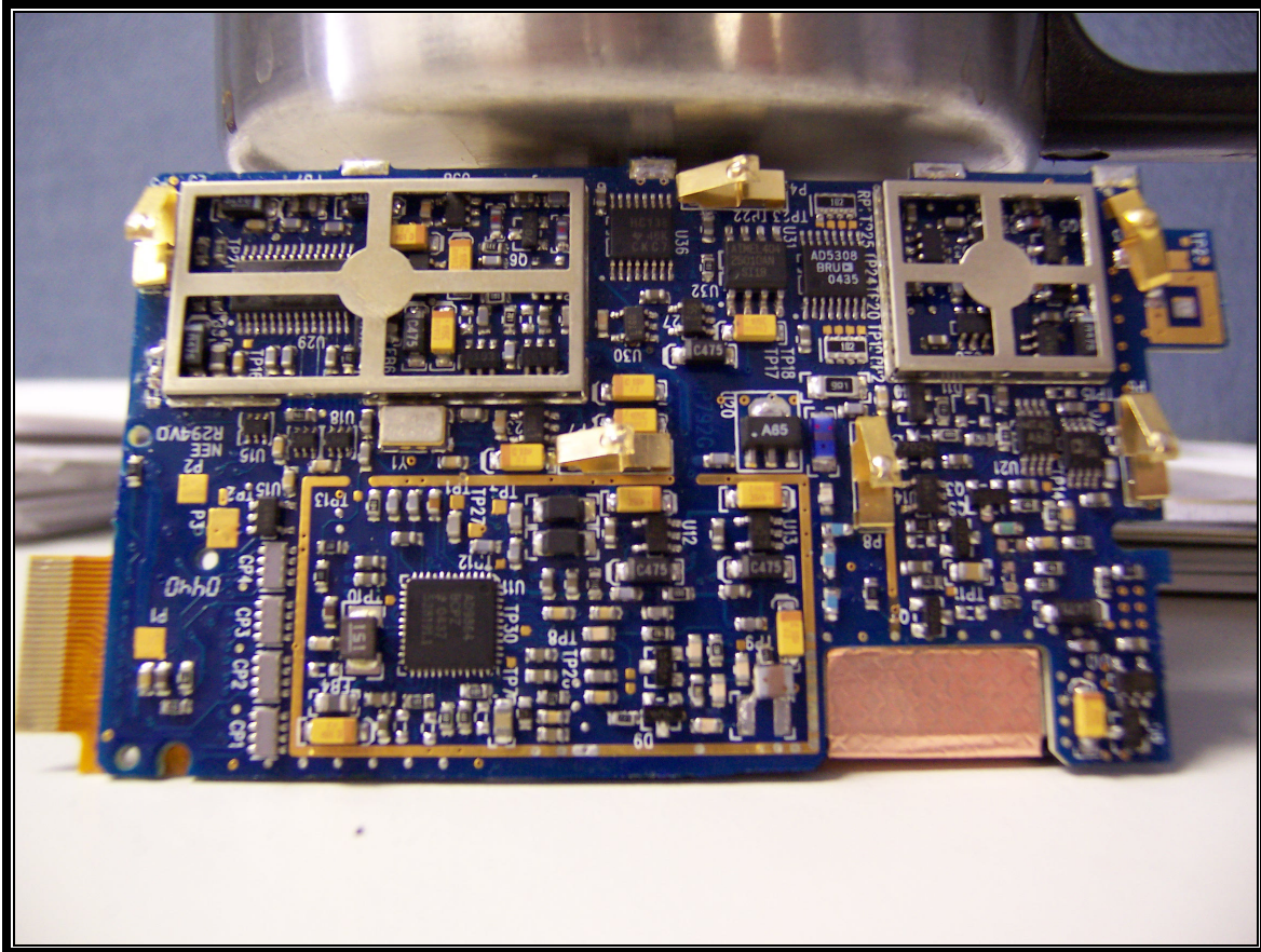
PHOTOGRAPH 15: RF BOARD BOTTOM VIEW
