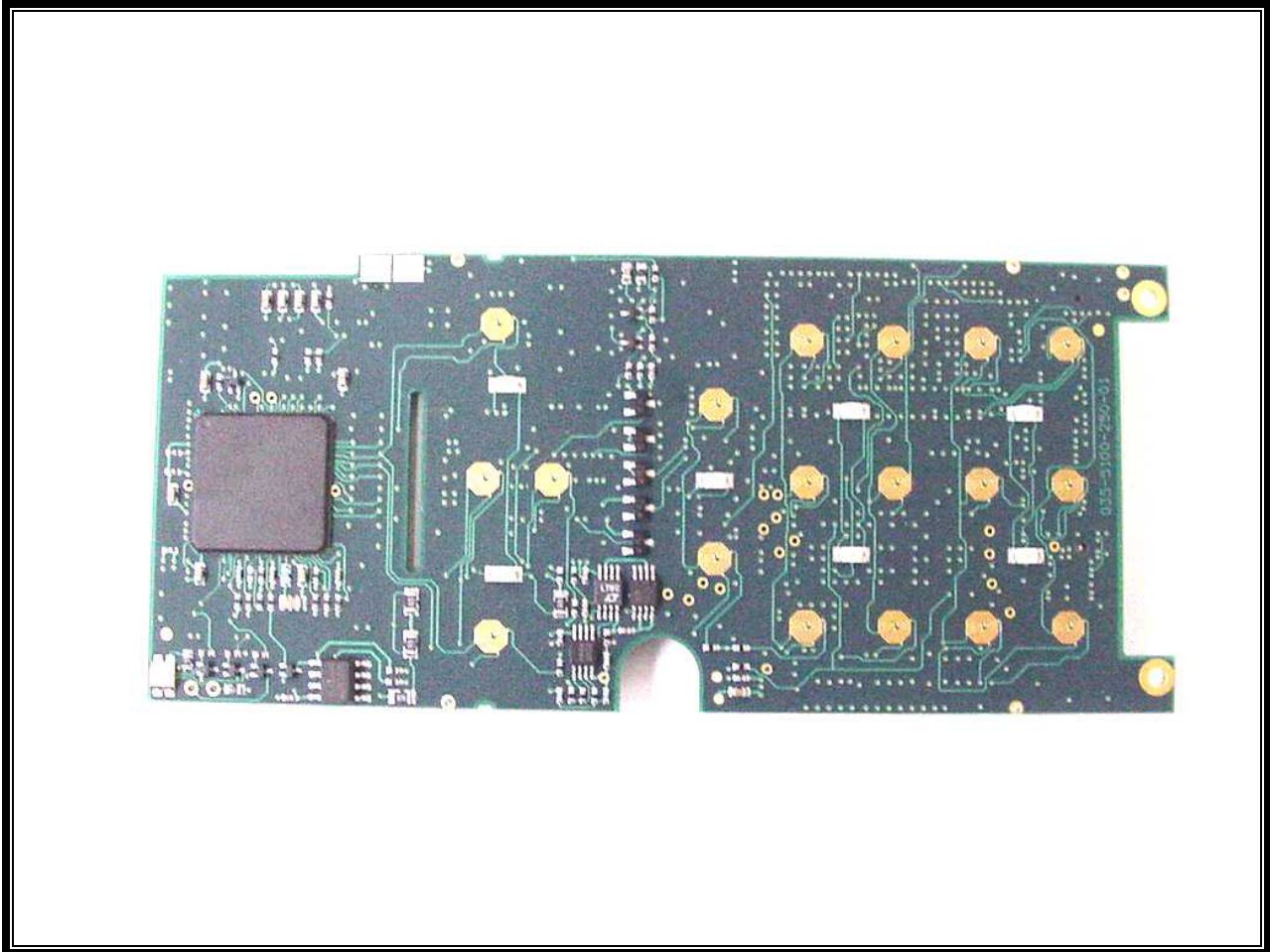
PHOTOGRAPH 17: USER INTERFACE BOARD FRONT VIEW
