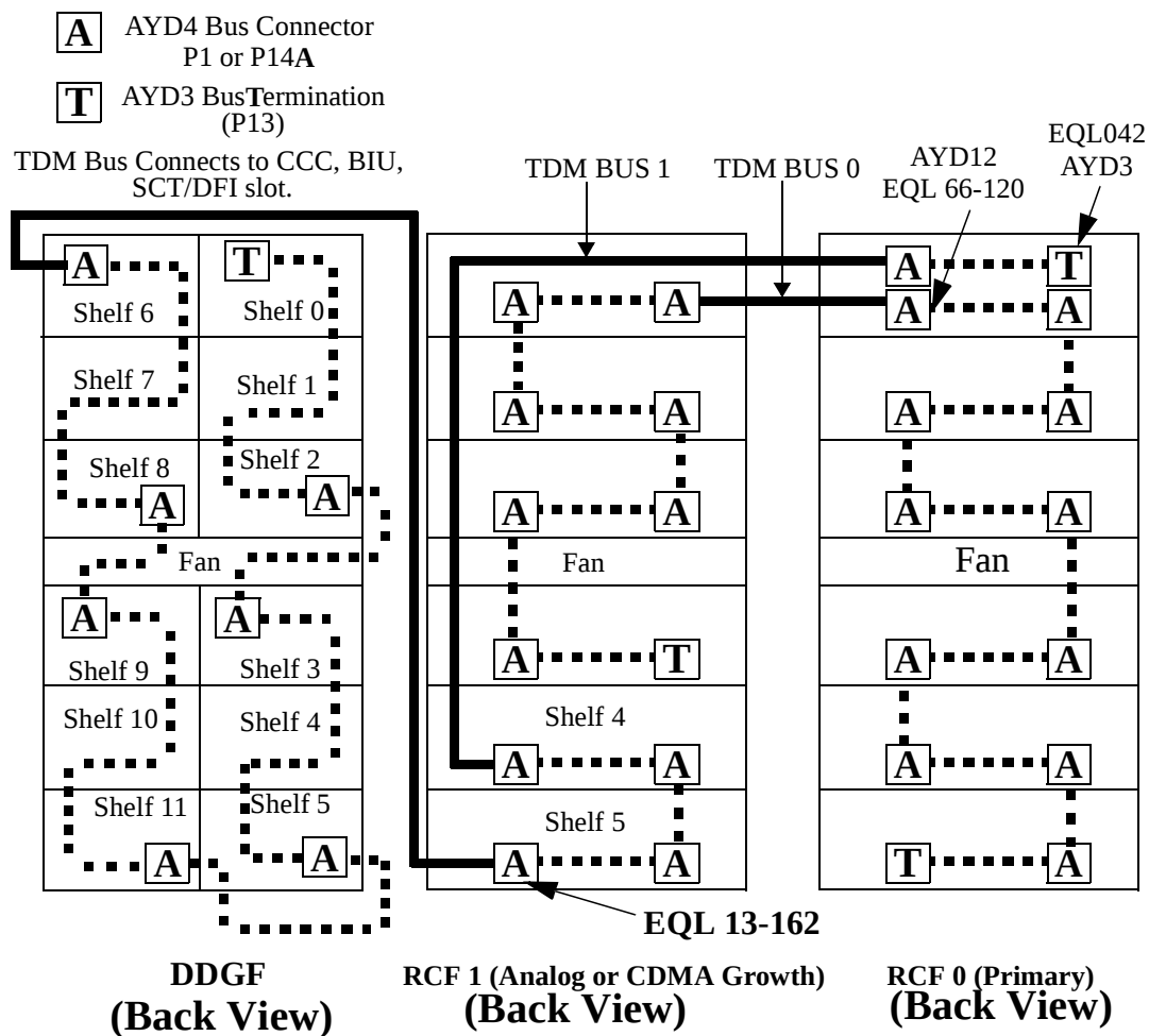
Figure 4-29. TDM Bus Installation. TDM bus cables are installed "red stripe up." (Configurations 4 and 5)
