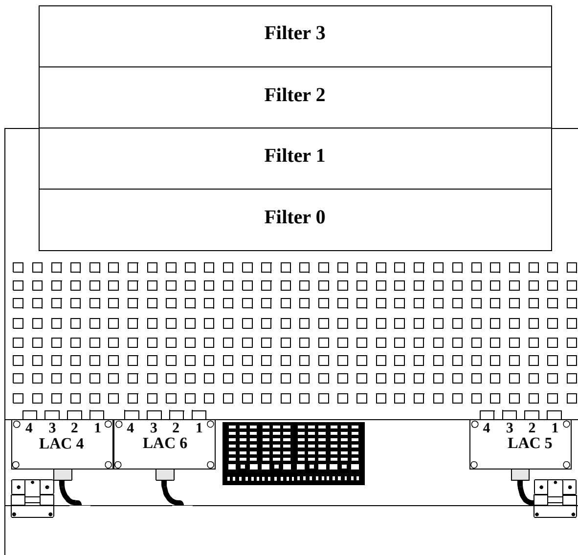
Figure 4-25. Top of LAF 1, MLAC Power Divider Input
