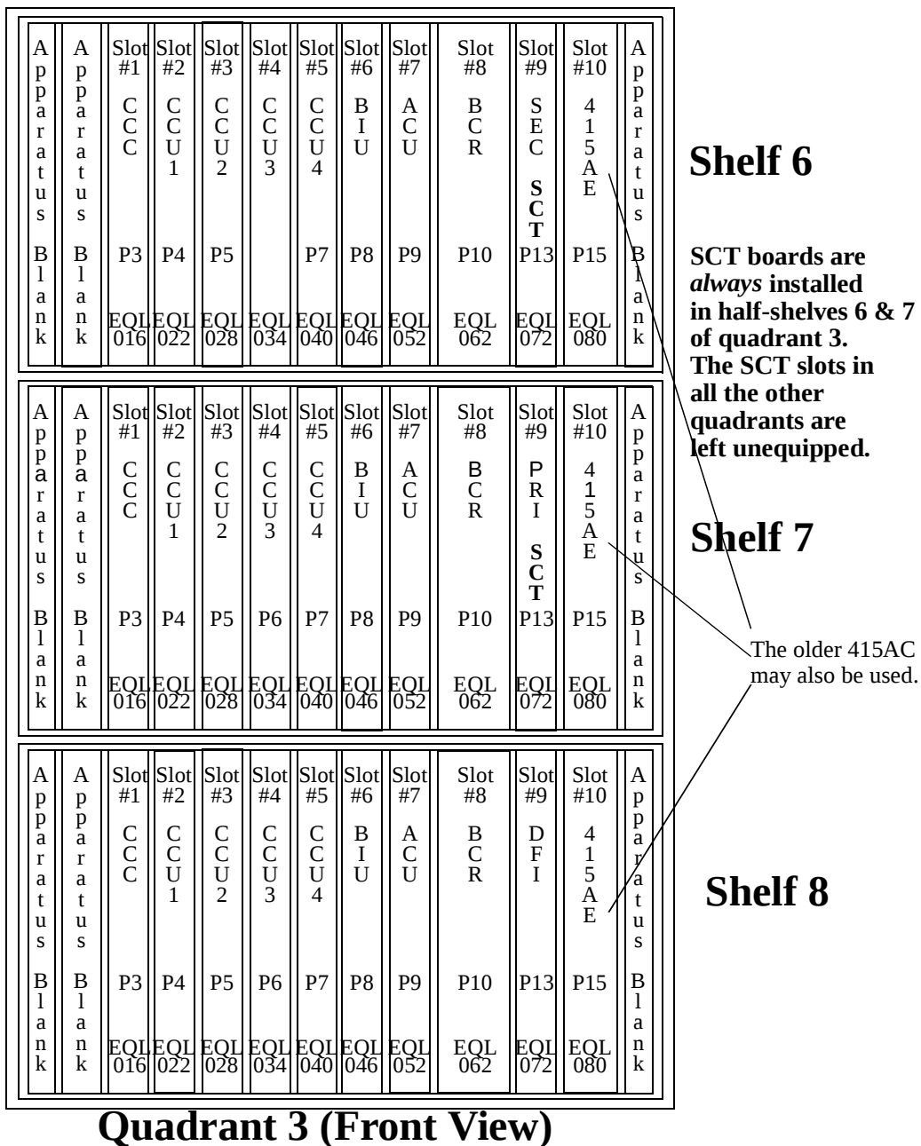
Figure 4-14. Illustration of Circuit Packs Populating the CRC
