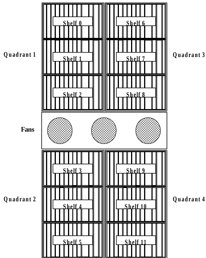
Figure 4-13. Quadrant and Half-shelf Numbering of DDGF (Front View)
