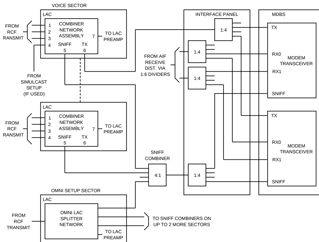
Figure 6-17. Multiple Modem Transceiver per Sector, Multiple LACs per Sector - Sniffing on Multiple LACs - Omnidirectional Setup
