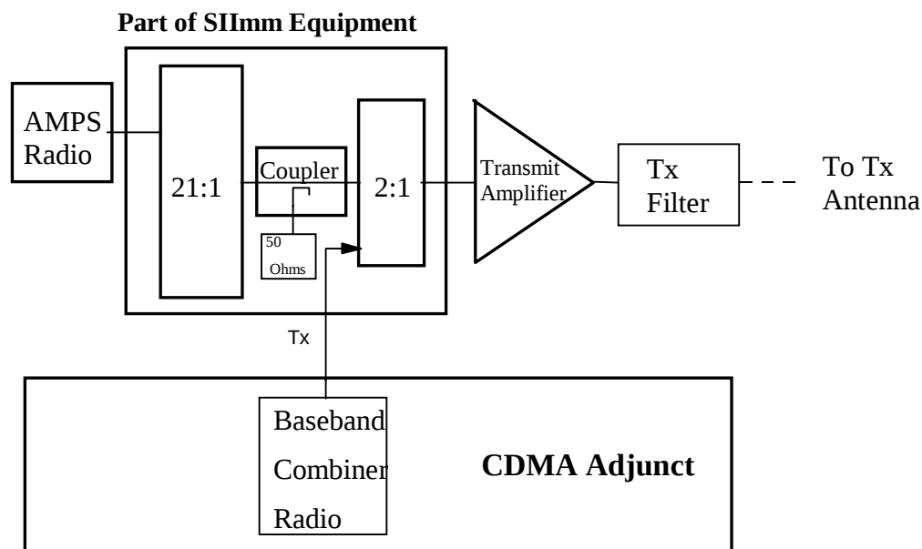
Figure 5-7. Series IImm (Microcell)/CDMA Adjunct Transmit (Tx) Path Using Series IImm (Microcell) Amplifier
