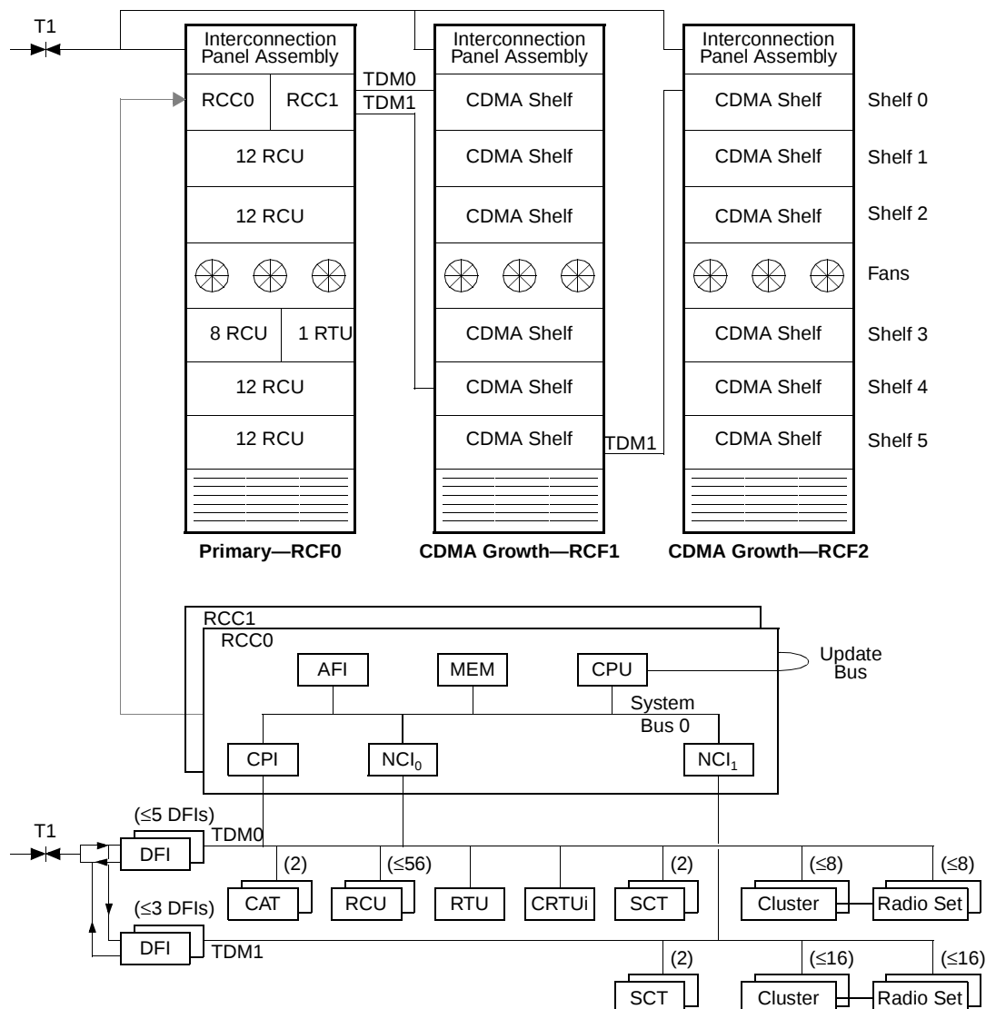
Figure 4-4. Radio Frame Set Having Two CDMA Growth RCFs (TDMs install "red stripe up")
