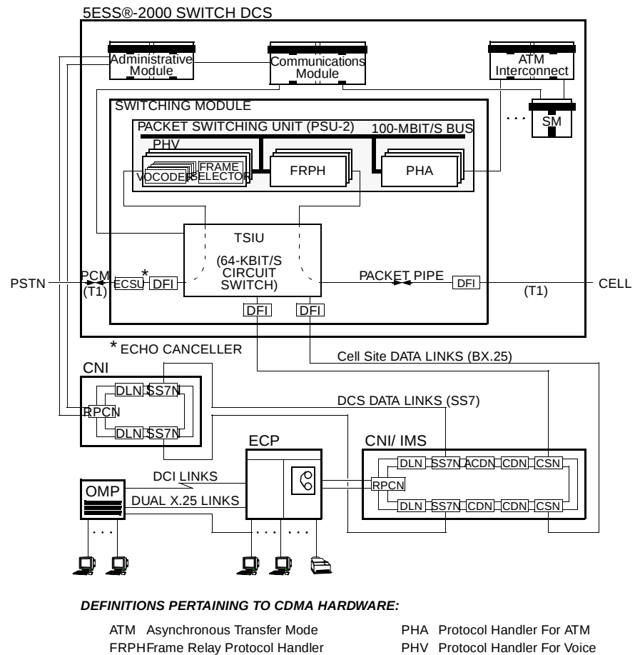
Figure 4-2. Series II Cell Site Code Division Multiple Access (CDMA) Communications Path
