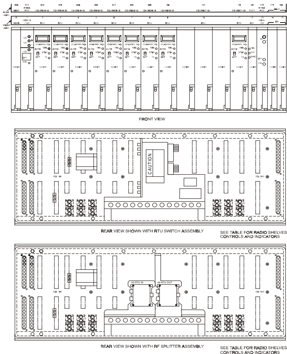
Figure 8-7. Radio Test Unit (RTU) - Shelf 3 ED-2R835-30
