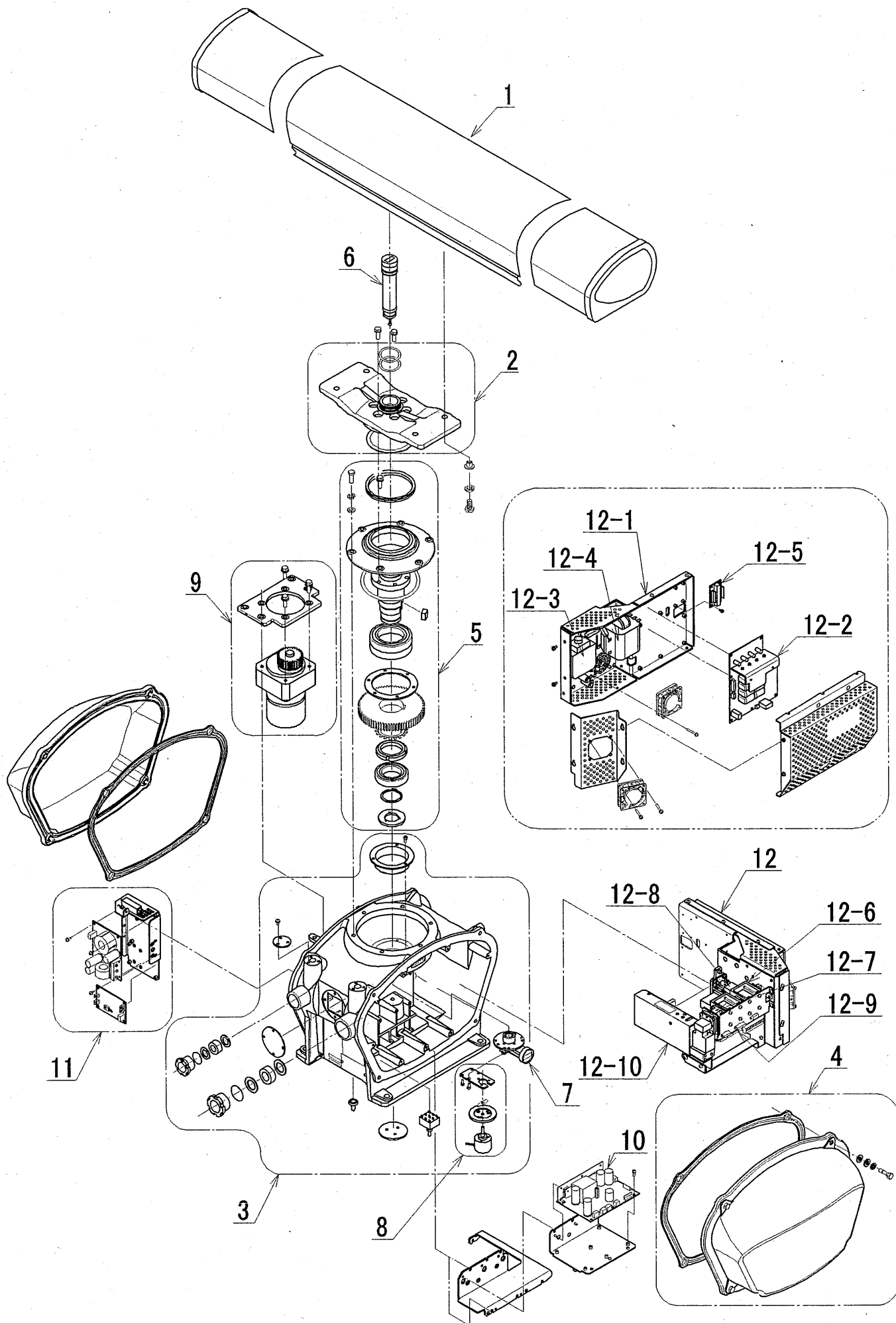
NKE-2252 SCANNER UNIT
