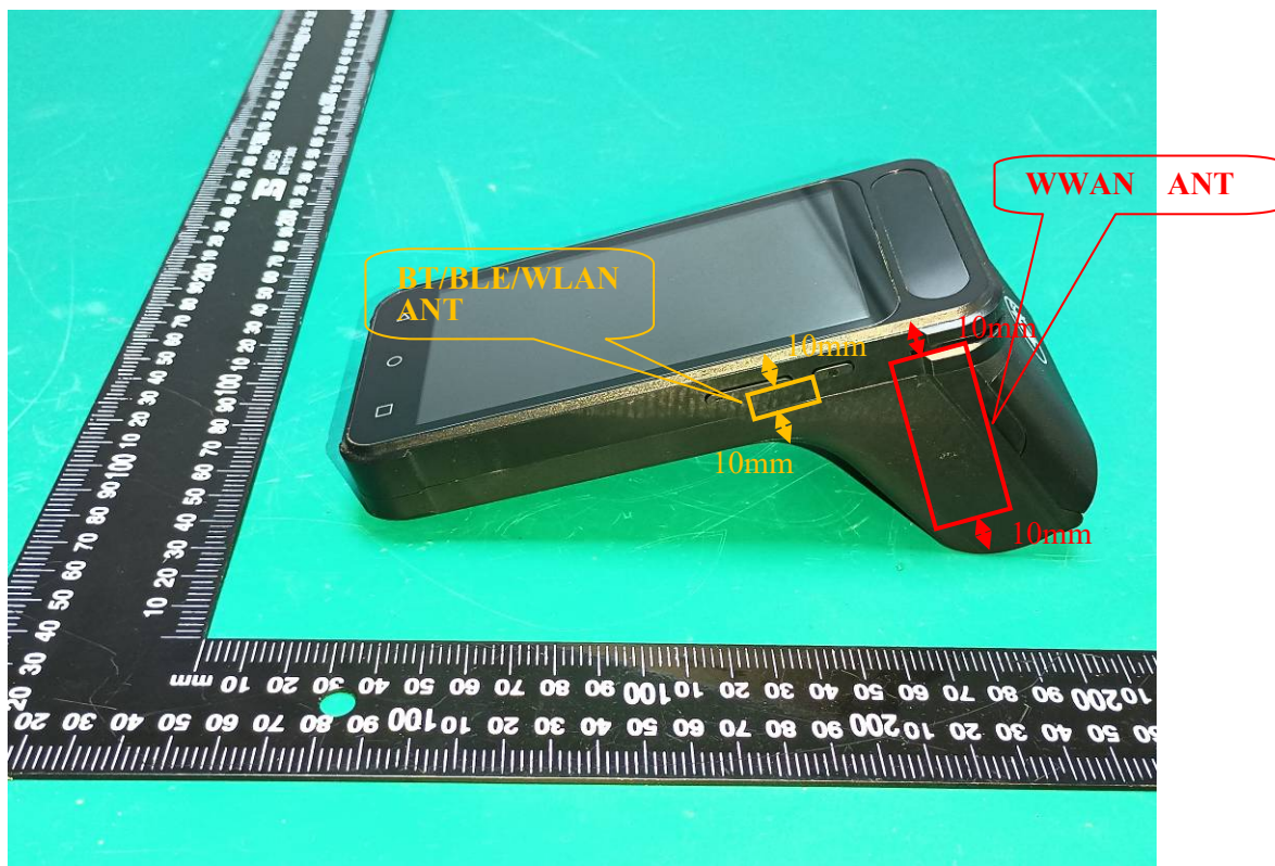
EUT Right View
