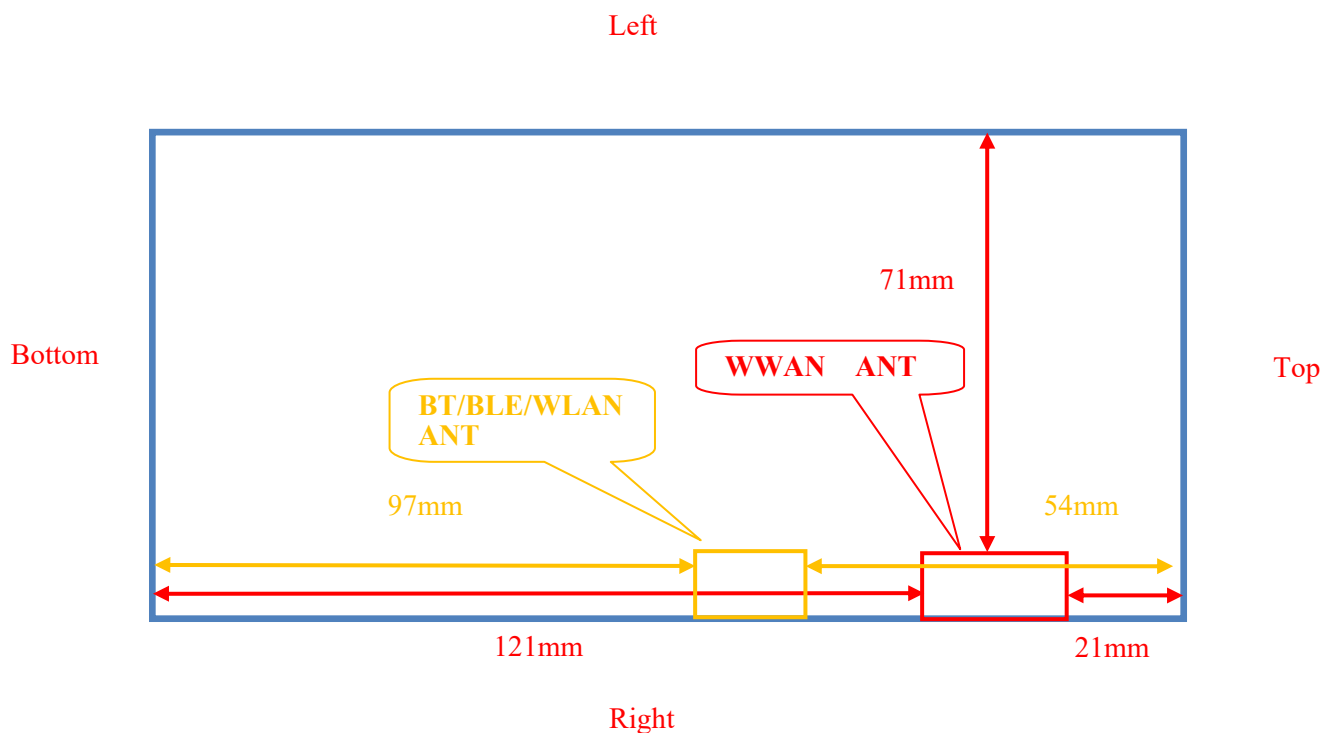
EUT Front View
