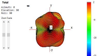
3D Antenna Pattern Plot
