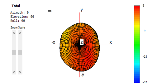
3D Antenna Pattern Plot
