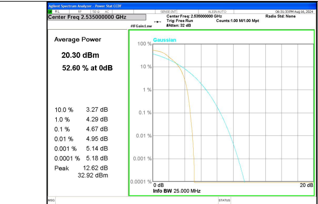
Band 7 5MHz/2535.0/Mid QPSK 25@0
