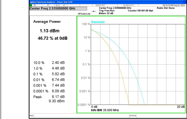
Band 7 5MHz/2535.0/Mid 16QAM 25@0
