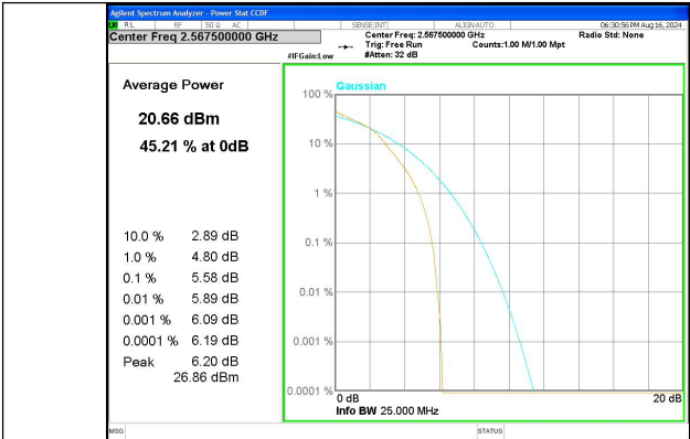
Band 7 5MHz/2567.5/High 16QAM 25@0
