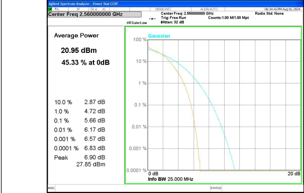
Band 7 20MHz/2560.0/High 16QAM 100@0
