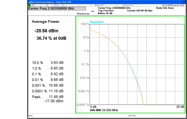
Band 7 5MHz/2502.5/Low QPSK 25@0
