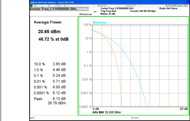
Band 7 20MHz/2510.0/Low 16QAM 100@0
