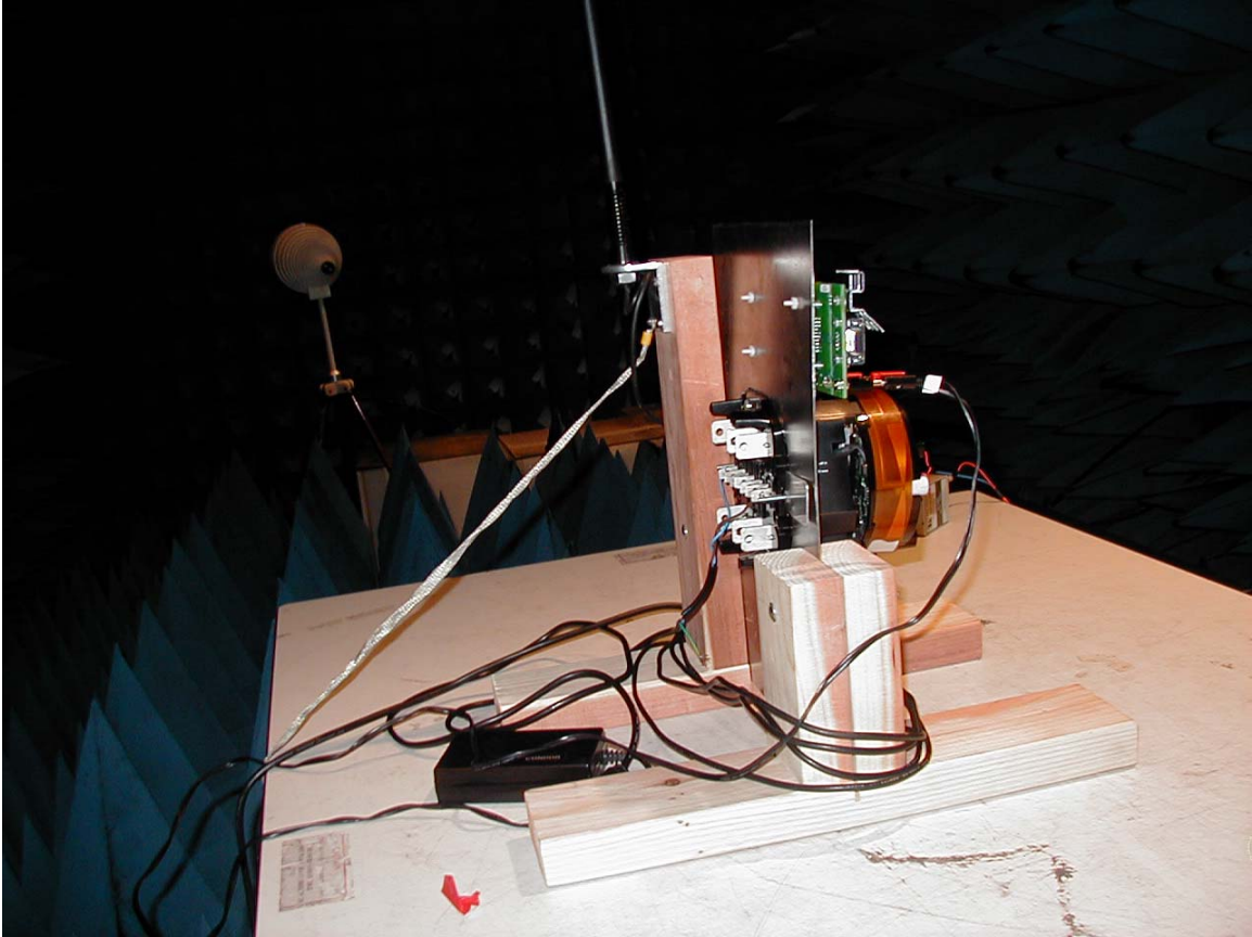
MPE Test Setup Photo# 2
