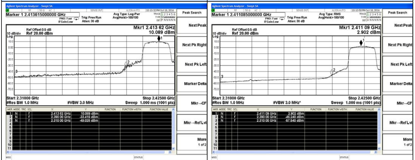
802.11n(HT20)-Low channel(Peak)
