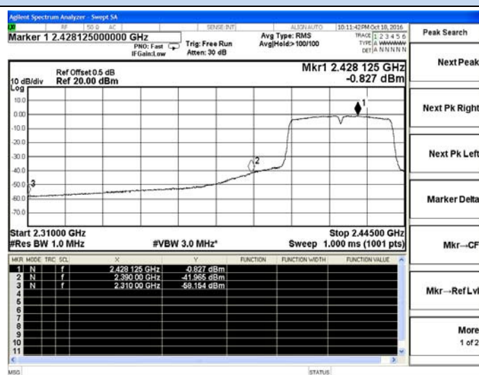
802.11n(HT40)-Low channel(Average)
