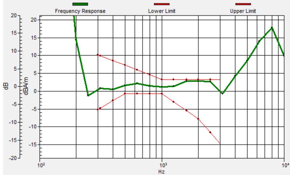
General Scans/z (axial) wideband at best S/N 2/ABM Freq Resp(x,y,z,f)
