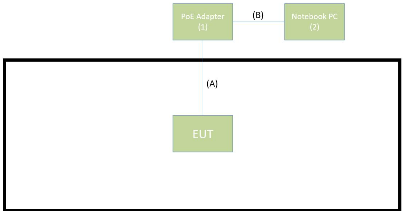
Connection Diagram
