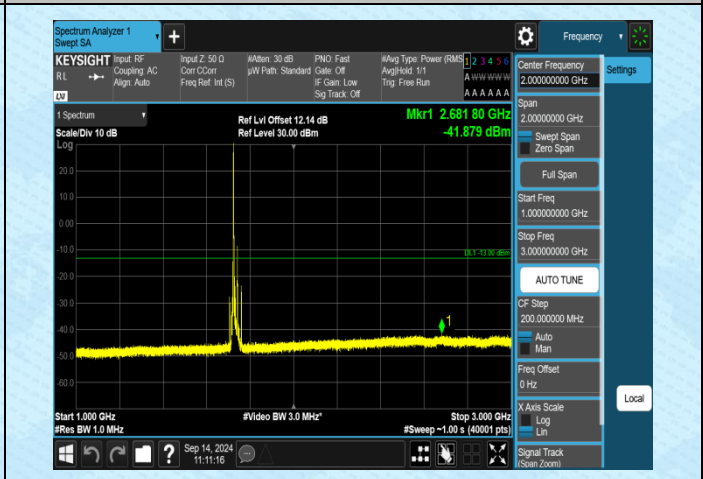
Band4-20MHz-QPSK-20175-1RB#0-1000~3000-PASS
