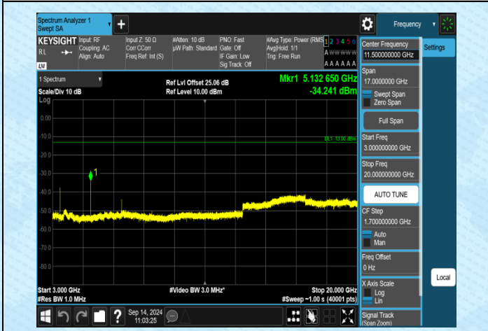
Band4-15MHz-QPSK-20025-1RB#0-3000~20000-PASS
