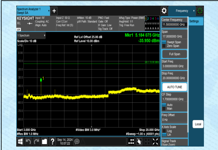
Band4-10MHz-QPSK-20175-1RB#0-3000~20000-PASS
