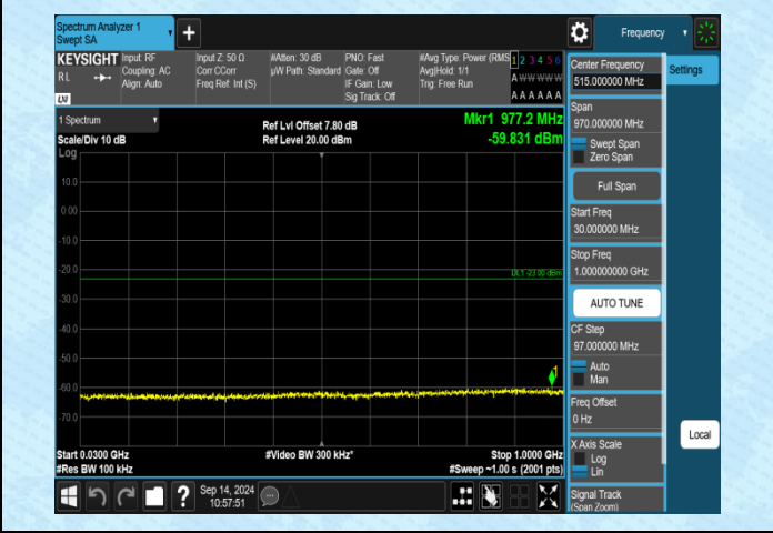
Band4-10MHz-QPSK-20350-1RB#0-30~1000-PASS
