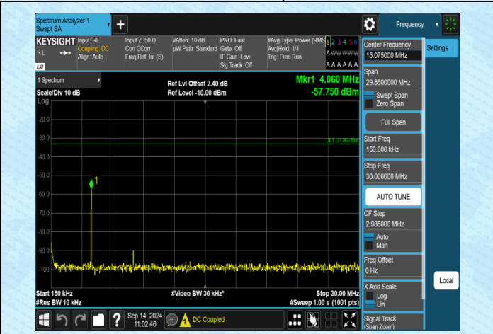
Band4-15MHz-QPSK-20025-1RB#0-0.15~30-PASS
