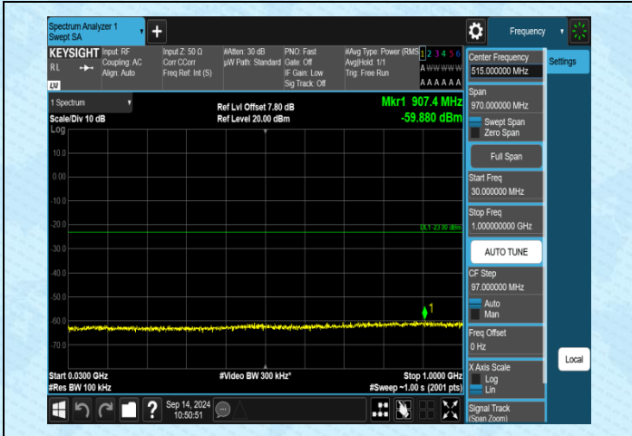
Band4-5MHz-QPSK-20375-1RB#0-30~1000-PASS
