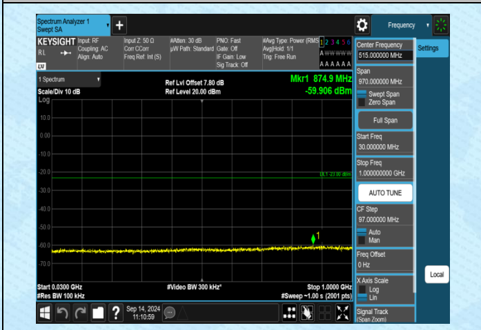
Band4-20MHz-QPSK-20175-1RB#0-30~1000-PASS
