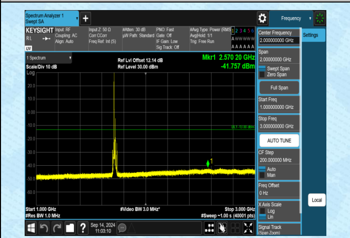
Band4-15MHz-QPSK-20025-1RB#0-1000~3000-PASS
