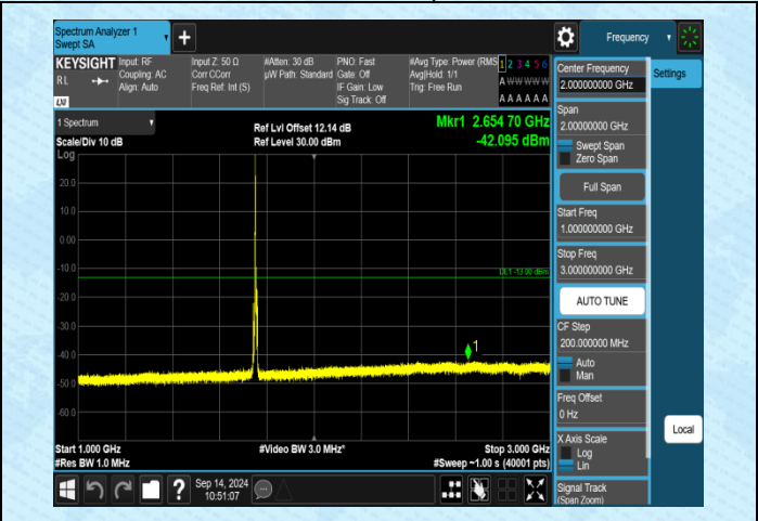
Band4-5MHz-QPSK-20375-1RB#0-1000~3000-PASS
