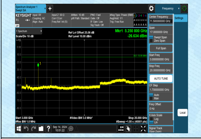
Band4-5MHz-QPSK-20375-1RB#0-3000~20000-PASS
