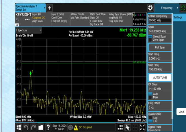
Band4-15MHz-QPSK-20325-1RB#0-0.009~0.15-PASS
