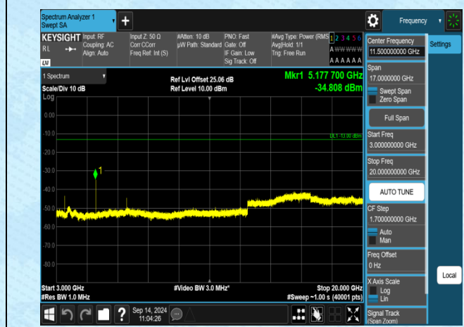
Band4-15MHz-QPSK-20175-1RB#0-3000~20000-PASS
