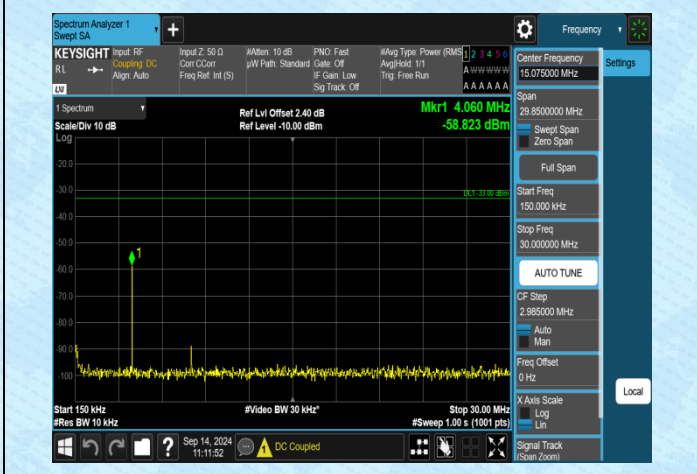
Band4-20MHz-QPSK-20300-1RB#0-0.15~30-PASS
