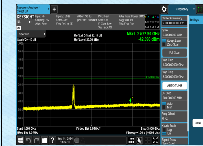
Band4-15MHz-QPSK-20175-1RB#0-1000~3000-PASS
