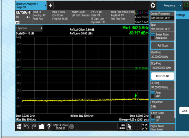
Band4-10MHz-QPSK-20175-1RB#0-30~1000-PASS
