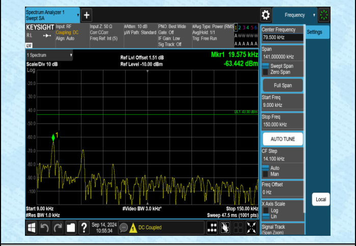
Band4-10MHz-QPSK-20000-1RB#0-0.009~0.15-PASS
