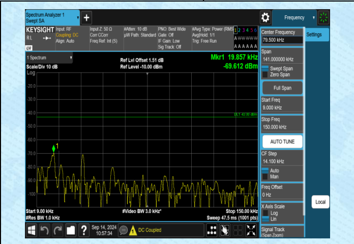
Band4-10MHz-QPSK-20350-1RB#0-0.009~0.15-PASS
