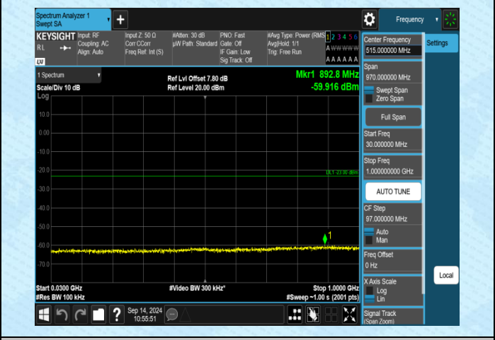
Band4-10MHz-QPSK-20000-1RB#0-30~1000-PASS
