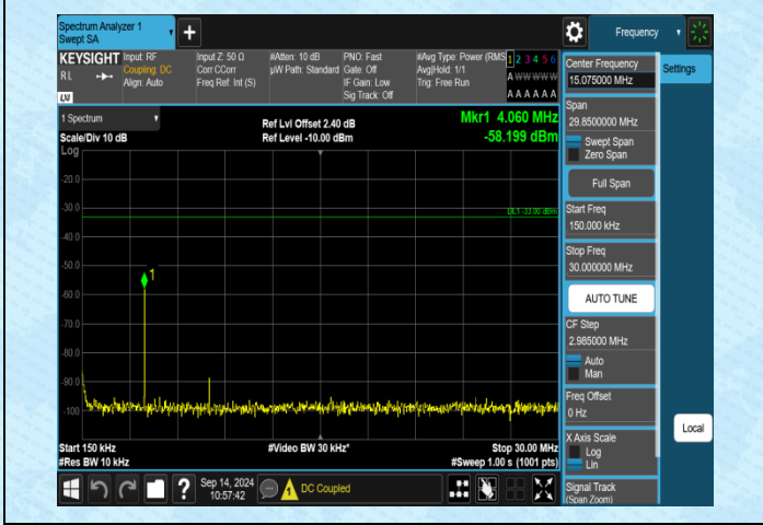
Band4-10MHz-QPSK-20350-1RB#0-0.15~30-PASS
