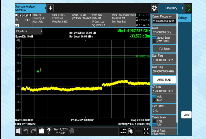
Band4-20MHz-QPSK-20300-1RB#0-3000~20000-PASS
