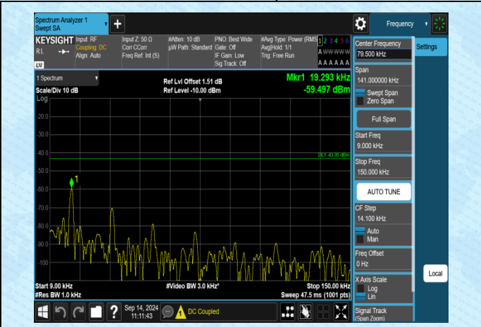
Band4-20MHz-QPSK-20300-1RB#0-0.009~0.15-PASS
