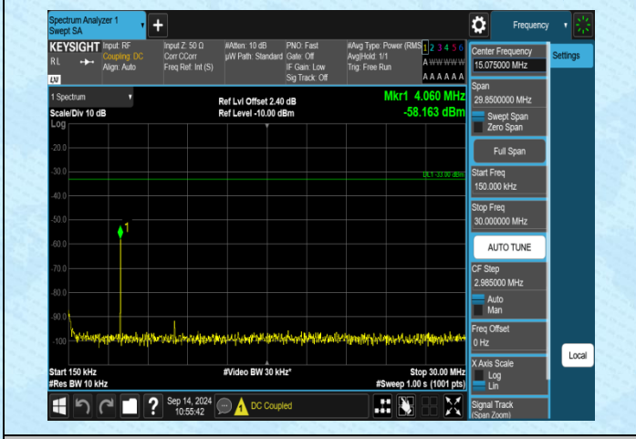
Band4-10MHz-QPSK-20000-1RB#0-0.15~30-PASS
