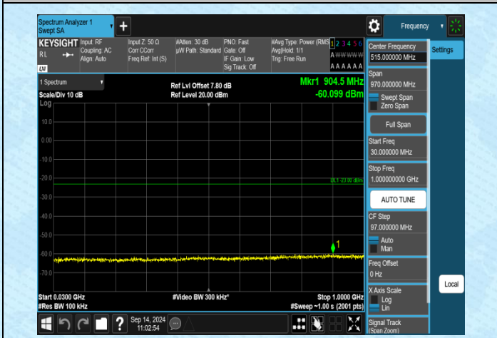
Band4-15MHz-QPSK-20025-1RB#0-30~1000-PASS
