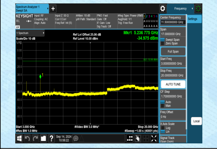
Band4-10MHz-QPSK-20350-1RB#0-3000~20000-PASS
