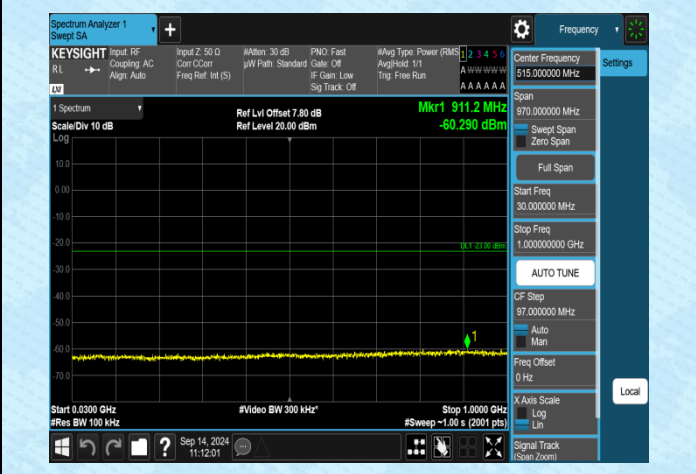
Band4-20MHz-QPSK-20300-1RB#0-30~1000-PASS
