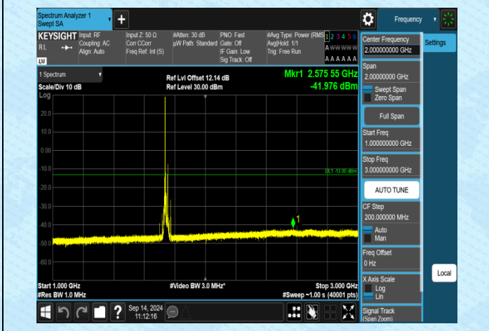
Band4-20MHz-QPSK-20300-1RB#0-1000~3000-PASS
