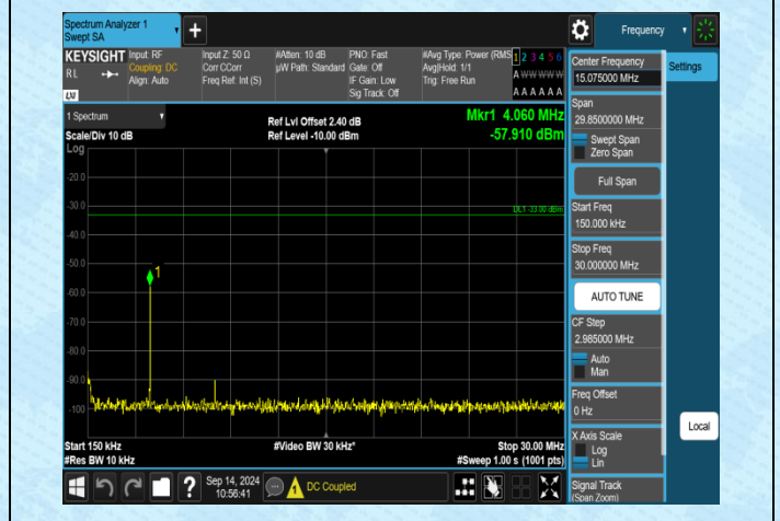
Band4-10MHz-QPSK-20175-1RB#0-0.15~30-PASS
