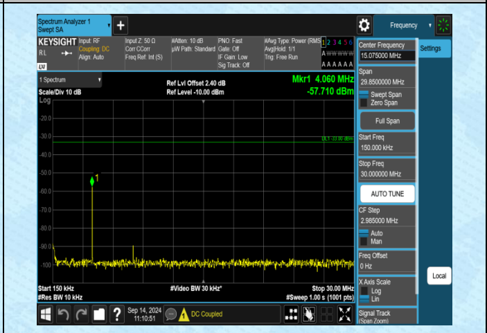
Band4-20MHz-QPSK-20175-1RB#0-0.15~30-PASS
