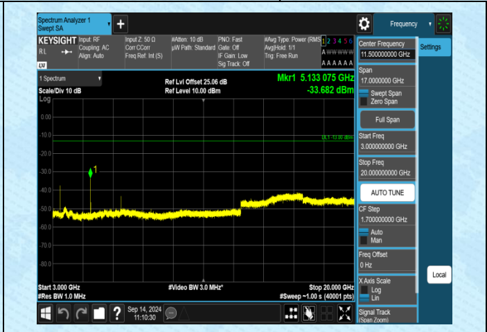
Band4-20MHz-QPSK-20050-1RB#0-3000~20000-PASS
