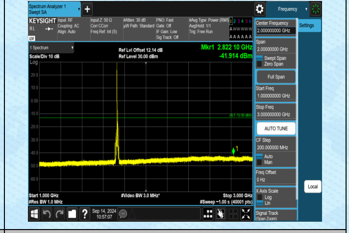
Band4-10MHz-QPSK-20175-1RB#0-1000~3000-PASS
