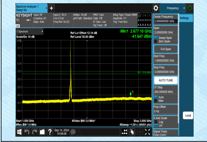
Band4-10MHz-QPSK-20350-1RB#0-1000~3000-PASS
