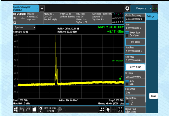
Band4-20MHz-QPSK-20050-1RB#0-1000~3000-PASS
