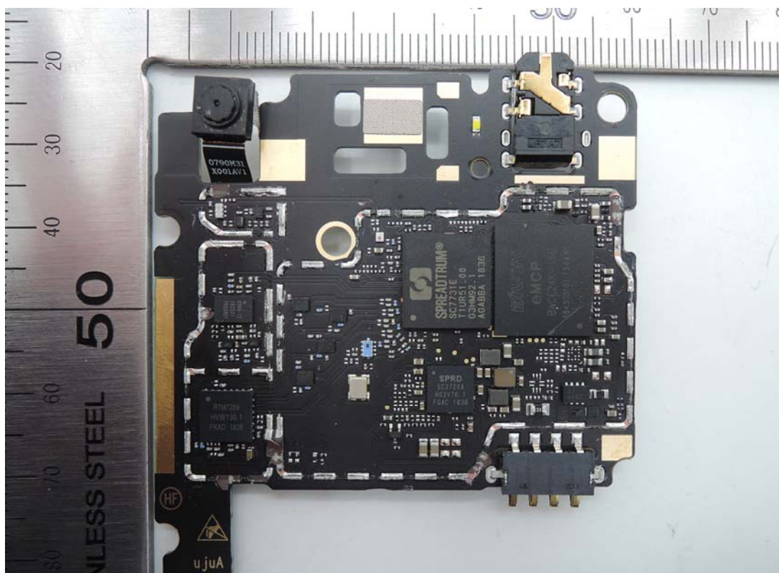
RF IC details photo 3 (front)
