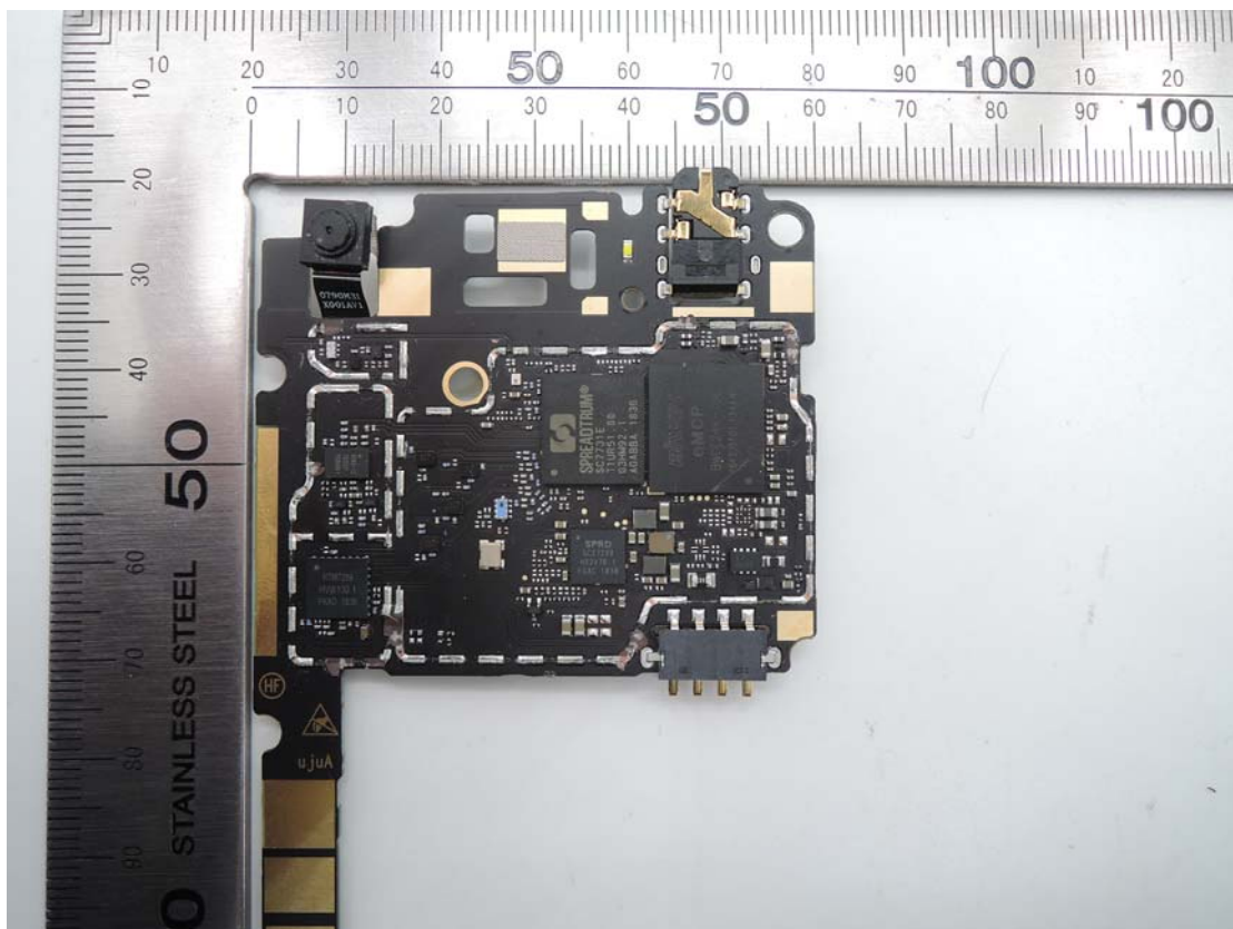
RF IC details photo 1 (front)
