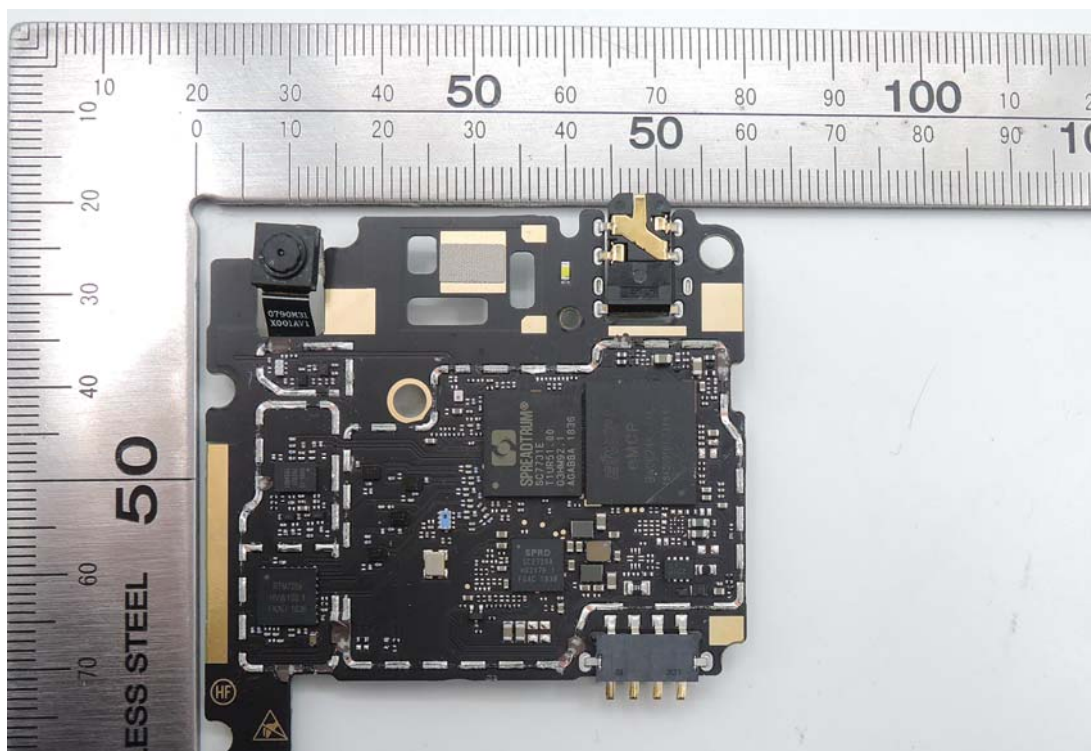
RF IC details photo 2(front)
