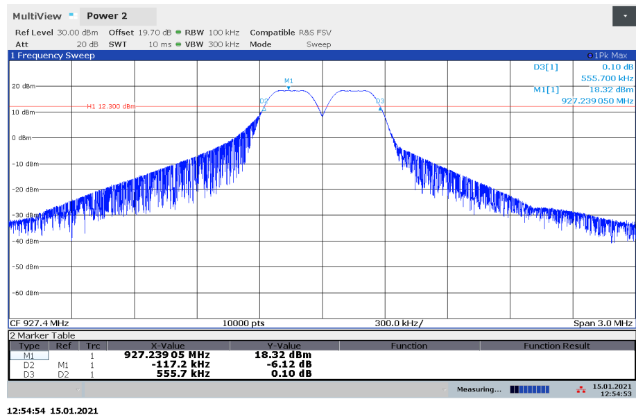
Plot 5: High Channel, 6 dB-BW
