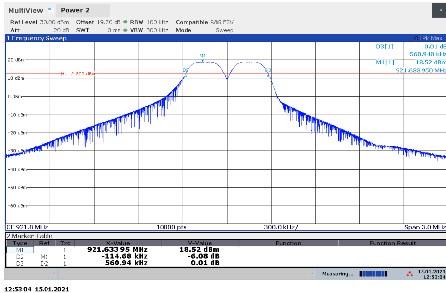
Plot 3: Middle Channel, 6 dB-BW
