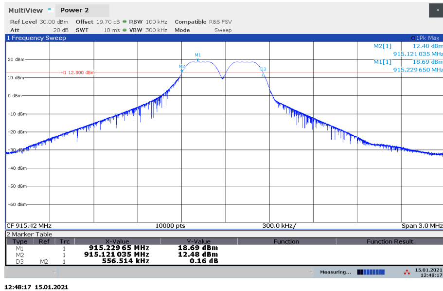
Plot 1: Low Channel, 6 dB-BW
