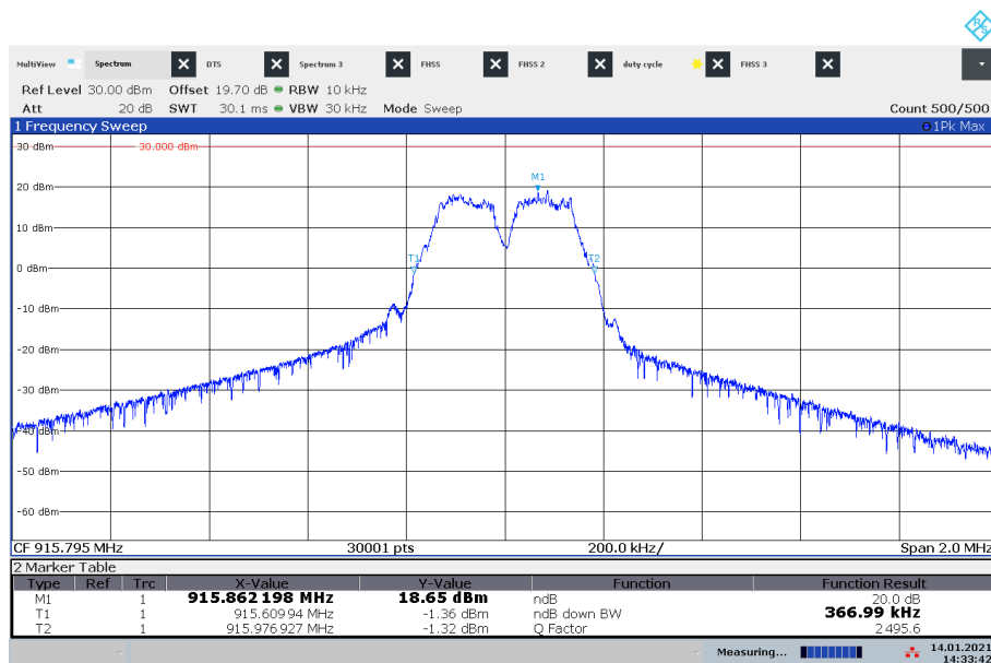
Plot 3: 915.795 MHz, 20 dB-BW
