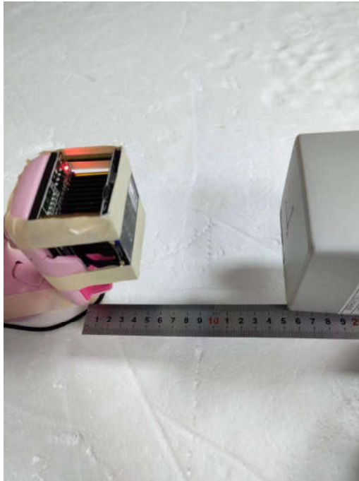
Test Setup of Front(Mode b/c/d/e)
