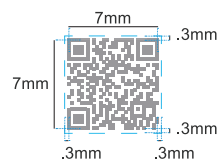
QR Code Sizing Not to Scale
