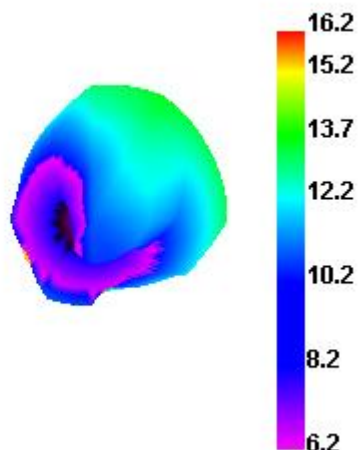
Wifi 13 TRP
