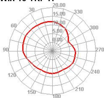
Wifi 13 TRP H
