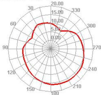
Wifi 36 TRP H
