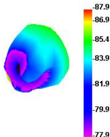
Wifi 6 TIS
