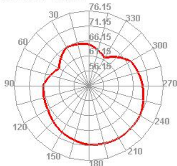
Wifi 36 TIS H
