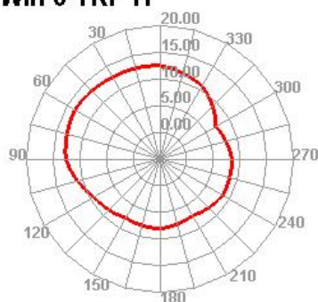
Wifi 6 TRP H
