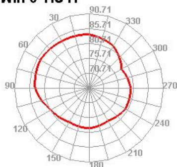
Wifi 6 TIS H
