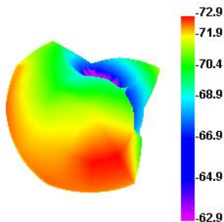
Wifi 165 TIS
