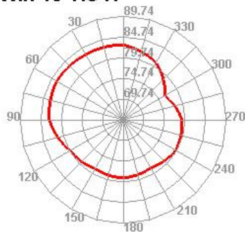
Wifi 13 TIS H
