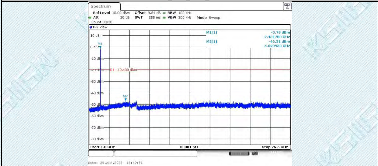
11N20SISO_Ant1_2462_1000~26500
