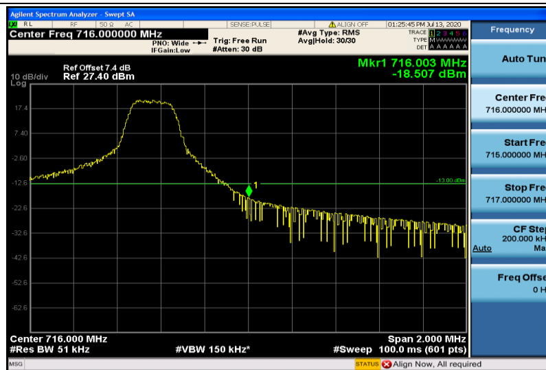
Band12-5MHz-QPSK-23155-1RB#24
