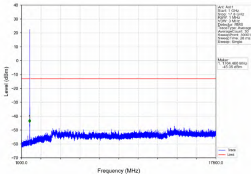
n66_15kHz_SISO_NTNV_10MHz_DFT-s-OFDM PI/2 BPSK_1745MHz_Edge_1RB_Left
