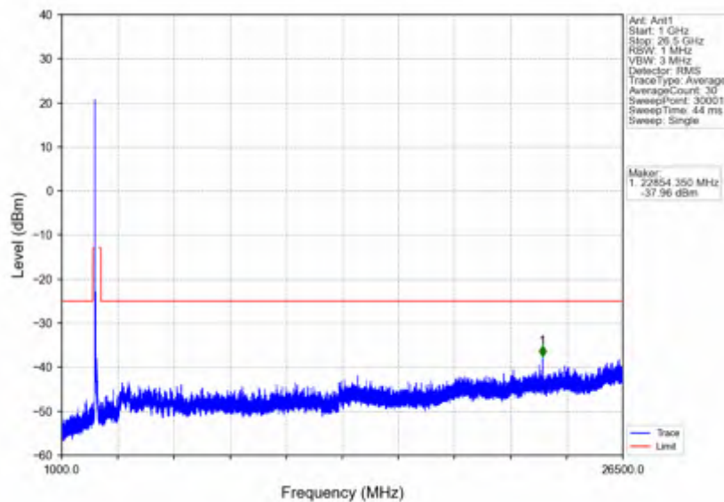
n41_30kHz_SISO_NTNV_90MHz_CP-OFDM QPSK_2541MHz_Outer_Full
