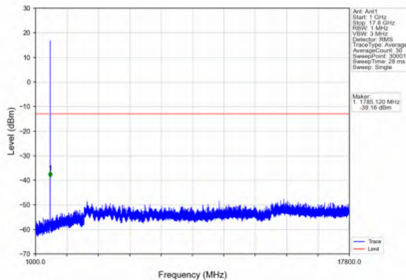
n66_15kHz_SISO_NTNV_5MHz_DFT-s-OFDM QPSK_1777.5MHz_Inner_1RB_Right
