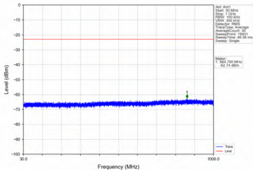
n41 30kHz SISO NTNV 100MHz CP-OFDM QPSK 2640MHz Outer Full
