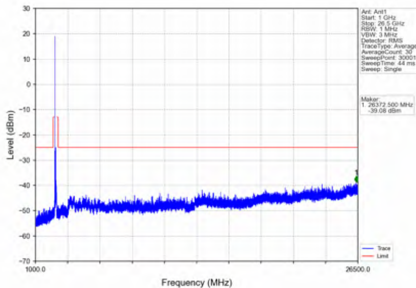
n41_30kHz_SISO_NTNV_100MHz_CP-OFDM_QPSK_2592.99MHz_Edge_1RB_Left
