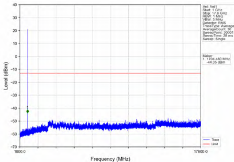
n66_15kHz_SISO_NTNV_5MHz_CP-OFDM QPSK_1745MHz_Edge_1RB_Left
