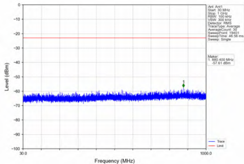
n41_30kHz_SISO_NTNV_90MHz_CP-OFDM QPSK_2644.98MHz_Edge_1RB_Right
