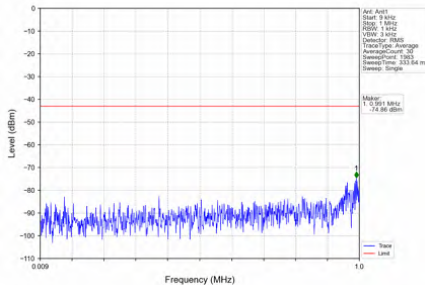
n66_15kHz_SISO_NTNV_10MHz_DFT-s-OFDM_PI/2_BPSK_1715MHz_Outer_Full
