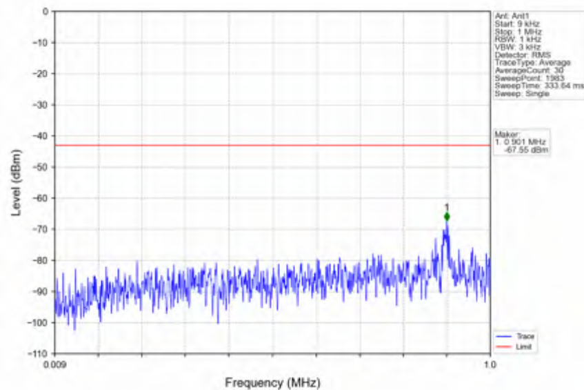
n66_15kHz_SISO_NTNV_5MHz_DFT-s-OFDM_PI/2_BPSK_1712.5MHz_Outer_Full
