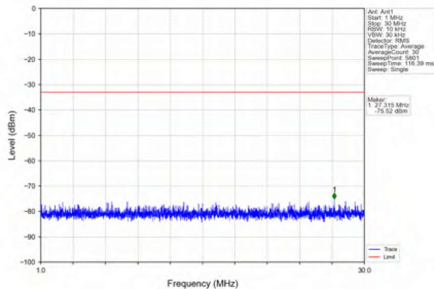
n66_15kHz_SISO_NTNV_5MHz_CP-OFDM QPSK_1777.5MHz_Inner_1RB_Right
