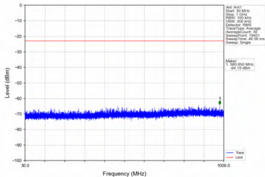
n66_15kHz_SISO_NTNV_10MHz_DFT-s-OFDM_PI/2_BPSK_1775MHz_Outer_Full
