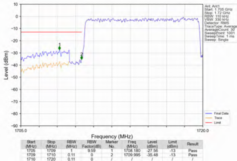
n66_15kHz_SISO_NTNV_10MHz_CP-OFDM QPSK_1715MHz_Outer_Full
