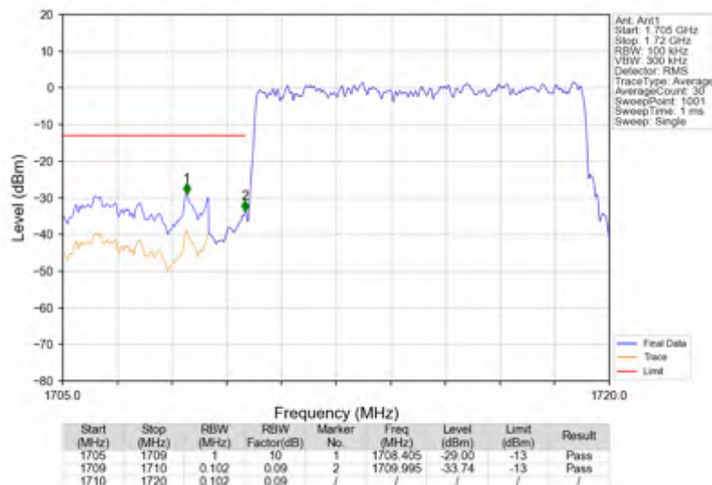
n66_15kHz_SISO_NTNV_10MHz_DFT-s-OFDM PI/2 BPSK_1715MHz_Outer_Full
