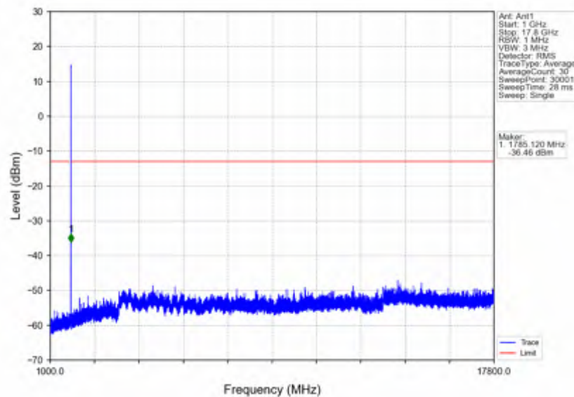
n66_15kHz_SISO_NTNV_5MHz_CP-OFDM QPSK_1777.5MHz_Outer_Full
