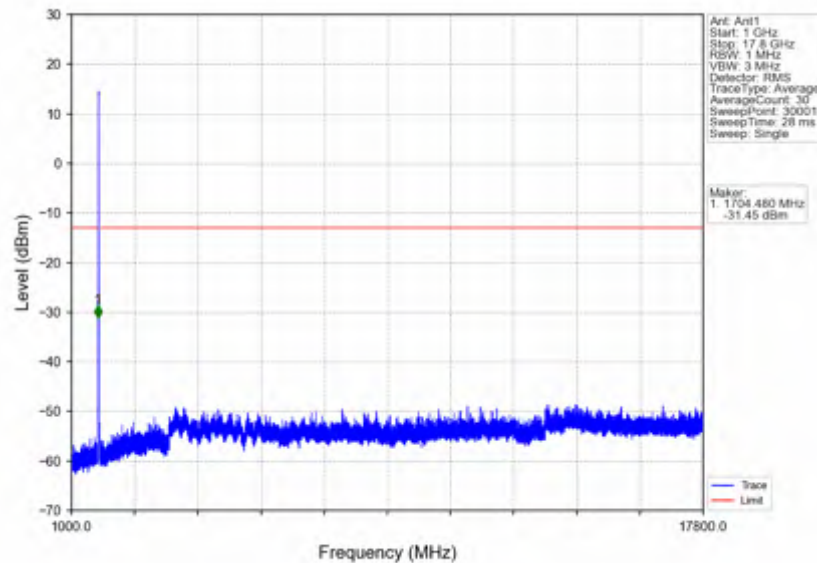
n66_15kHz_SISO_NTNV_10MHz_DFT-s-OFDM_PI/2_BPSK_1715MHz_Outer_Full
