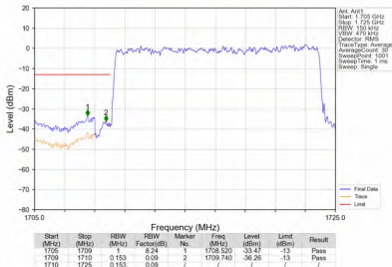
n66_15kHz_SISO_NTNV_15MHz_DFT-s-OFDM PI/2 BPSK_1717.5MHz_Outer_Full
