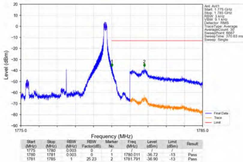
n66_15kHz_SISO_NTNV_5MHz_DFT-s-OFDM QPSK_1777.5MHz_Edge_1RB_Right
