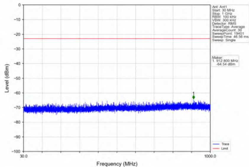
n66_15kHz_SISO_NTNV_5MHz_DFT-s-OFDM_PI/2_BPSK_1777.5MHz_Outer_Full
