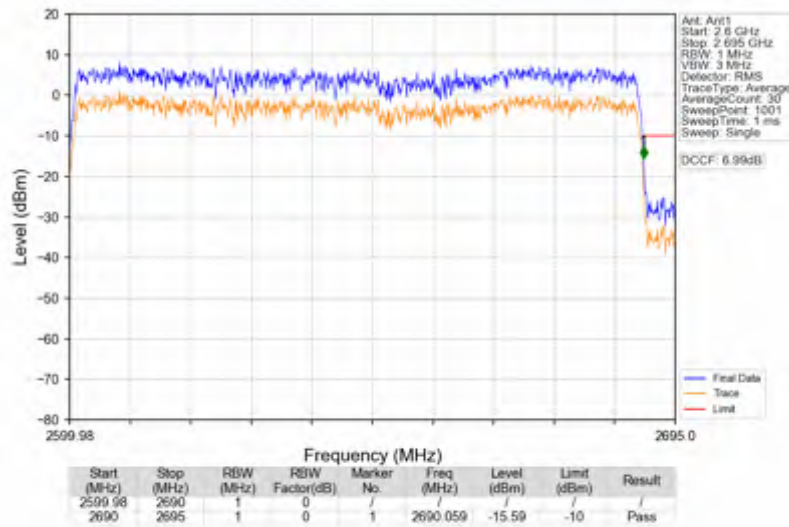
n41_30kHz_SISO_NTNV_90MHz_CP-OFDM QPSK_2644.98MHz_Outer_Full
