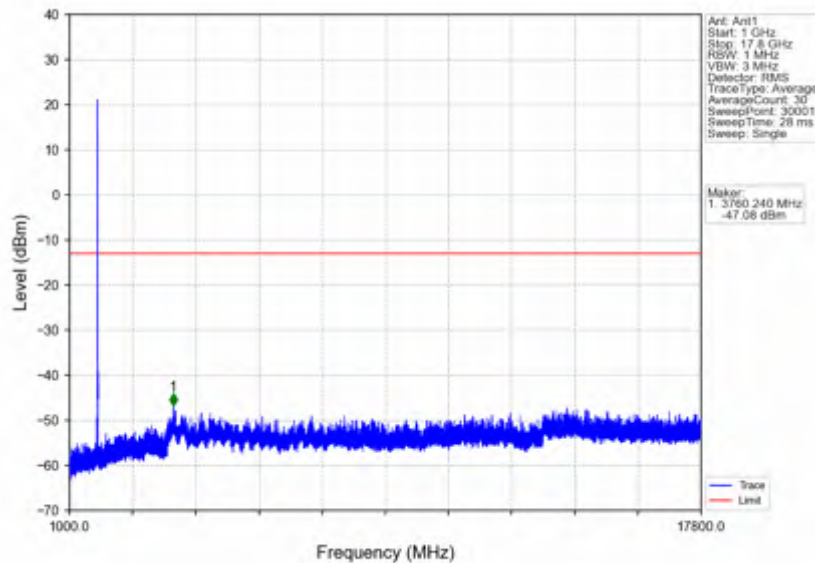
n66_15kHz_SISO_NTNV_10MHz_CP-OFDM_QPSK_1745MHz_Edge_1RB_Left
