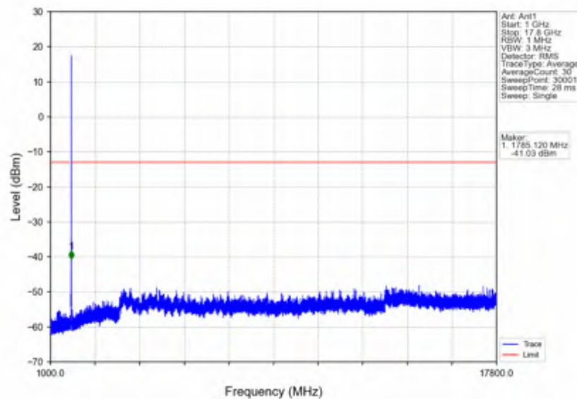
n66_15kHz_SISO_NTNV_5MHz_DFT-s-OFDM_PI/2_BPSK_1777.5MHz_Outer_Full
