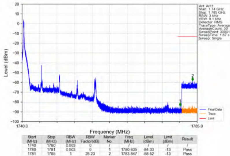
n66_15kHz_SISO_NTNV_10MHz_DFT-s-OFDM PI/2 BPSK_1745MHz_Edge_1RB_Left
