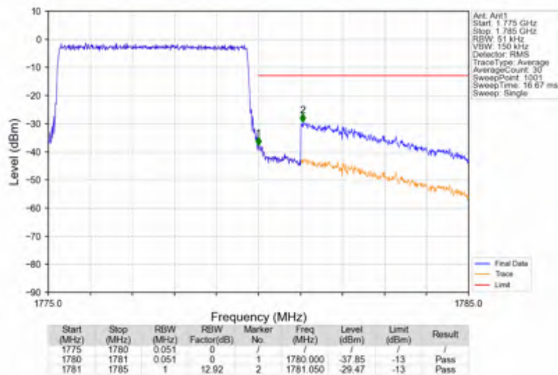
n66_15kHz_SISO_NTNV_5MHz_CP-OFDM QPSK_1777.5MHz_Outer_Full
