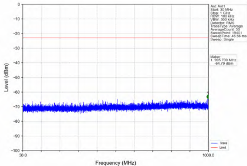
n66_15kHz_SISO_NTNV_10MHz_DFT-s-OFDM_QPSK_1775MHz_Inner_1RB_Right
