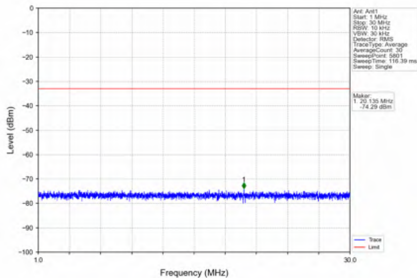
n41_30kHz_SISO_NTNV_100MHz_DFT-s-OFDM_QPSK_2546.01MHz_Edge_1RB_Left
