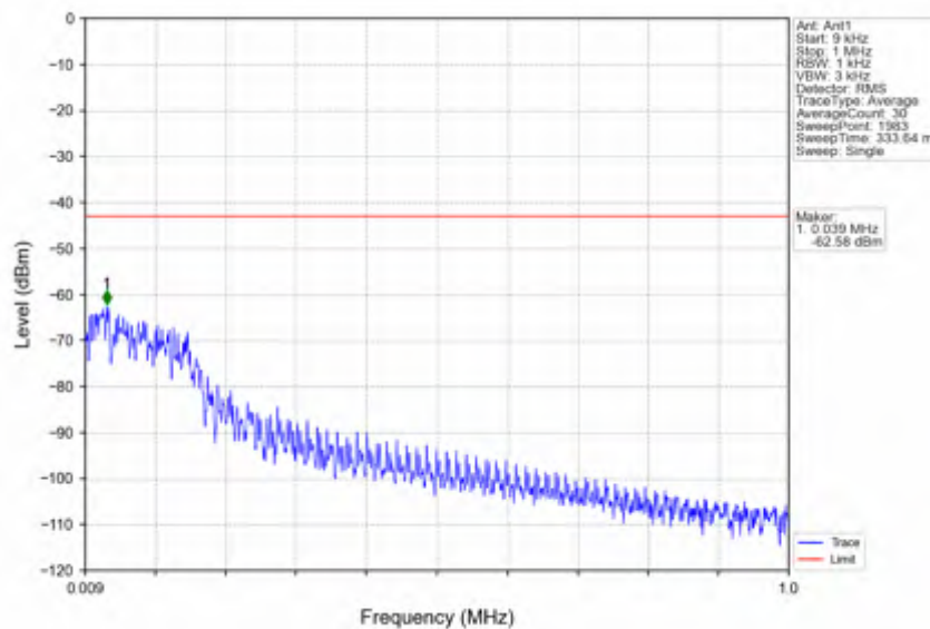
n66_15kHz_SISO_NTNV_5MHz_CP-OFDM_QPSK_1777.5MHz_Edge_1RB_Right
