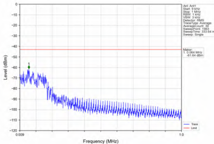
n66_15kHz_SISO_NTNV_10MHz_DFT-s-OFDM PI/2 BPSK_1775MHz_Edge_1RB_Right
