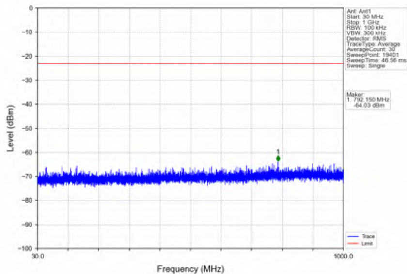
n66_15kHz_SISO_NTNV_10MHz_DFT-s-OFDM_QPSK_1715MHz_Inner_1RB_Left
