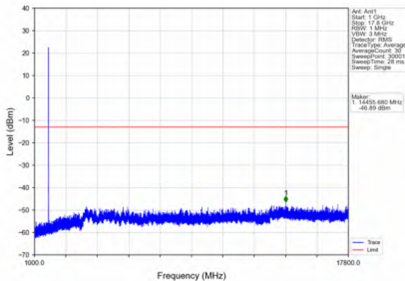
n66_15kHz_SISO_NTNV_5MHz_DFT-s-OFDM_PI/2_BPSK_1745MHz_Edge_1RB_Left
