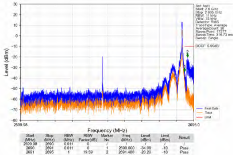
n41_30kHz_SISO_NTNV_90MHz_CP-OFDM QPSK_2644.98MHz_Inner_1RB_Right
