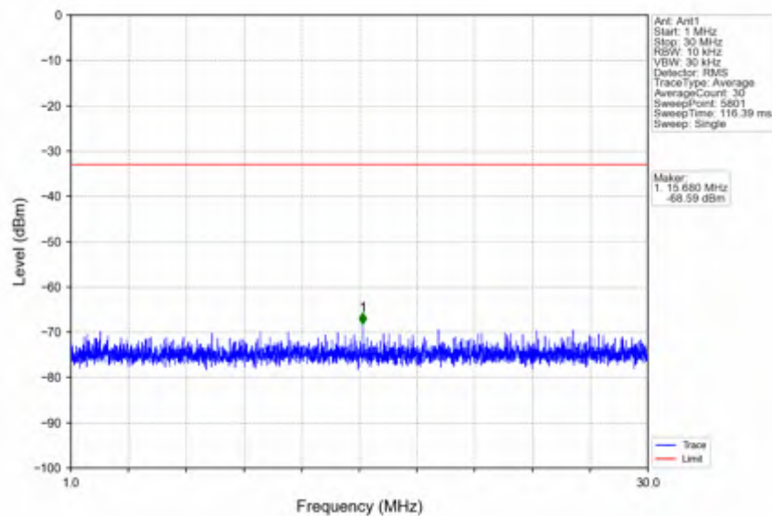
n41_30kHz_SISO_NTNV_100MHz_CP-OFDM QPSK_2546.01MHz_Edge_1RB_Left
