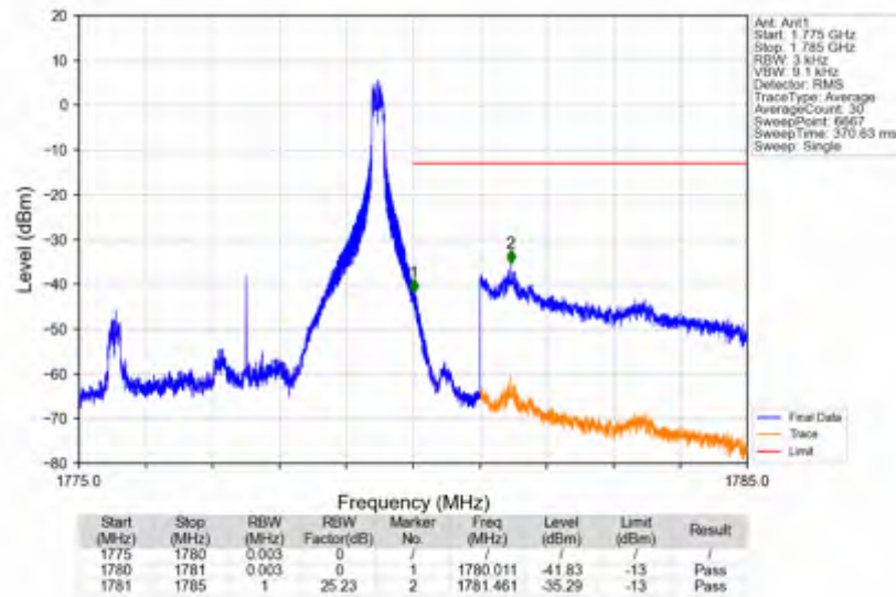
n66_15kHz_SISO_NTNV_5MHz_DFT-s-OFDM QPSK_1777.5MHz_Inner_1RB_Right
