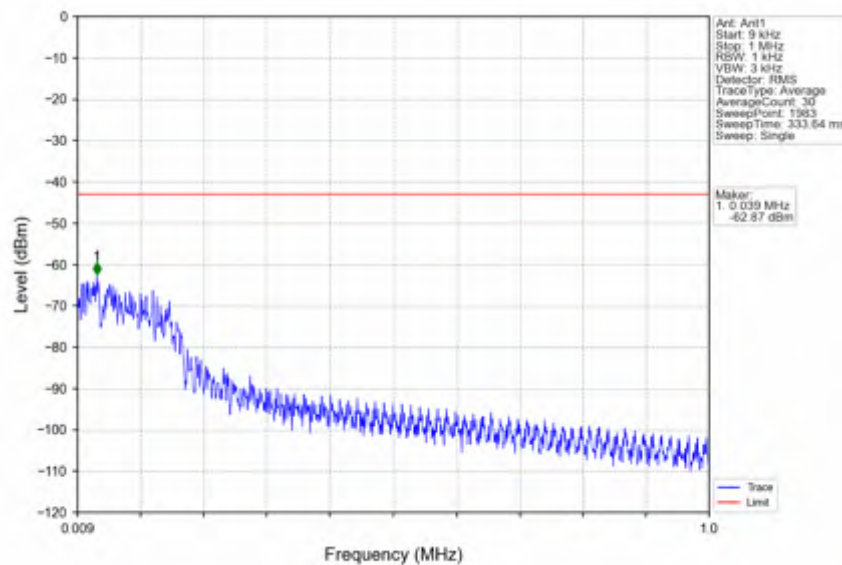
n66_15kHz_SISO_NTNV_10MHz_CP-OFDM_QPSK_1745MHz_Edge_1RB_Left
