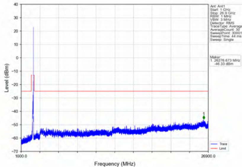
n41_30kHz_SISO_NTNV_100MHz_DFT-s-OFDM_QPSK_2640MHz_Inner_1RB_Right
