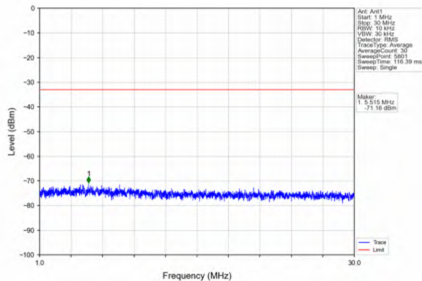
n41_30kHz_SISO_NTNV_100MHz_DFT-s-OFDM QPSK_2546.01MHz_Outer_Full
