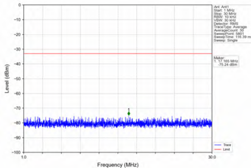
n66_15kHz_SISO_NTNV_10MHz_DFT-s-OFDM QPSK_1745MHz_Edge_1RB_Left
