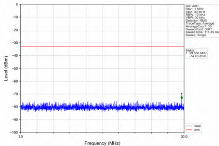
n66_15kHz_SISO_NTNV_5MHz_DFT-s-OFDM QPSK_1745MHz_Edge_1RB_Left
