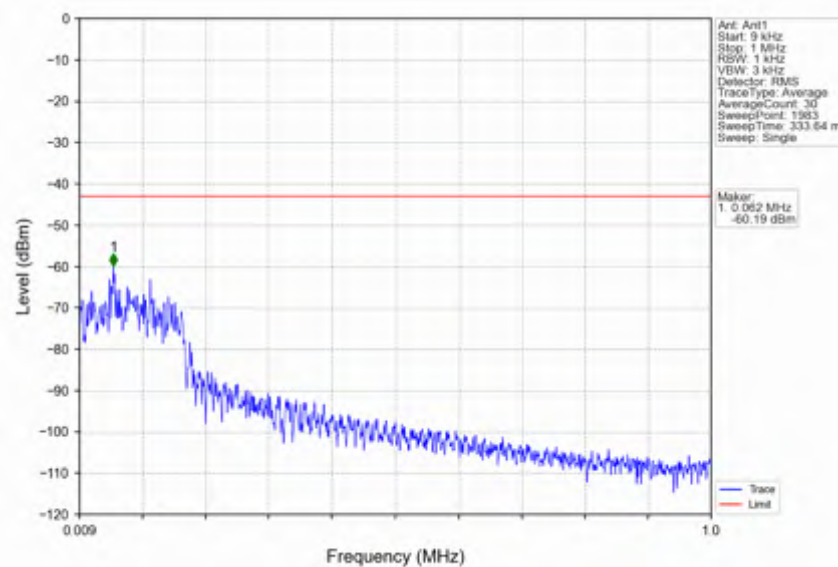
n66_15kHz_SISO_NTV_5MHz_DFT-s-OFDM QPSK_1745MHz_Edge_1RB_Left
