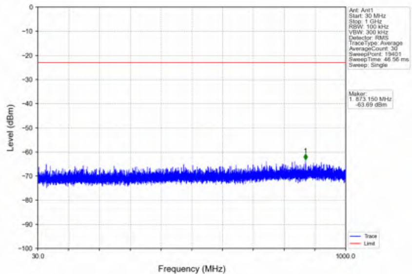
n66_15kHz_SISO_NTNV_5MHz_CP-OFDM QPSK_1712.5MHz_Edge_1RB_Left
