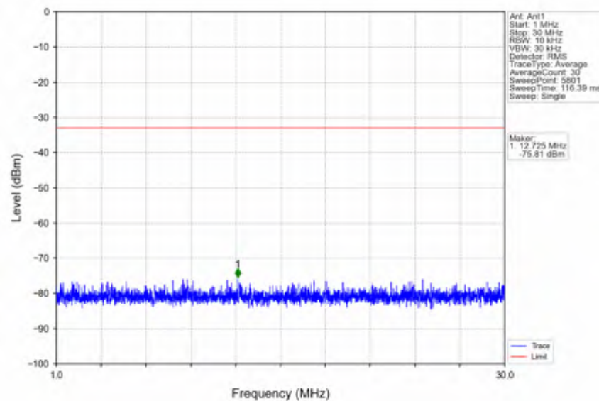
n66_15kHz_SISO_NTNV_5MHz_DFT-s-OFDM QPSK_1712.5MHz_Outer_Full
