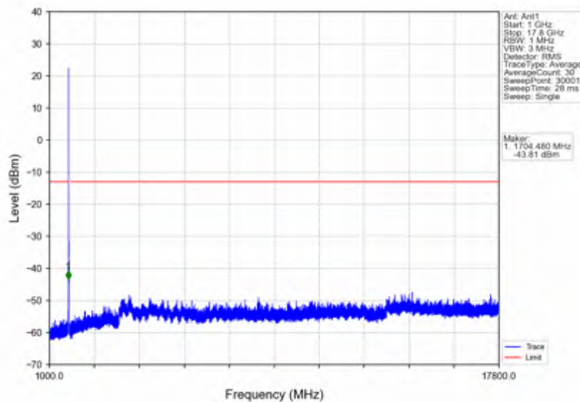
n66_15kHz_SISO_NTNV_10MHz_DFT-s-OFDM_QPSK_1715MHz_Inner_1RB_Left
