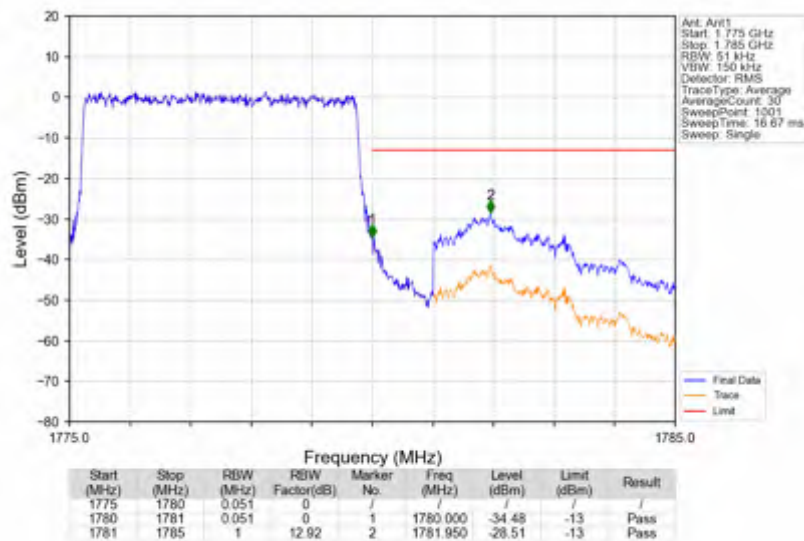
n66_15kHz_SISO_NTNV_5MHz_DFT-s-OFDM PI/2 BPSK_1777.5MHz_Outer_Full
