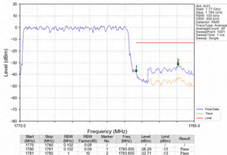
n66_15kHz_SISO_NTNV_10MHz_DFT-s-OFDM PI/2 BPSK_1775MHz_Outer_Full
