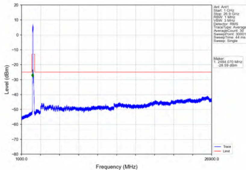
n41 30kHz SISO NTV 90MHz CP-OFDM QPSK 2541MHz Outer Full
