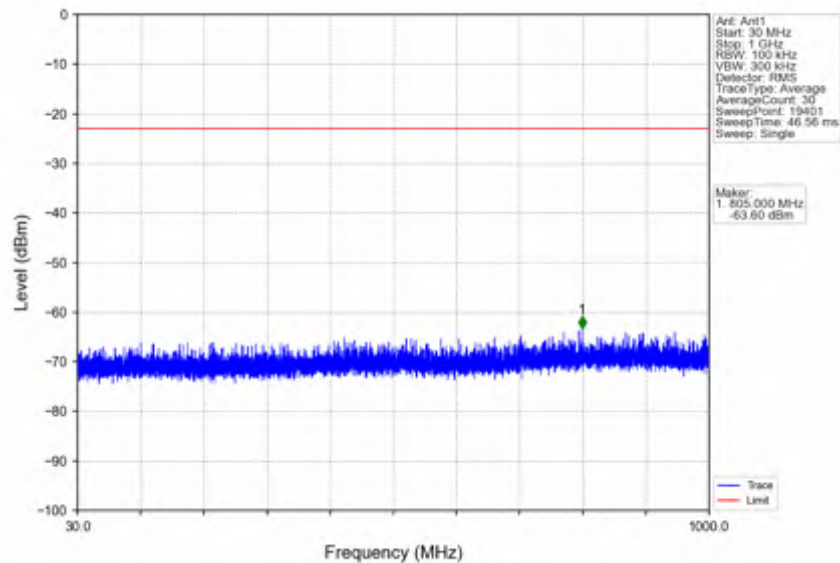
n66_15kHz_SISO_NTNV_10MHz_CP-OFDM_QPSK_1745MHz_Edge_1RB_Left
