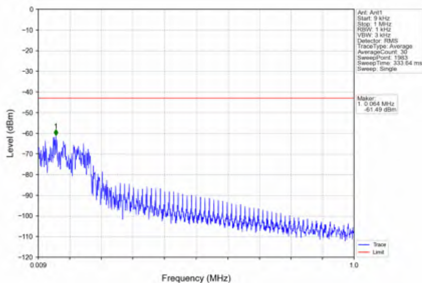
n66_15kHz_SISO_NTNV_5MHz_DFT-s-OFDM_PI/2_BPSK_1712.5MHz_Edge_1RB_Left
