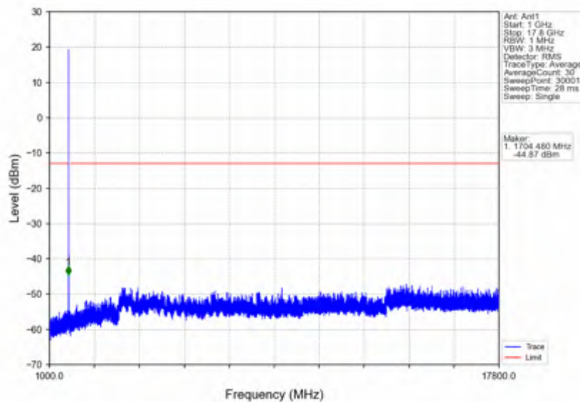
n66_15kHz_SISO_NTNV_5MHz_CP-OFDM QPSK_1712.5MHz_Outer_Full
