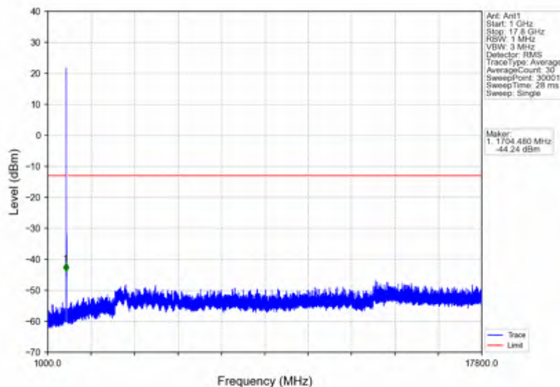
n66_15kHz_SISO_NTNV_10MHz_DFT-s-OFDM PI/2 BPSK_1715MHz_Outer_Full
