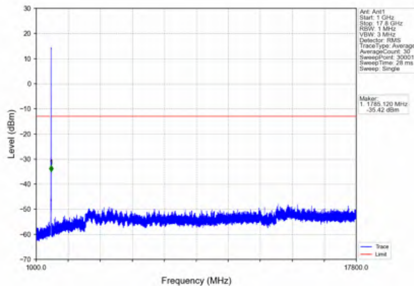
n66_15kHz_SISO_NTNV_10MHz_DFT-s-OFDM_PI/2_BPSK_1775MHz_Outer_Full
