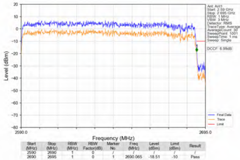
n41_30kHz_SISO_NTNV_100MHz_CP-OFDM QPSK_2640MHz_Outer_Full
