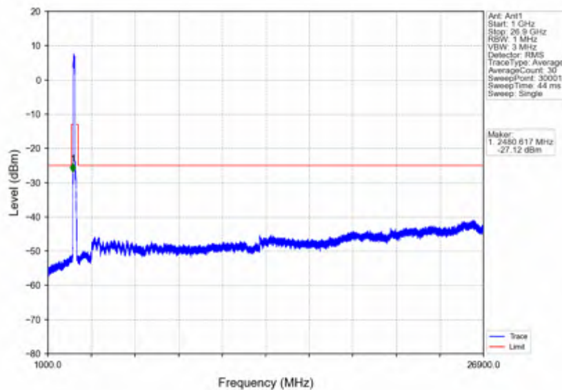
n41_30kHz_SISO_NTNV_100MHz_DFT-s-OFDM QPSK_2546.01MHz_Inner_1RB_Left
