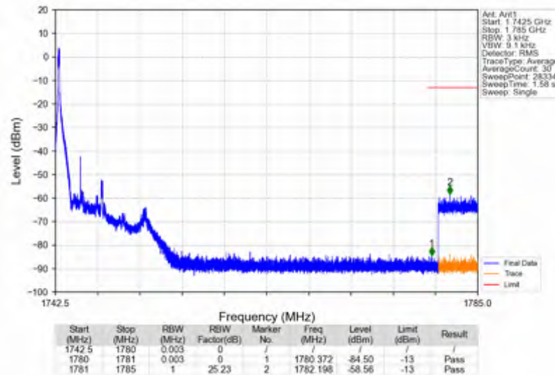
n66_15kHz_SISO_NTV_5MHz_DFT-s-OFDM QPSK_1745MHz_Edge_1RB_Left
