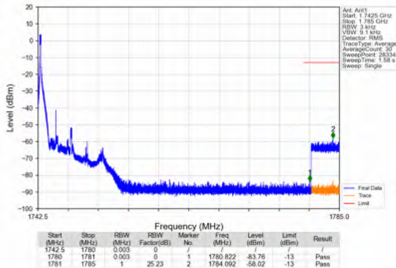
n66_15kHz_SISO_NTNV_5MHz_DFT-s-OFDM PI/2 BPSK_1745MHz_Edge_1RB_Left
