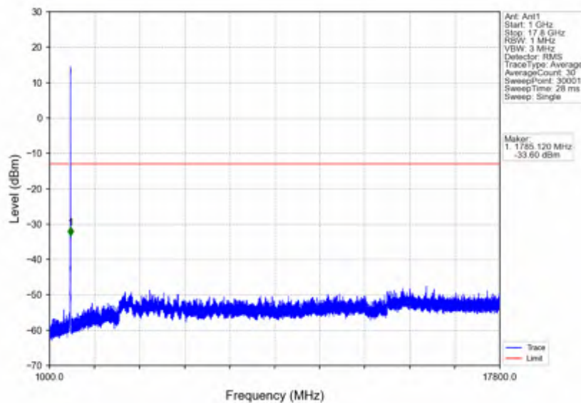
n66_15kHz_SISO_NTNV_10MHz_DFT-s-OFDM QPSK_1775MHz_Inner_1RB_Right
