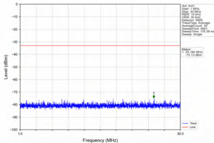
n66_15kHz_SISO_NTNV_5MHz_DFT-s-OFDM QPSK_1777.5MHz_Outer_Full
