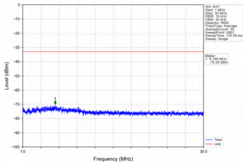
n41_30kHz_SISO_NTNV_90MHz_CP-OFDM QPSK_2541MHz_Outer_Full
