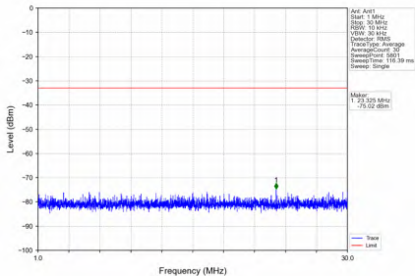
n66_15kHz_SISO_NTNV_10MHz_CP-OFDM QPSK_1775MHz_Outer_Full
