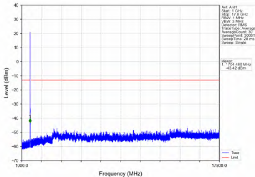
n66_15kHz_SISO_NTNV_10MHz_CP-OFDM QPSK_1715MHz_Outer_Full
