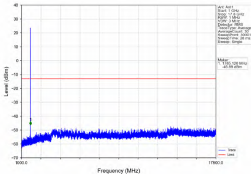
n66_15kHz_SISO_NTNV_5MHz_DFT-s-OFDM PI/2 BPSK_1777.5MHz_Outer_Full
