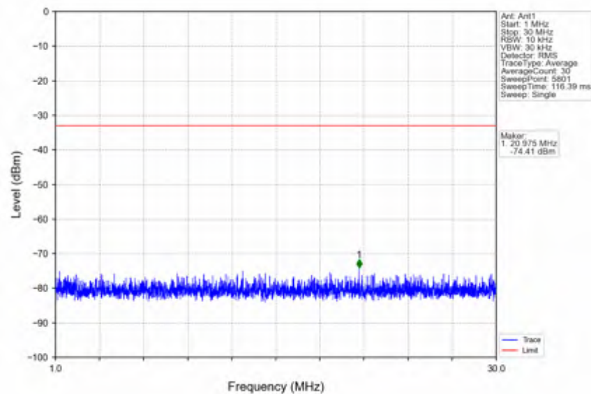
n66_15kHz_SISO_NTNV_10MHz_DFT-s-OFDM QPSK_1715MHz_Edge_1RB_Left
