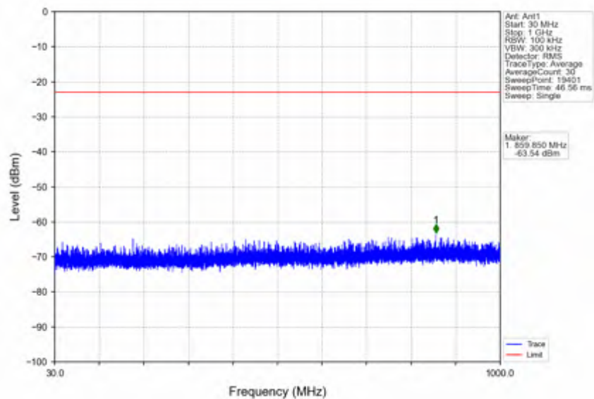
n66_15kHz_SISO_NTNV_5MHz_CP-OFDM_QPSK_1777.5MHz_Edge_1RB_Right
