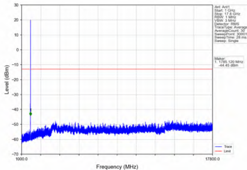
n66_15kHz_SISO_NTNV_10MHz_CP-OFDM QPSK_1775MHz_Outer_Full
