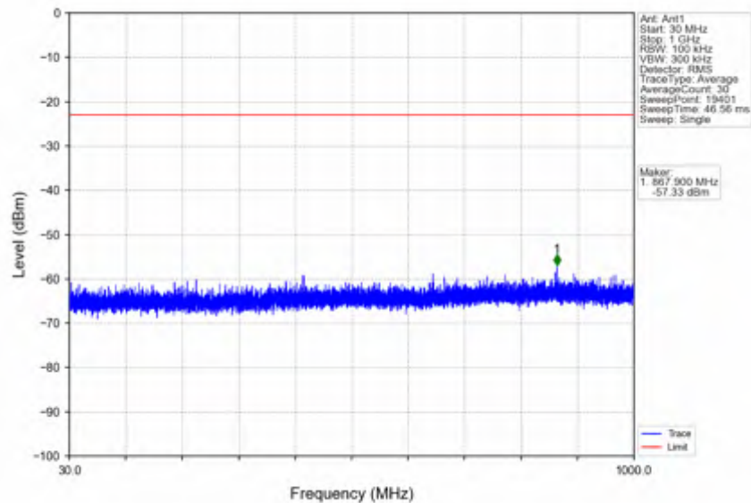
n41_30kHz_SISO_NTNV_100MHz_DFT-s-OFDM QPSK_2640MHz_Edge_1RB_Right
