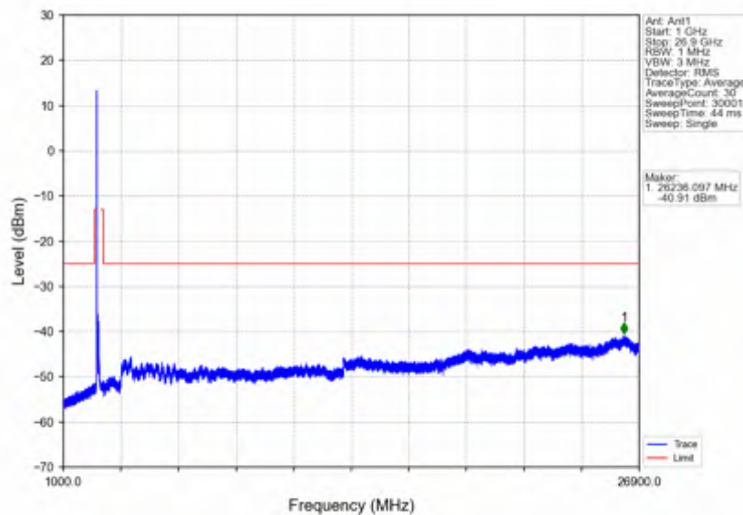
n41_30kHz_SISO_NTNV_100MHz_DFT-s-OFDM_QPSK_2546.01MHz_Edge_1RB_Left
