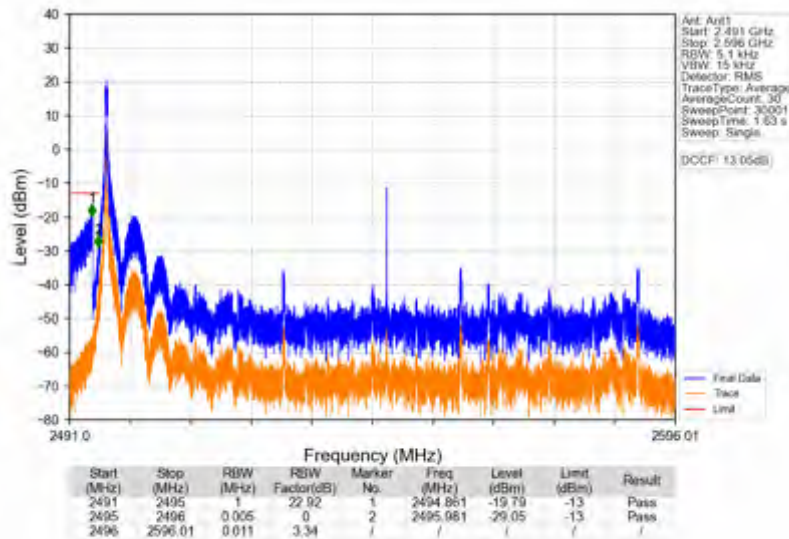
n41_30kHz_SISO_NTNV_100MHz_DFT-s-OFDM QPSK_2546.01MHz_Inner_1RB_Left
