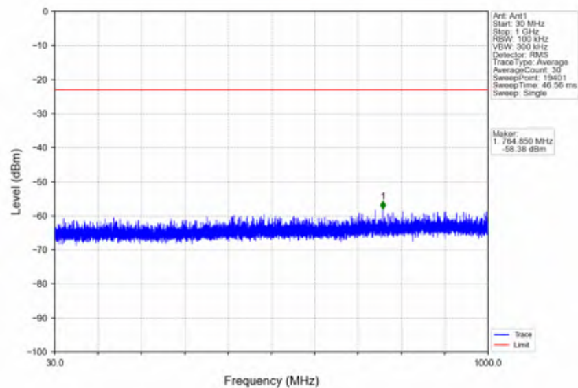
n41_30kHz_SISO_NTNV_90MHz_CP-OFDM QPSK_2592.99MHz_Edge_1RB_Left
