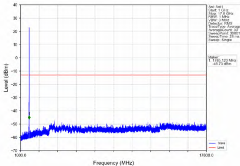
n66_15kHz_SISO_NTNV_10MHz_DFT-s-OFDM QPSK_1715MHz_Edge_1RB_Left
