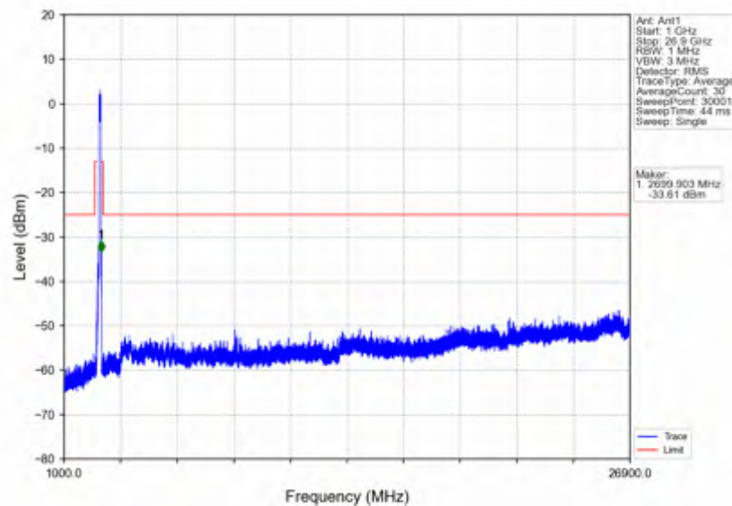
n41_30kHz_SISO_NTNV_90MHz_CP-OFDM QPSK_2644.98MHz_Outer_Full
