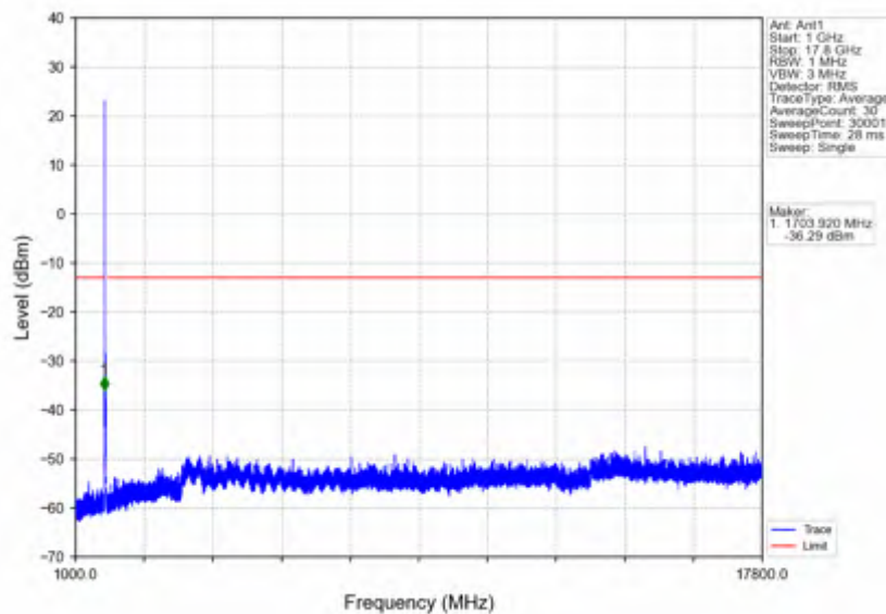
n66_15kHz_SISO_NTNV_15MHz_DFT-s-OFDM PI/2 BPSK_1745MHz_Edge_1RB_Left
