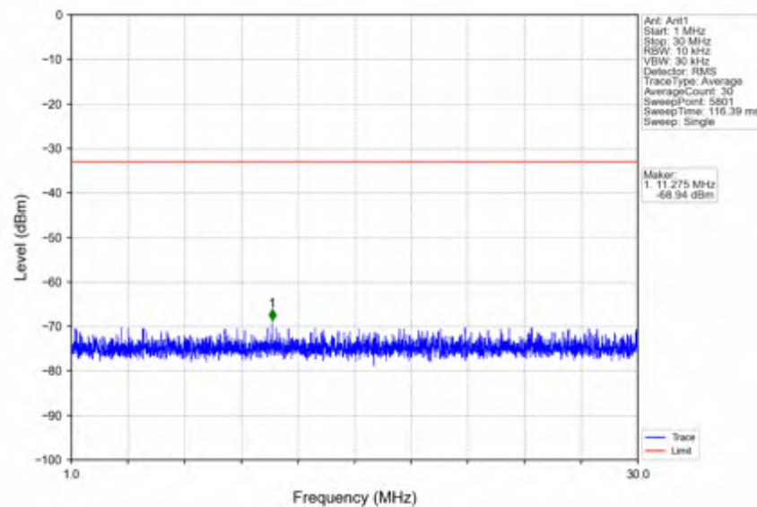
n41_30kHz_SISO_NTNV_100MHz_DFT-s-OFDM QPSK_2640MHz_Edge_1RB_Right
