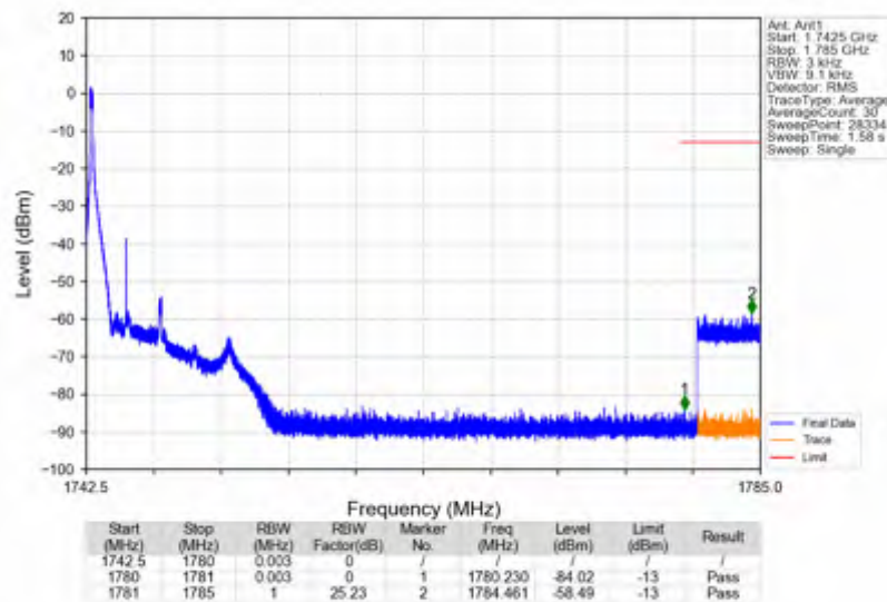
n66_15kHz_SISO_NTNV_5MHz_CP-OFDM QPSK_1745MHz_Edge_1RB_Left
