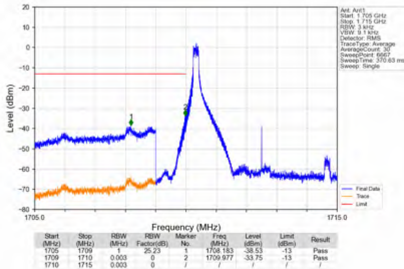
n66_15kHz_SISO_NTNV_5MHz_CP-OFDM_QPSK_1712.5MHz_Edge_1RB_Left
