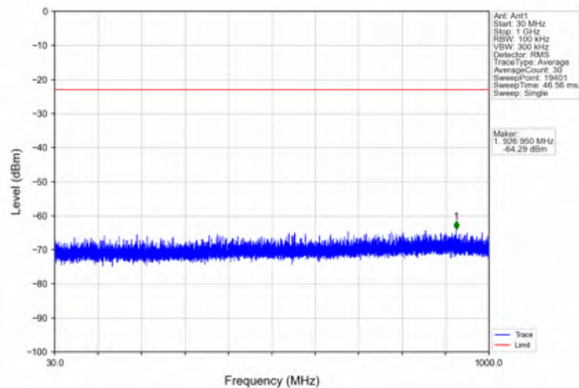
n66_15kHz_SISO_NTNV_15MHz_DFT-s-OFDM_PI/2_BPSK_1745MHz_Edge_1RB_Left
