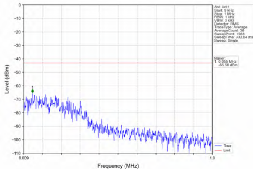
n41_30kHz_SISO_NTNV_100MHz_CP-OFDM QPSK_2592.99MHz_Edge_1RB_Left
