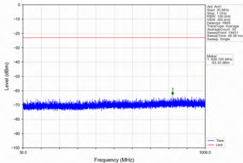
n66_15kHz_SISO_NTNV_10MHz_DFT-s-OFDM QPSK_1775MHz_Edge_1RB_Right
