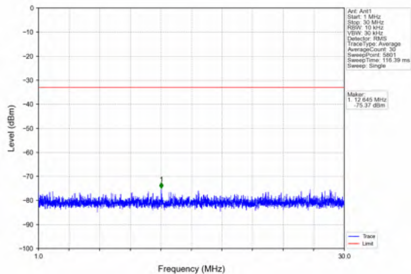
n66_15kHz_SISO_NTNV_5MHz_CP-OFDM QPSK_1777.5MHz_Outer_Full
