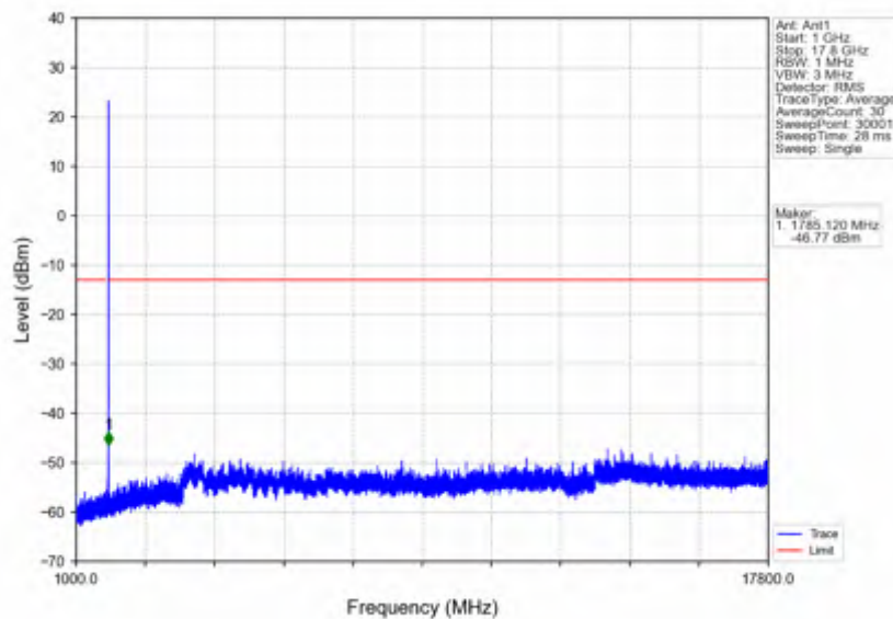
n66_15kHz_SISO_NTNV_5MHz_DFT-s-OFDM QPSK_1712.5MHz_Edge_1RB_Left
