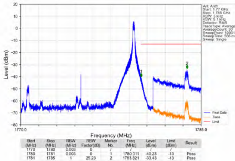
n66_15kHz_SISO_NTNV_10MHz_DFT-s-OFDM QPSK_1775MHz_Inner_1RB_Right
