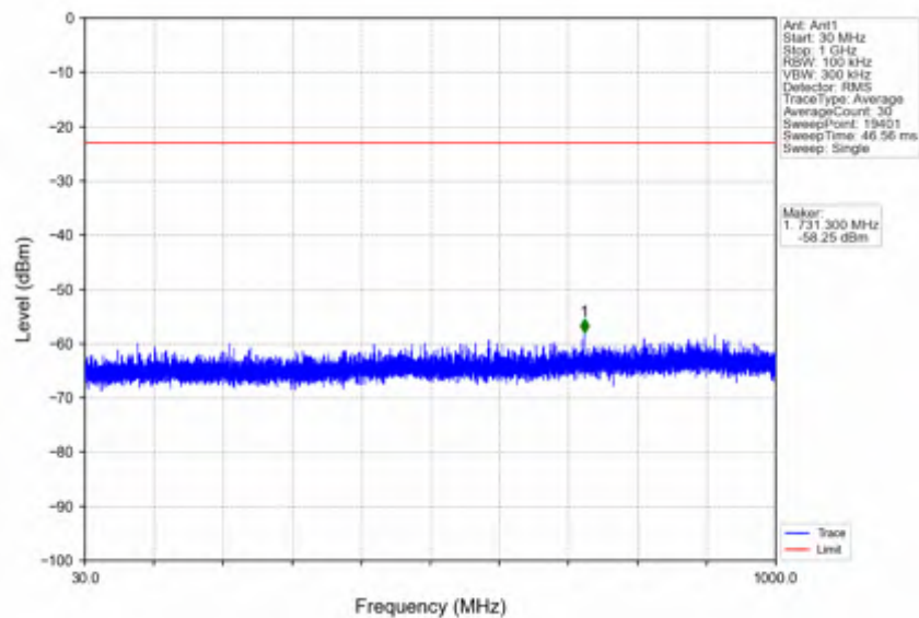
n41_30kHz_SISO_NTNV_100MHz_CP-OFDM_QPSK_2592.99MHz_Edge_1RB_Left
