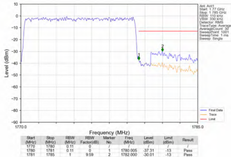
n66_15kHz_SISO_NTNV_10MHz_CP-OFDM QPSK_1775MHz_Outer_Full
