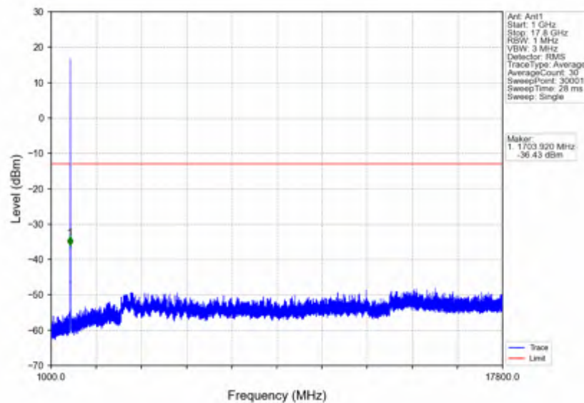
n66_15kHz_SISO_NTNV_5MHz_DFT-s-OFDM QPSK_1712.5MHz_Inner_1RB_Left
