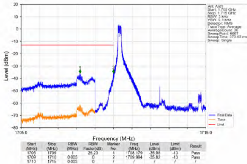
n66_15kHz_SISO_NTNV_5MHz_DFT-s-OFDM QPSK_1712.5MHz_Edge_1RB_Left
