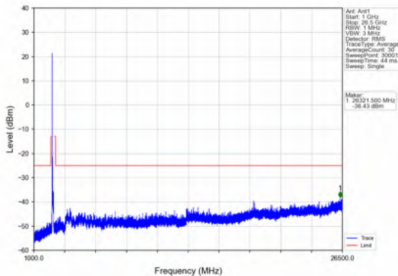
n41_30kHz_SISO_NTNV_100MHz_CP-OFDM QPSK_2546.01MHz_Outer_Full
