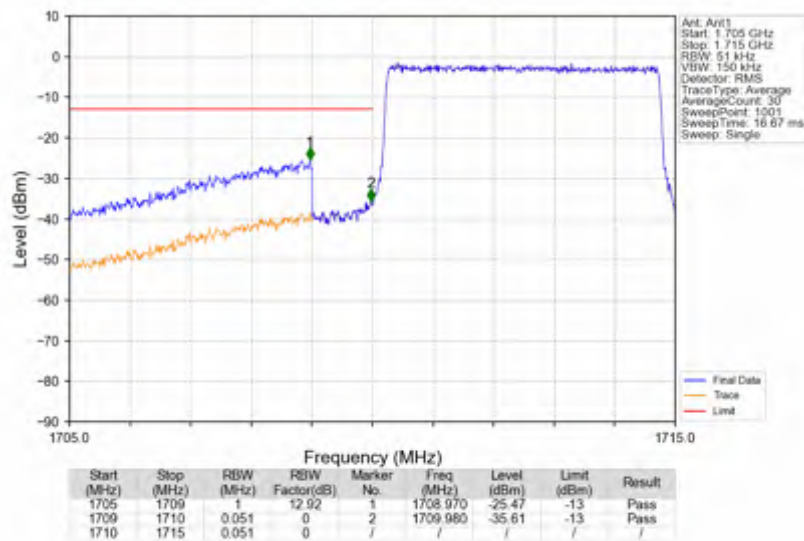
n66_15kHz_SISO_NTNV_5MHz_CP-OFDM QPSK_1712.5MHz_Outer_Full
