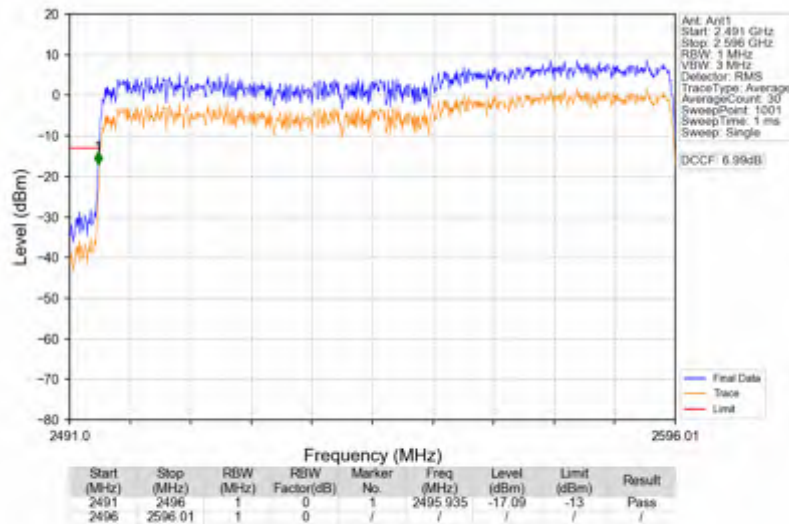
n41_30kHz_SISO_NTNV_100MHz_CP-OFDM QPSK_2546.01MHz_Outer_Full
