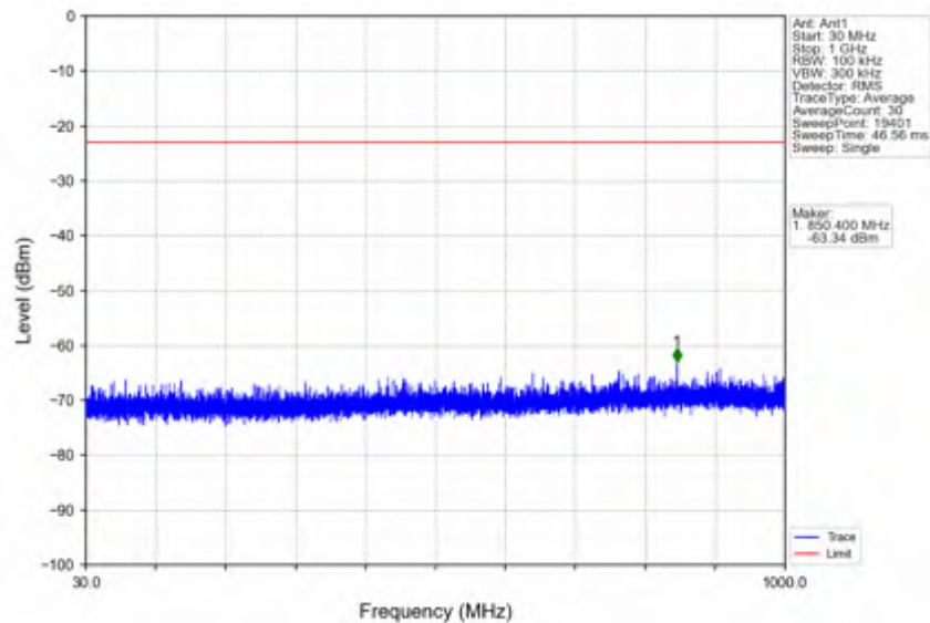
n66_15kHz_SISO_NTNV_5MHz_CP-OFDM QPSK_1712.5MHz_Outer_Full
