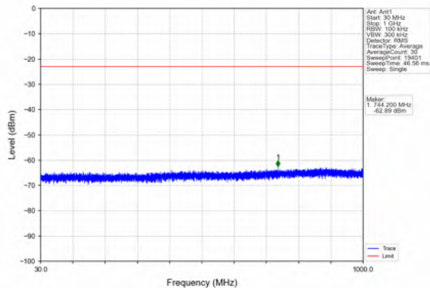
n41 30kHz SISO NTV 90MHz CP-OFDM QPSK 2541MHz Outer Full
