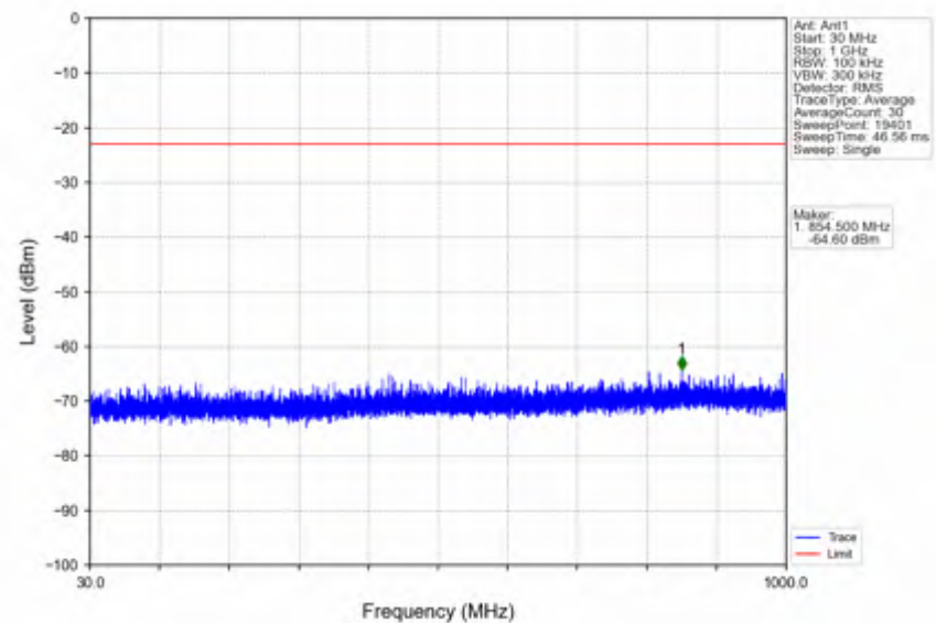
n66_15kHz_SISO_NTNV_10MHz_DFT-s-OFDM QPSK_1715MHz_Outer_Full
