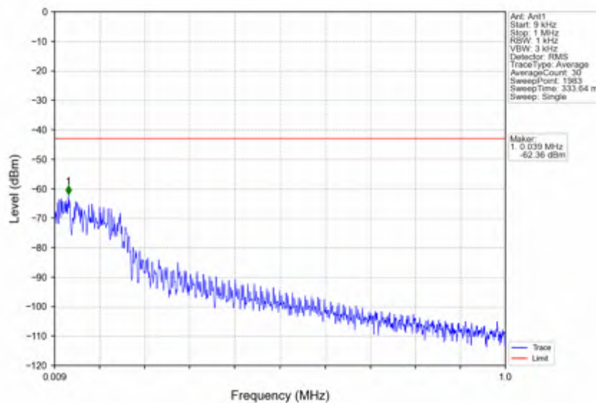
n66_15kHz_SISO_NTNV_5MHz_CP-OFDM_QPSK_1712.5MHz_Edge_1RB_Left
