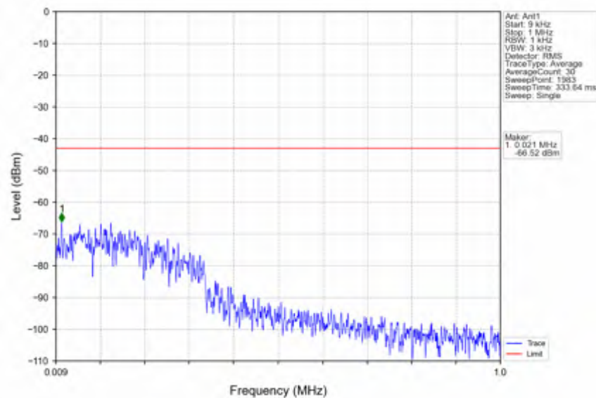
n41_30kHz_SISO_NTNV_90MHz_CP-OFDM QPSK_2592.99MHz_Edge_1RB_Left
