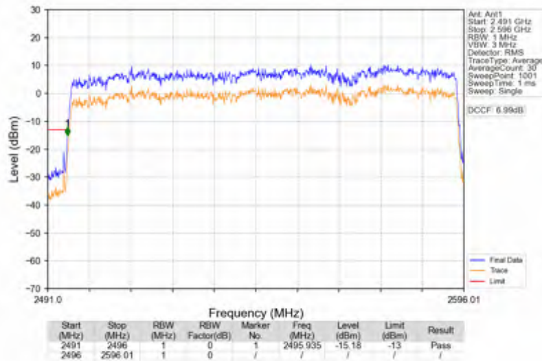
n41_30kHz_SISO_NTNV_100MHz_DFT-s-OFDM_QPSK_2546.01MHz_Outer_Full
