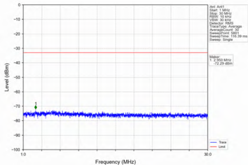
n41_30kHz_SISO_NTNV_100MHz_CP-OFDM QPSK_2546.01MHz_Outer_Full
