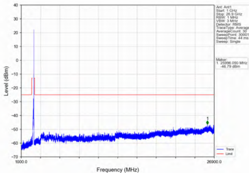
n41_30kHz_SISO_NTNV_100MHz_CP-OFDM QPSK_2640MHz_Outer_Full
