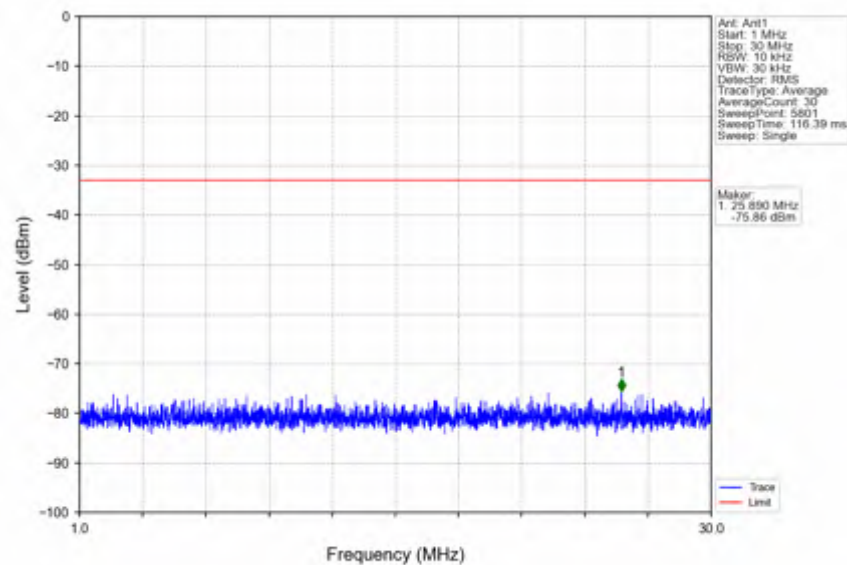
n66_15kHz_SISO_NTNV_10MHz_DFT-s-OFDM QPSK_1775MHz_Inner_1RB_Right
