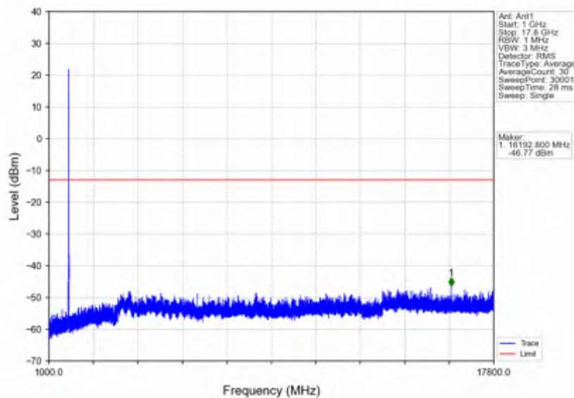
n66_15kHz_SISO_NTNV_10MHz_DFT-s-OFDM QPSK_1775MHz_Edge_1RB_Right
