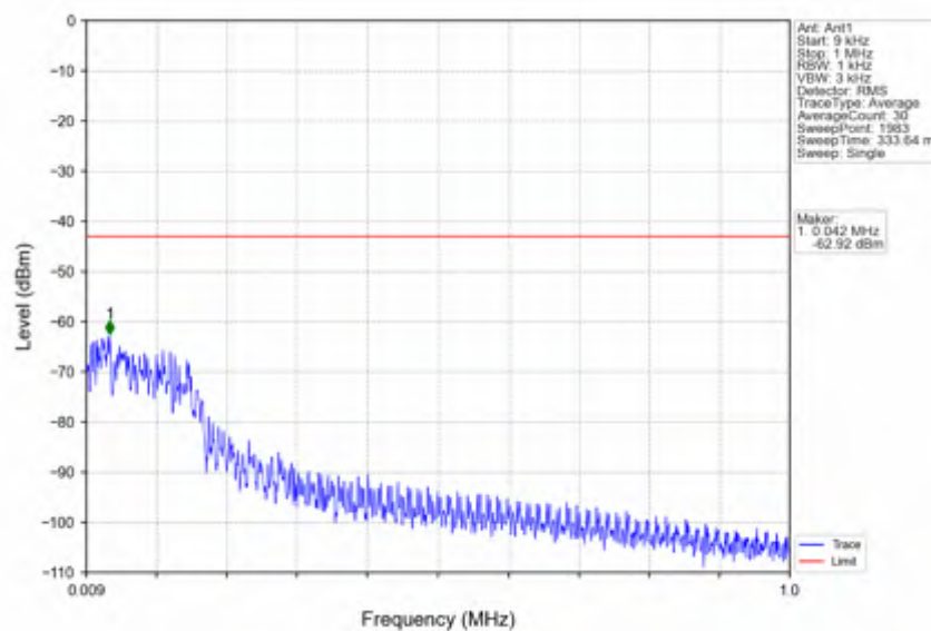
n66_15kHz_SISO_NTNV_10MHz_CP-OFDM QPSK_1775MHz_Edge_1RB_Right
