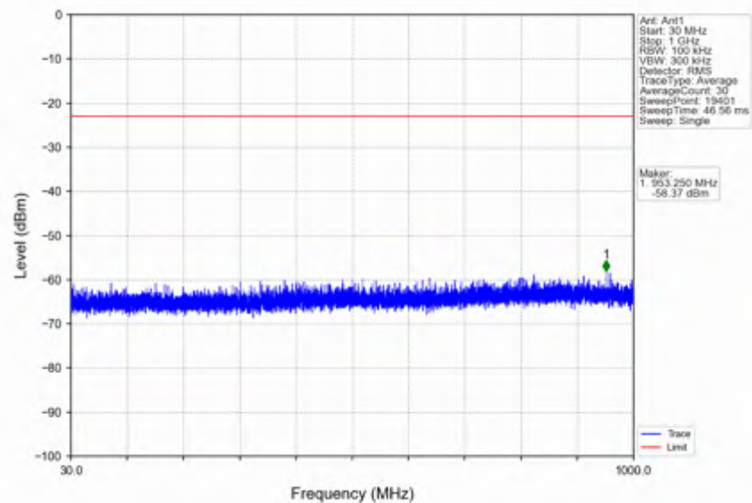
n41_30kHz_SISO_NTNV_100MHz_CP-OFDM QPSK_2640MHz_Edge_1RB_Right
