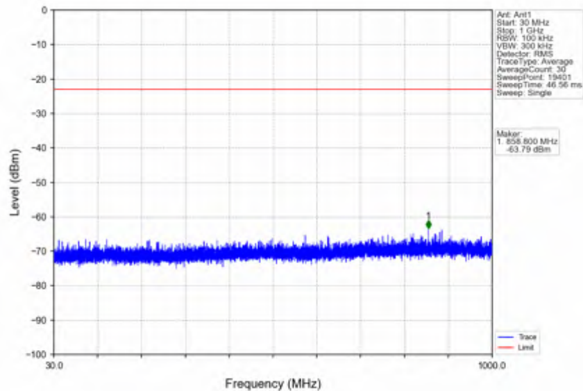
n66_15kHz_SISO_NTNV_10MHz_CP-OFDM QPSK_1775MHz_Outer_Full
