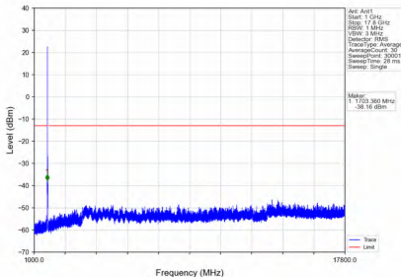
n66_15kHz_SISO_NTNV_15MHz_DFT-s-OFDM PI/2 BPSK_1717.5MHz_Outer_Full
