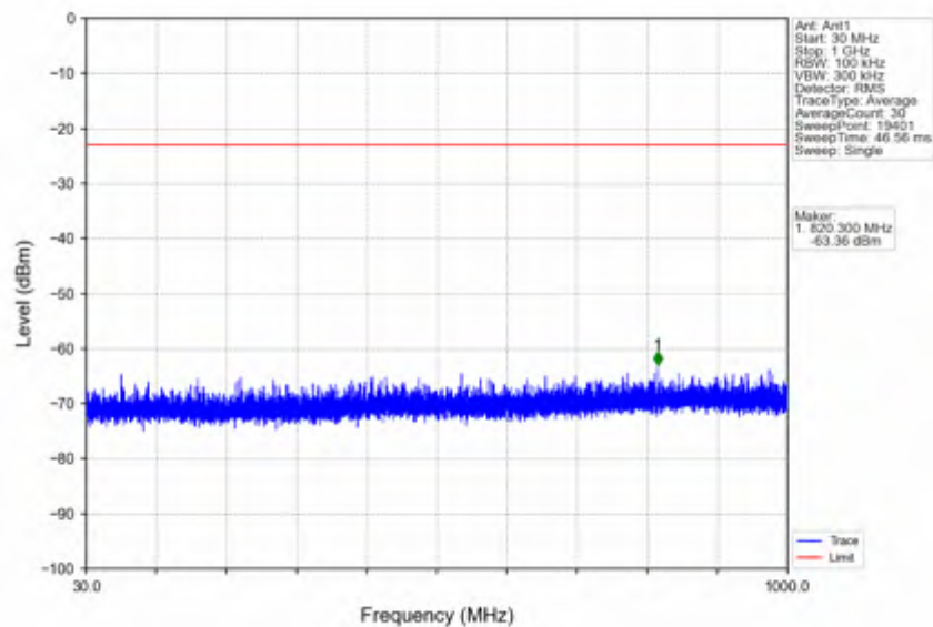
n66_15kHz_SISO_NTNV_5MHz_DFT-s-OFDM_PI/2_BPSK_1745MHz_Edge_1RB_Left
