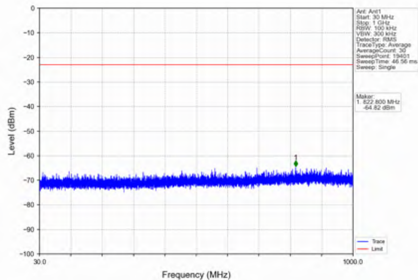
n66_15kHz_SISO_NTNV_5MHz_CP-OFDM QPSK_1777.5MHz_Outer_Full
