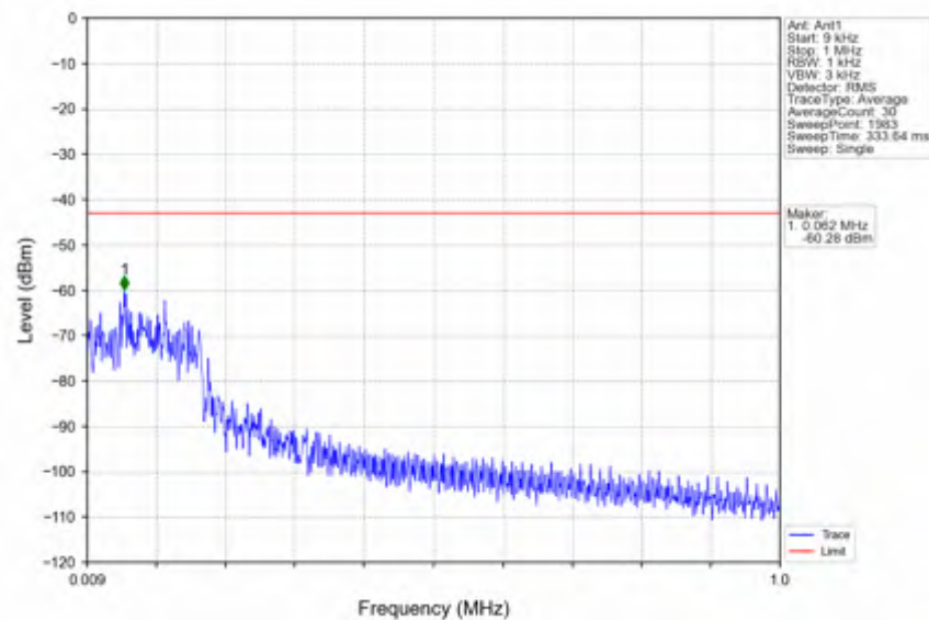
n66_15kHz_SISO_NTNV_10MHz_DFT-s-OFDM QPSK_1775MHz_Edge_1RB_Right
