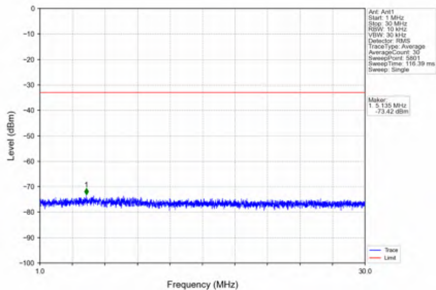
n41_30kHz_SISO_NTNV_100MHz_CP-OFDM QPSK_2640MHz_Outer_Full
