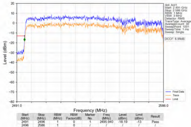
n41_30kHz_SISO_NTNV_90MHz_CP-OFDM QPSK_2541MHz_Outer_Full
