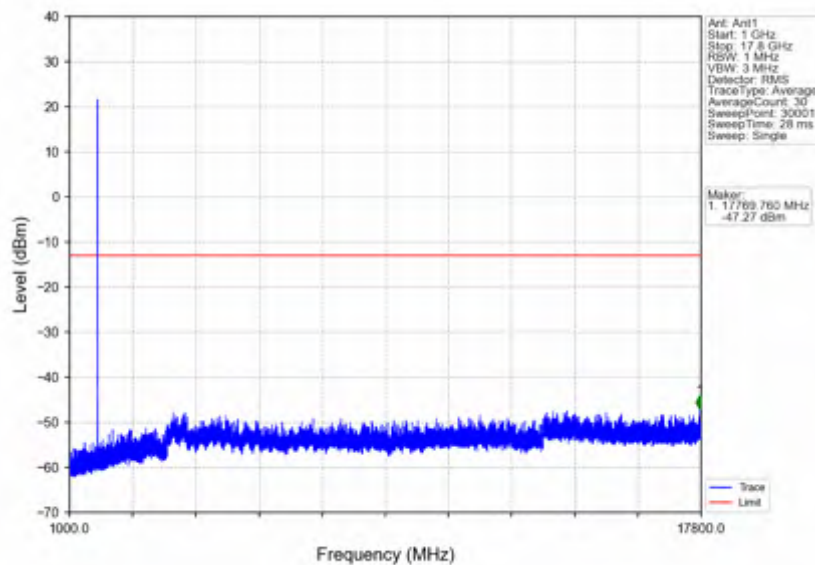
n66_15kHz_SISO_NTNV_5MHz_DFT-s-OFDM QPSK_1777.5MHz_Edge_1RB_Right
