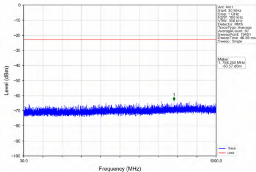
n66_15kHz_SISO_NTNV_10MHz_DFT-s-OFDM PI/2 BPSK_1745MHz_Edge_1RB_Left
