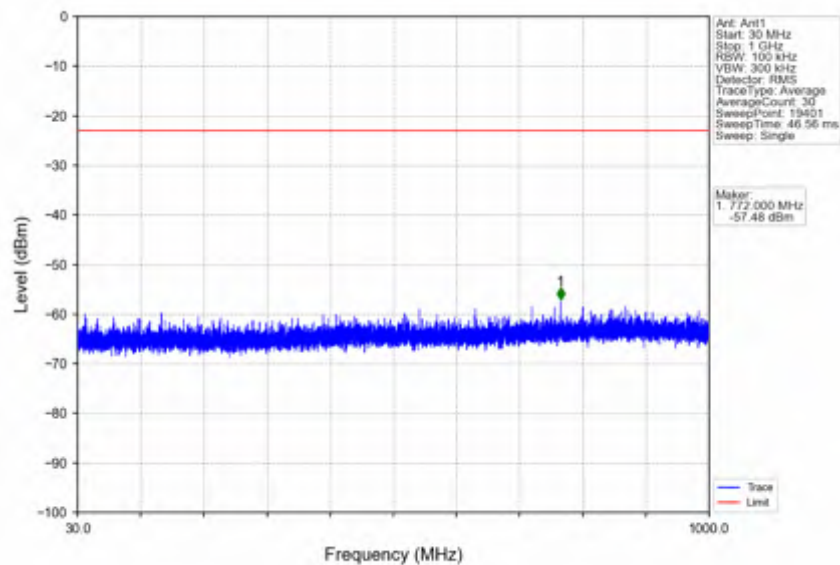
n41_30kHz_SISO_NTNV_100MHz_CP-OFDM QPSK_2546.01MHz_Edge_1RB_Left
