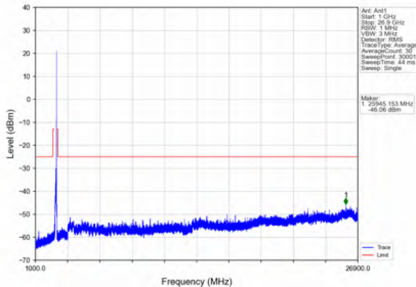
n41_30kHz_SISO_NTNV_100MHz_DFT-s-OFDM QPSK_2640MHz_Edge_1RB_Right
