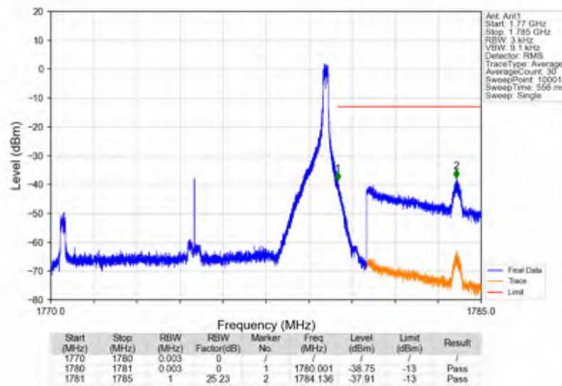
n66_15kHz_SISO_NTNV_10MHz_CP-OFDM QPSK_1775MHz_Edge_1RB_Right
