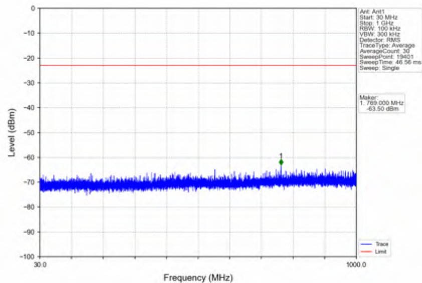
n66_15kHz_SISO_NTNV_5MHz_CP-OFDM QPSK_1777.5MHz_Inner_1RB_Right
