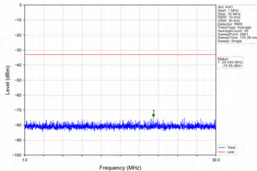
n66_15kHz_SISO_NTNV_10MHz_DFT-s-OFDM QPSK_1775MHz_Outer_Full
