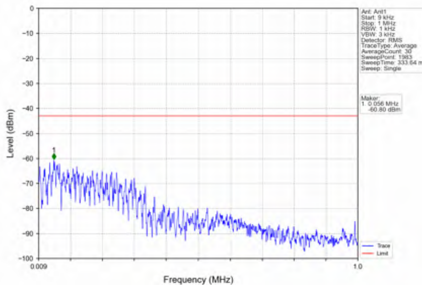
n41_30kHz_SISO_NTNV_90MHz_CP-OFDM QPSK_2644.98MHz_Inner_1RB_Right
