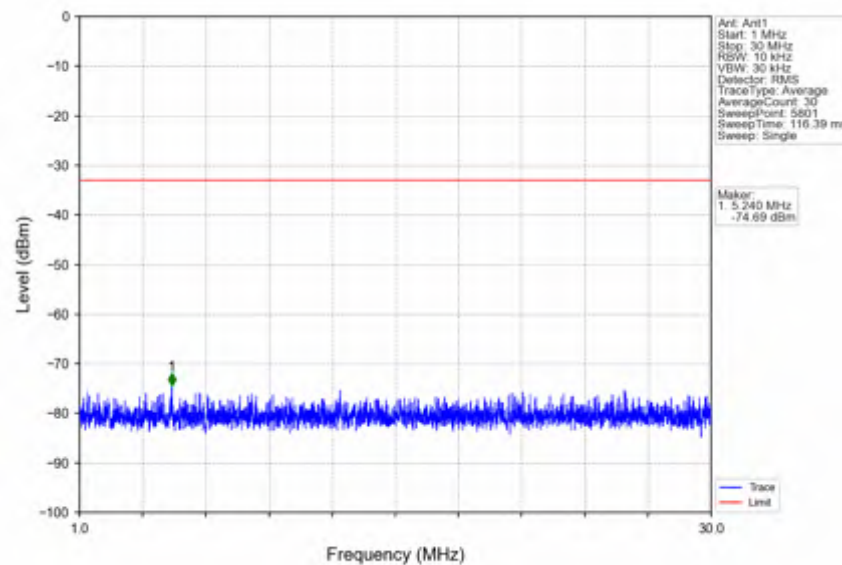
n66_15kHz_SISO_NTNV_15MHz_DFT-s-OFDM PI/2 BPSK_1745MHz_Edge_1RB_Left
