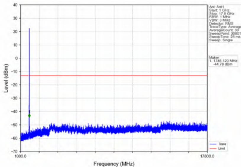
n66_15kHz_SISO_NTNV_10MHz_DFT-s-OFDM PI/2 BPSK_1775MHz_Outer_Full
