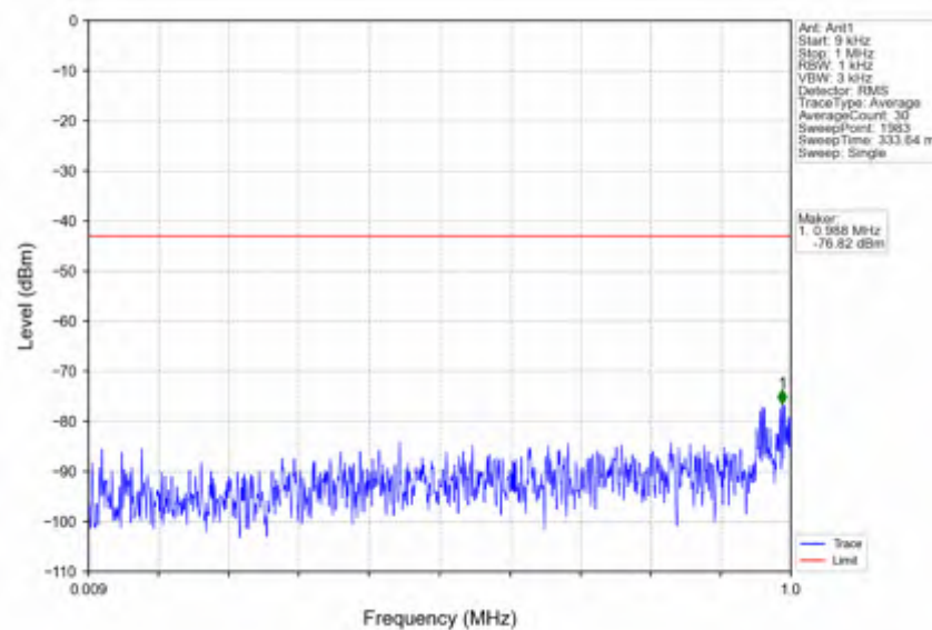
n66_15kHz_SISO_NTNV_10MHz_DFT-s-OFDM QPSK_1775MHz_Outer_Full
