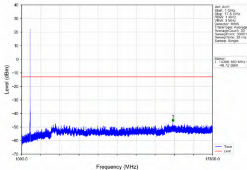
n66_15kHz_SISO_NTNV_15MHz_DFT-s-OFDM_PI/2_BPSK_1745MHz_Edge_1RB_Left
