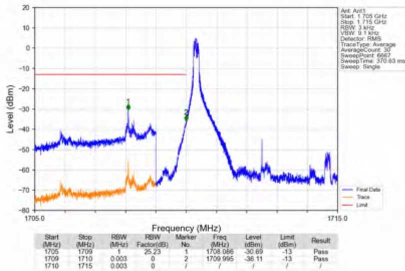
n66_15kHz_SISO_NTNV_5MHz_DFT-s-OFDM_PI/2_BPSK_1712.5MHz_Edge_1RB_Left
