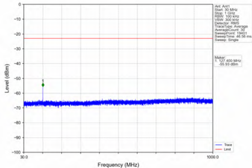
n41_30kHz_SISO_NTNV_100MHz_DFT-s-OFDM_QPSK_2640MHz_Inner_1RB_Right
