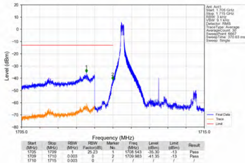
n66_15kHz_SISO_NTNV_5MHz_DFT-s-OFDM QPSK_1712.5MHz_Inner_1RB_Left
