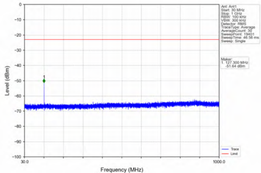
n41_30kHz_SISO_NTNV_100MHz_CP-OFDM QPSK_2640MHz_Inner_1RB_Right
