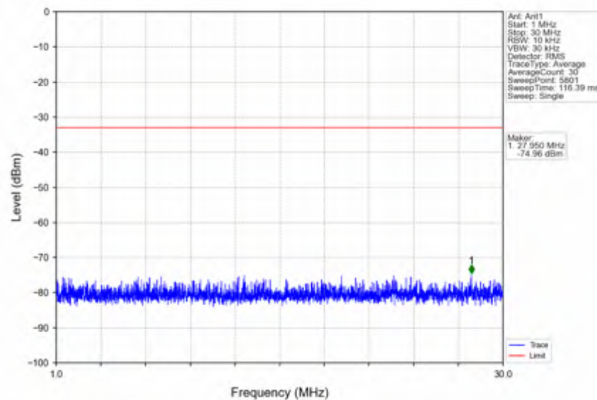
n66_15kHz_SISO_NTNV_5MHz_CP-OFDM QPSK_1745MHz_Edge_1RB_Left
