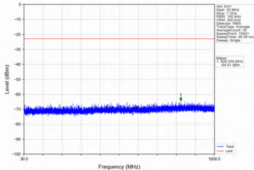
n66_15kHz_SISO_NTNV_10MHz_DFT-s-OFDM_PI/2_BPSK_1715MHz_Outer_Full
