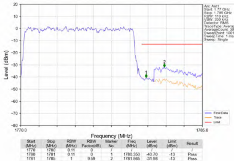
n66_15kHz_SISO_NTNV_10MHz_DFT-s-OFDM QPSK_1775MHz_Outer_Full
