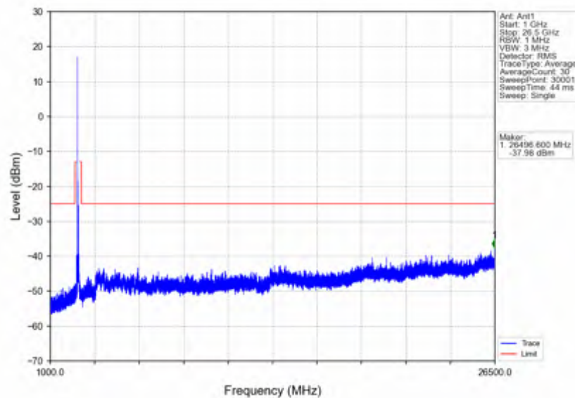
n41_30kHz_SISO_NTNV_90MHz_CP-OFDM QPSK_2592.99MHz_Edge_1RB_Left
