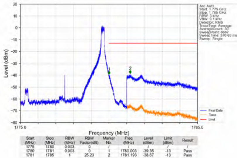
n66_15kHz_SISO_NTNV_5MHz_CP-OFDM_QPSK_1777.5MHz_Edge_1RB_Right
