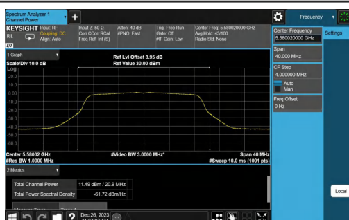
11N20MIMO-Ant0-5580-TPC_L-PASS
