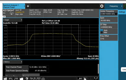
11N20MIMO-Ant1-5580-TPC_L-PASS
