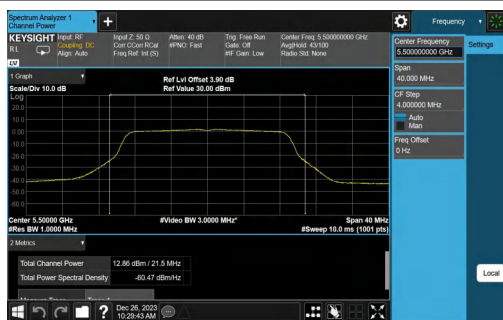
11N20SISO-Ant0-5500-TPC_L-PASS
