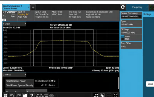
11N20MIMO-Ant0-5700-TPC_L-PASS
