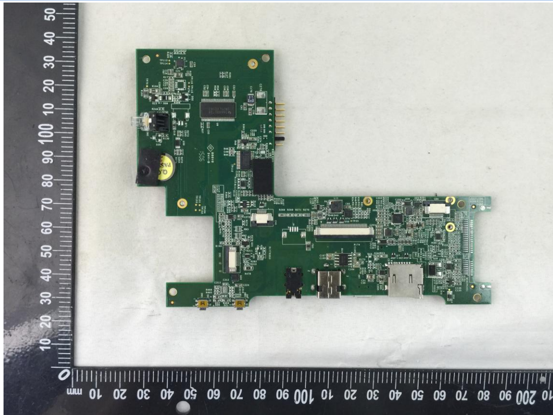
MAIN BOARD 5 BACK VIEW
