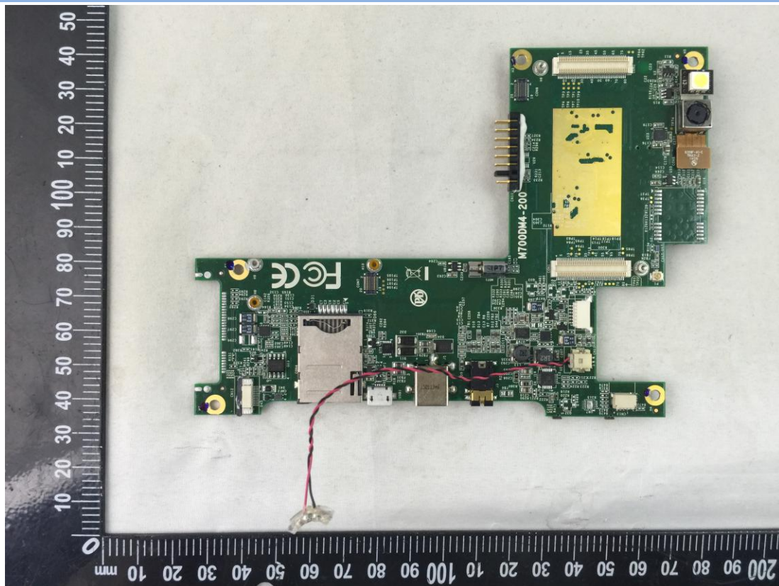
MAIN BOARD 5 FRONT VIEW
