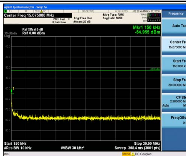
Band5_10MHz_16QAM_20600_1RB#0
