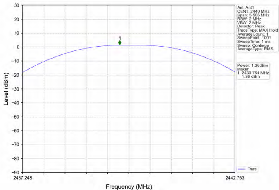
8-DPSK_MCH_2440MHz_Ant1_NTNV
