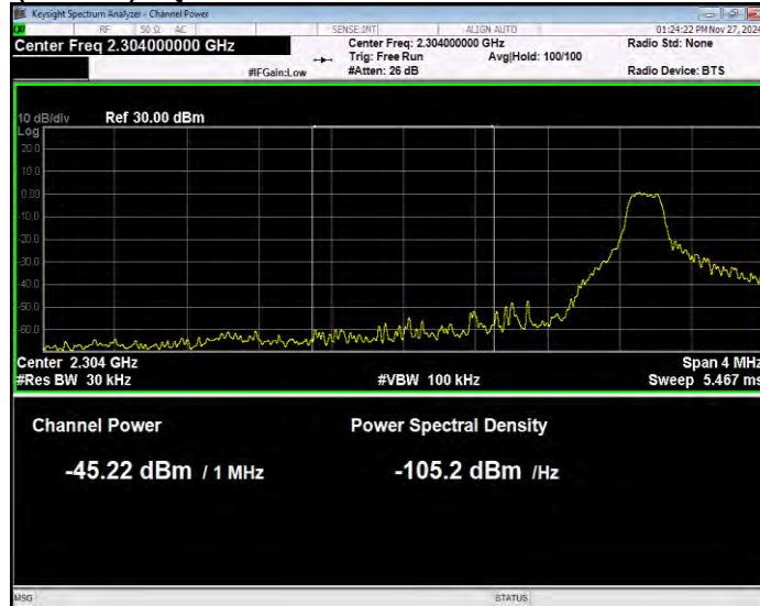
Band40(2305-2315) 16QAM BW=5MHz Channel=38725 RB Size=1 Position=#0 Normal
