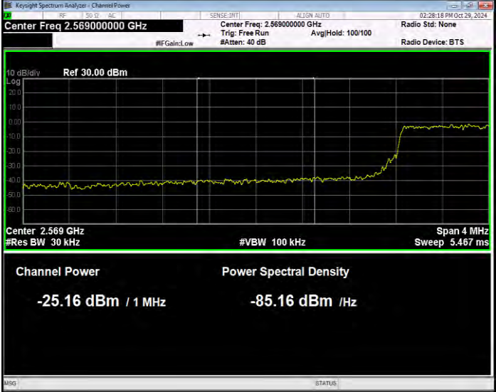
Band38 QPSK BW=5MHz Channel=37775 RB Size=25 Position=#0 Normal
