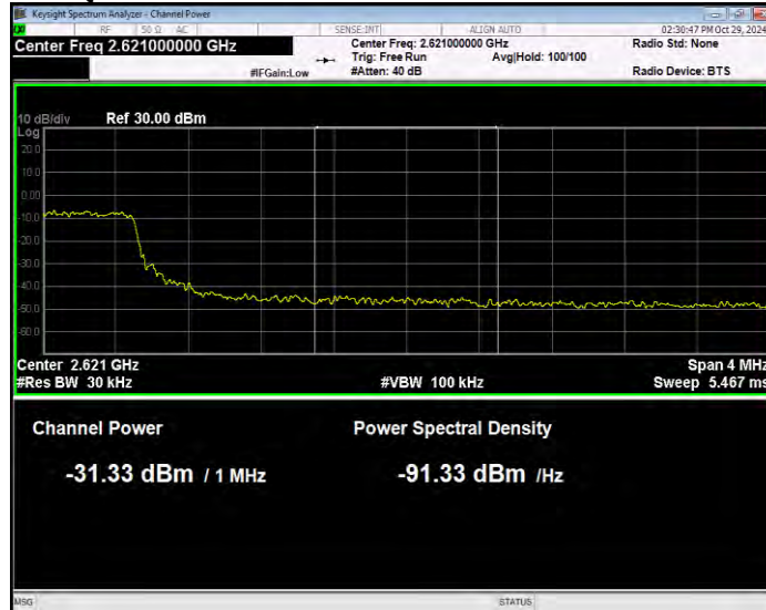
Band38 QPSK BW=10MHz Channel=38200 RB Size=50 Position=#0 Normal
