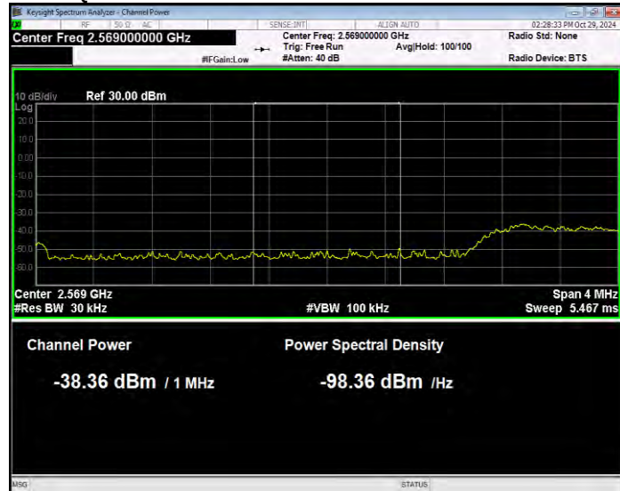
Band38 16QAM BW=5MHz Channel=37775 RB Size=1 Position=#Max Normal
