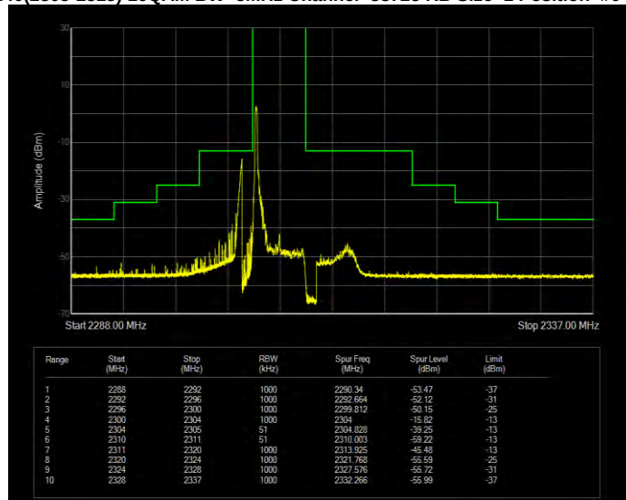
Band40(2305-2315) 16QAM BW=5MHz Channel=38725 RB Size=25 Position=#0 Extended
