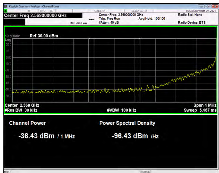
Band38 QPSK BW=20MHz Channel=37850 RB Size=1 Position=#0 Normal
