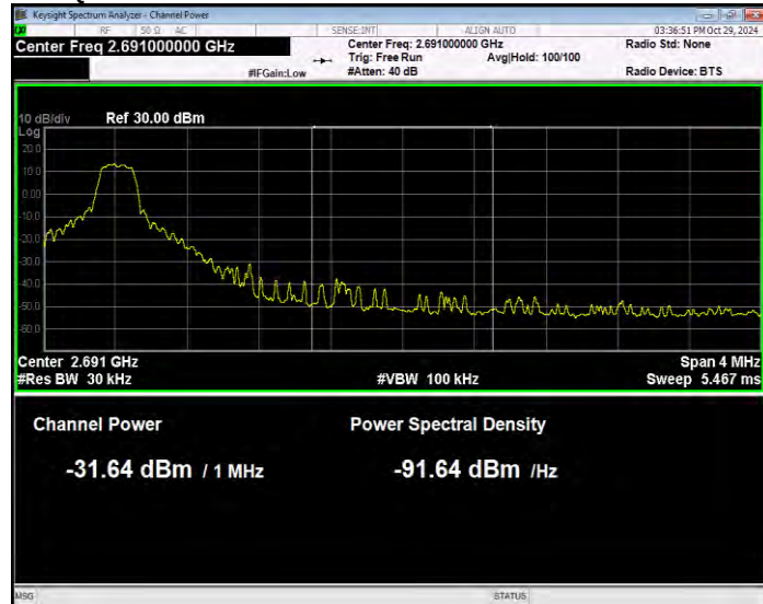
Band41 QPSK BW=10MHz Channel=41540 RB Size=1 Position=#Max Normal
