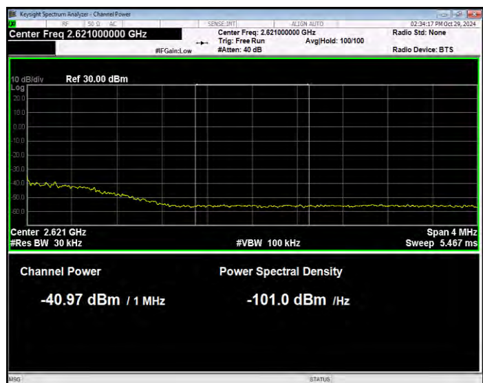
Band38 16QAM BW=20MHz Channel=38150 RB Size=1 Position=#0 Normal
