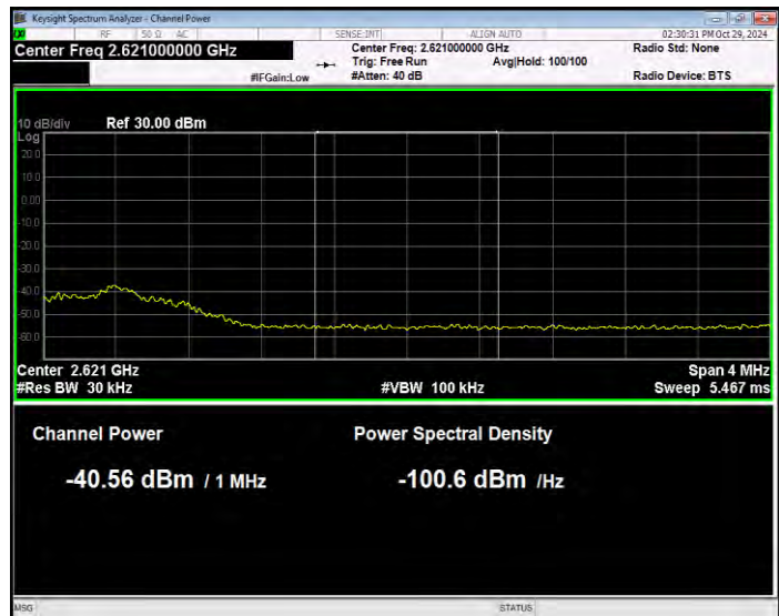
Band38 QPSK BW=10MHz Channel=38200 RB Size=1 Position=#0 Normal
