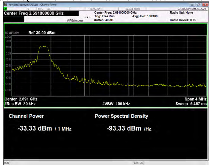
Band41 16QAM BW=5MHz Channel=41565 RB Size=1 Position=#Max Normal
