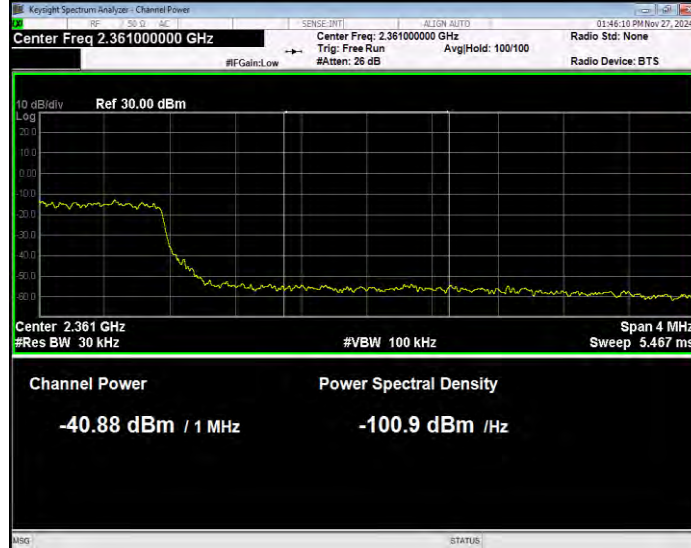
Band40(2350-2360) 16QAM BW=5MHz Channel=39225 RB Size=25 Position=#0 Normal
