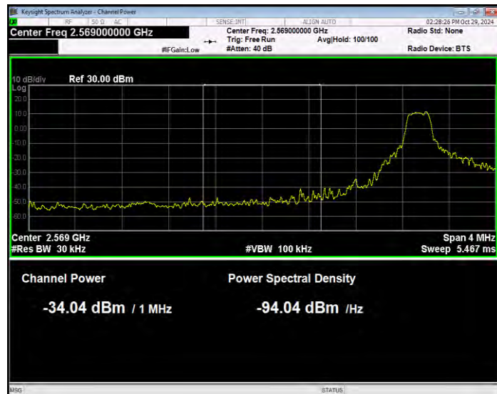
Band38 16QAM BW=5MHz Channel=37775 RB Size=1 Position=#0 Normal
