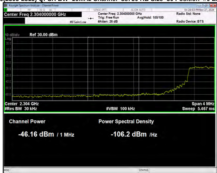
Band40(2305-2315) QPSK BW=10MHz Channel=38750 RB Size=50 Position=#0 Normal
