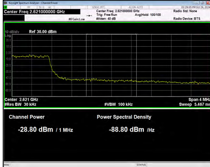
Band38 QPSK BW=5MHz Channel=38225 RB Size=25 Position=#0 Normal
