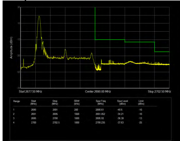
Band41 QPSK BW=10MHz Channel=41540 RB Size=1 Position=#Max Extended
