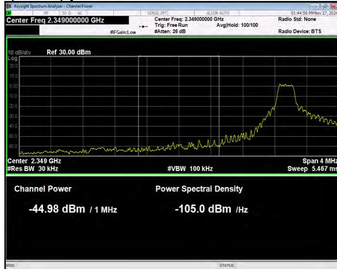
Band40(2350-2360) QPSK BW=5MHz Channel=39175 RB Size=1 Position=#0 Normal
