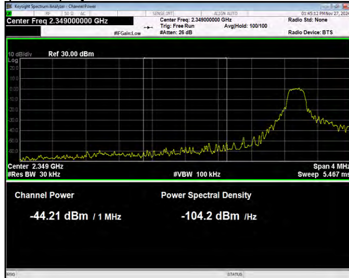
Band40(2350-2360) 16QAM BW=5MHz Channel=39175 RB Size=1 Position=#0 Normal
