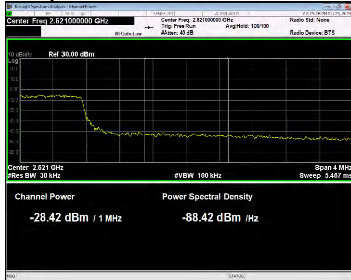
Band38 16QAM BW=5MHz Channel=38225 RB Size=25 Position=#0 Normal
