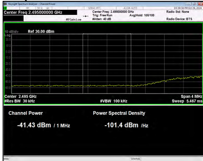
Band41 16QAM BW=20MHz Channel=39750 RB Size=1 Position=#Max Normal
