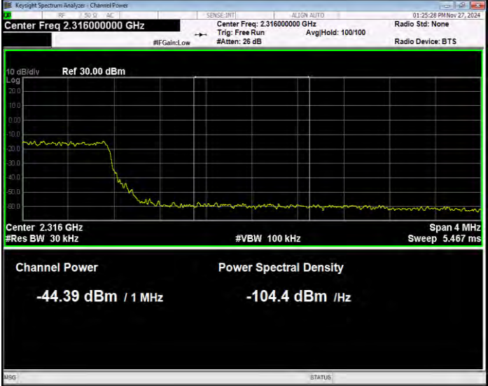
Band40(2305-2315) 16QAM BW=5MHz Channel=38775 RB Size=25 Position=#0 Normal
