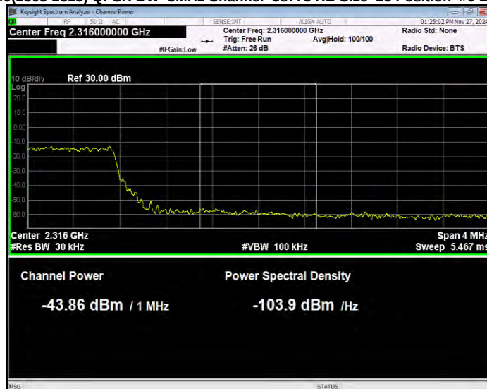
Band40(2305-2315) QPSK BW=5MHz Channel=38775 RB Size=25 Position=#0 Normal
