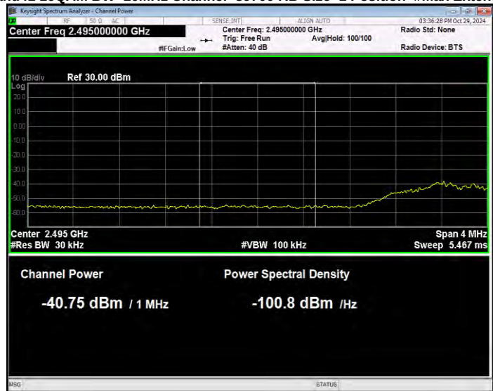
Band41 16QAM BW=10MHz Channel=39700 RB Size=1 Position=#Max Normal
