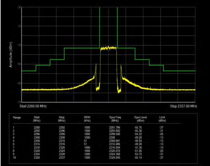
Band40(2305-2315) QPSK BW=10MHz Channel=38750 RB Size=1 Position=#0 Extended
