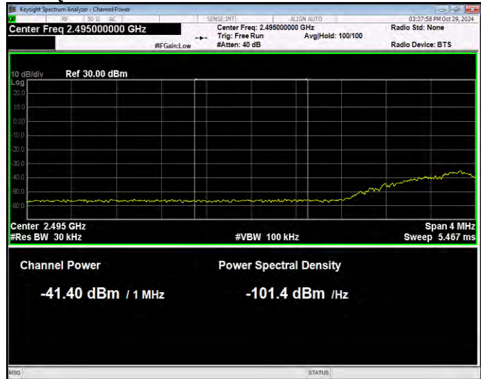
Band41 16QAM BW=15MHz Channel=39725 RB Size=1 Position=#Max Normal
