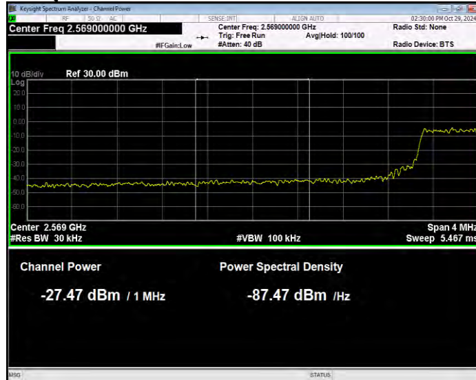
Band38 QPSK BW=10MHz Channel=37800 RB Size=50 Position=#0 Normal
