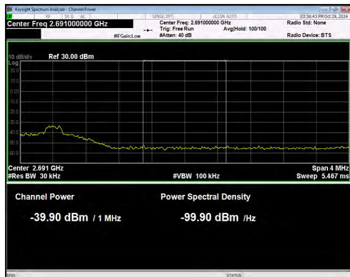
Band41 QPSK BW=10MHz Channel=41540 RB Size=1 Position=#0 Normal
