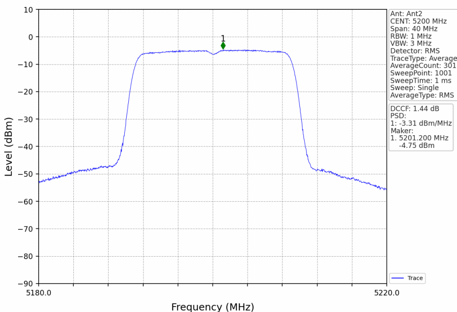
802.11ac(VHT20)_MCH_5200MHz_MIMO_NTNV
