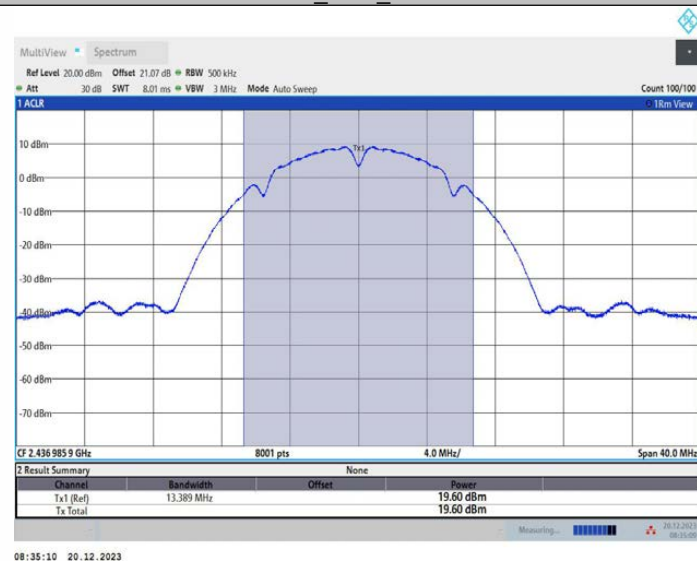
11B_Ant3_2437
