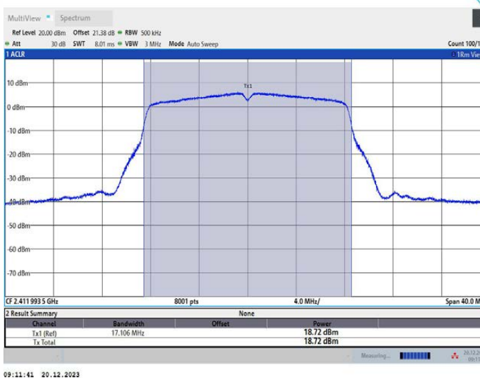
11G_Ant4_2412
