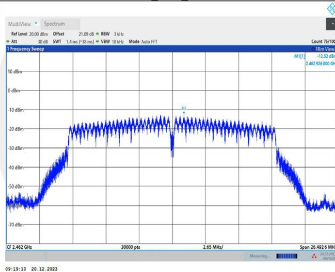
11G_Ant4_2462
