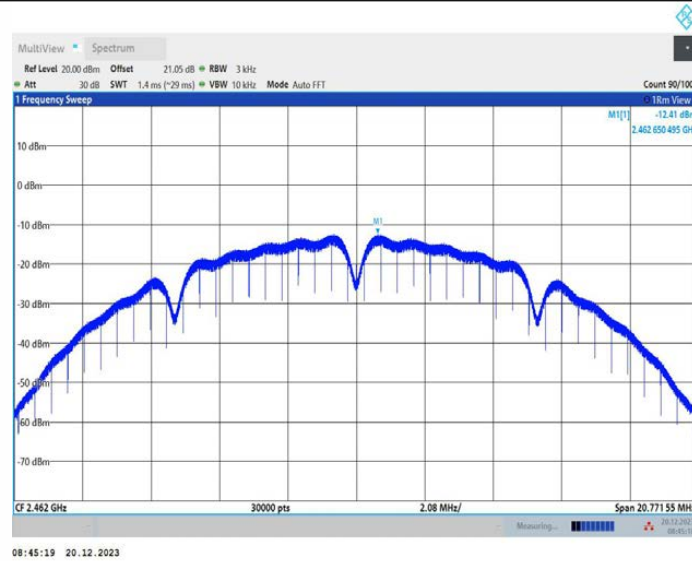
11B_Ant3_2462
