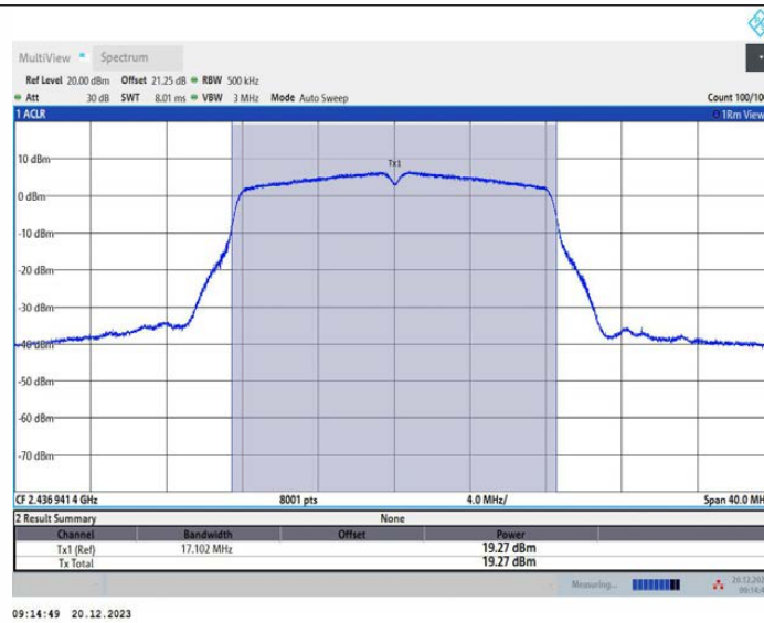
11G_Ant4_2437
