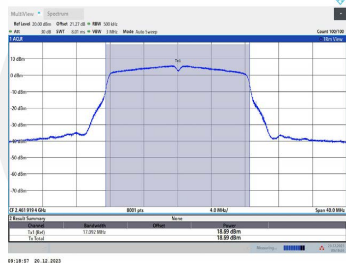
11G_Ant4_2462
