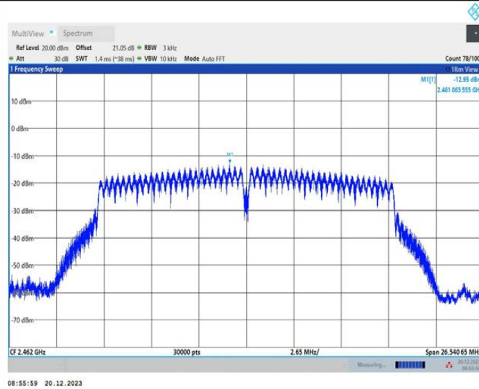
11G_Ant3_2462
