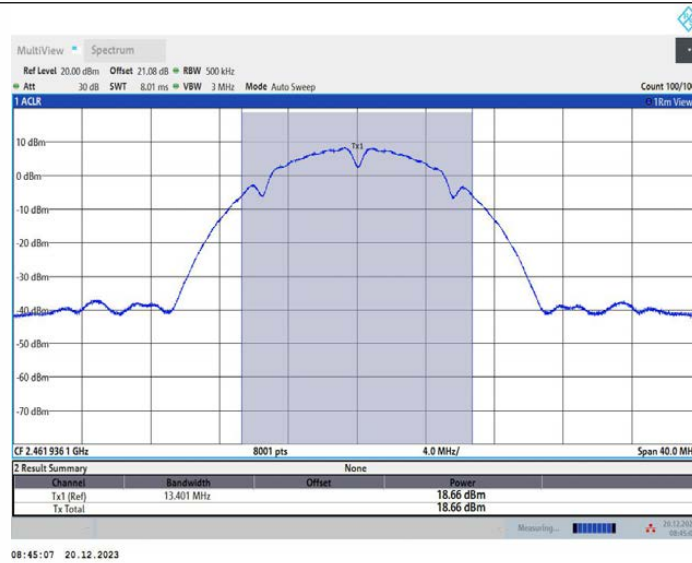
11B_Ant3_2462
