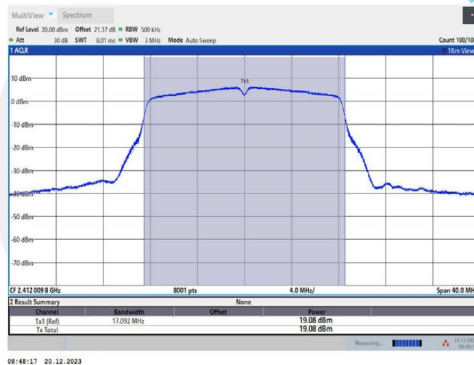
11G_Ant3_2412
