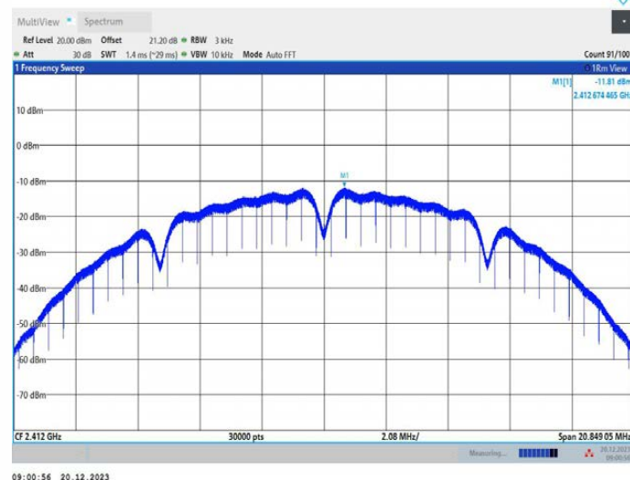
11B_Ant3_2412
