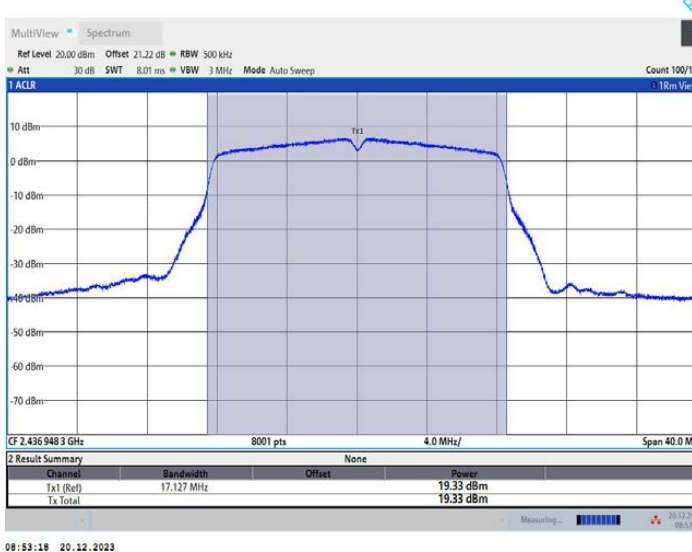
11G_Ant3_2437
