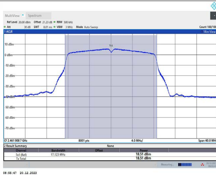
11G_Ant3_2462
