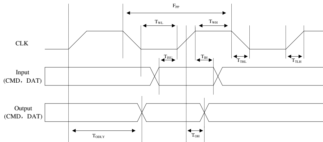
Figure8: SDIO Timing
