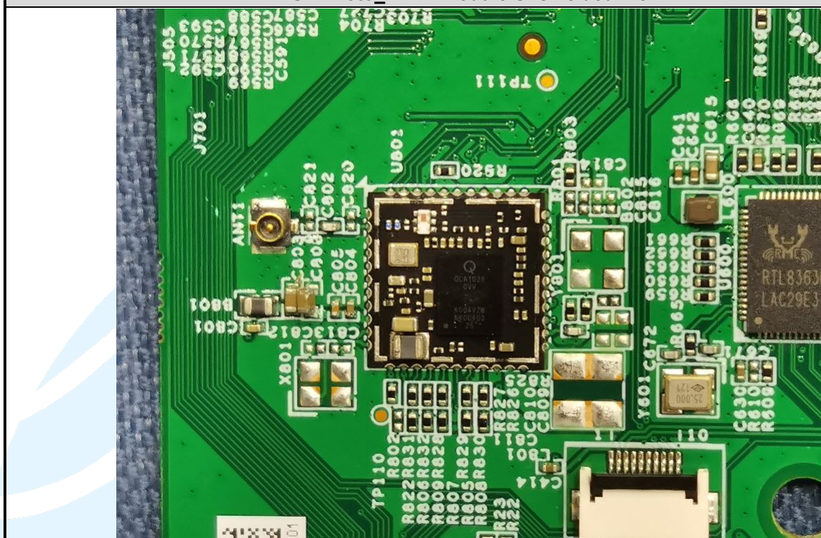
EUT Photo_ Wi-Fi Module Unshielded View
